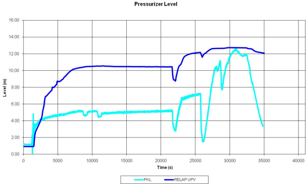
Figure 9: Pressurizer Level
