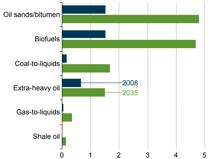
Figure 30. Unconventional liquids production by fuel type, 2008 and 2035 (million barrels per day)
