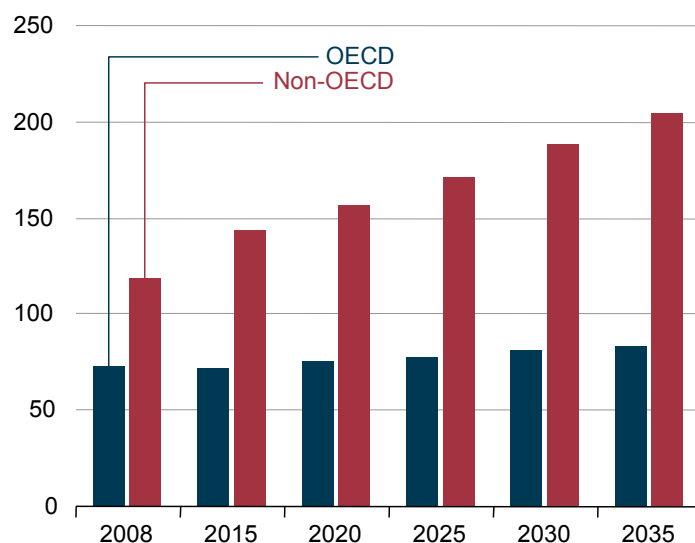
Figure 22. World delivered industrial energy consumption, 2008-2035 (quadrillion Btu)
