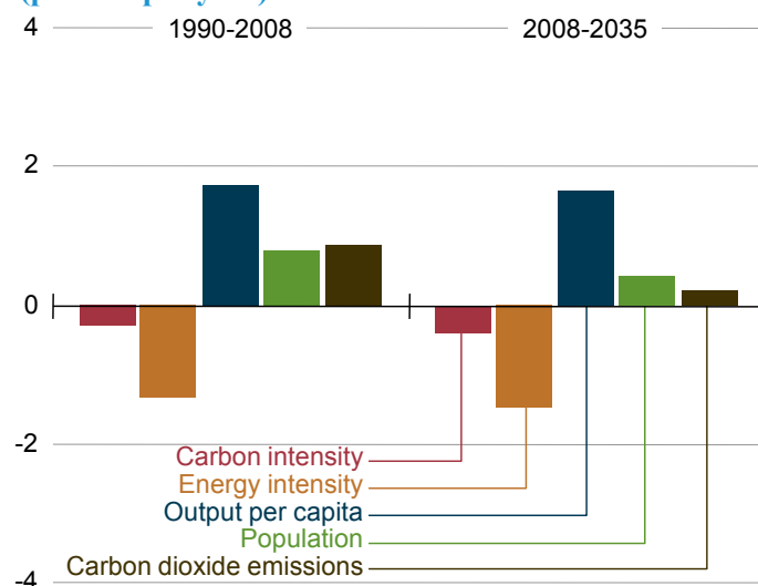
Figure 118. Average annual changes in Kaya decomposition components of OECD carbon dioxide emissions growth, 1990-2008 and 2008-2035 (percent per year)
