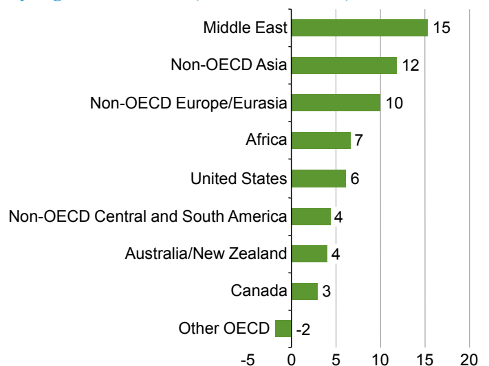
Figure 41. Change in world natural gas production by region, 2008-2035 (trillion cubic feet)
