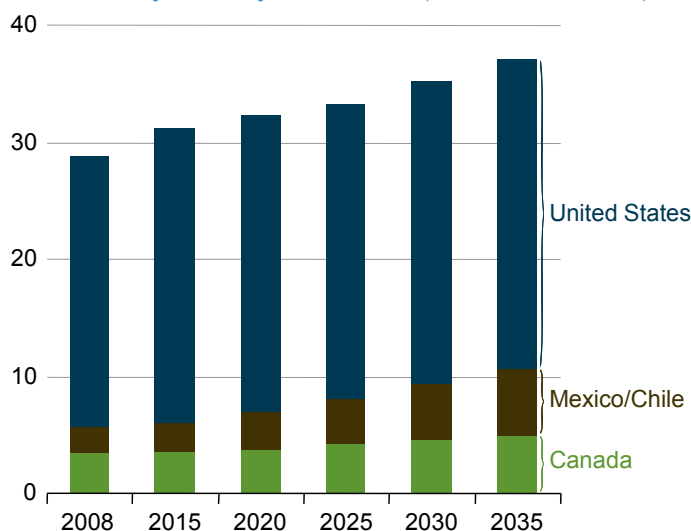
Figure 43. Natural gas consumption in OECD Americas by country, 2008-2035 (trillion cubic feet)
