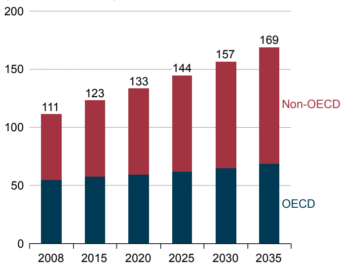
Figure 40. World natural gas consumption, 2008-2035 (trillion cubic feet)
