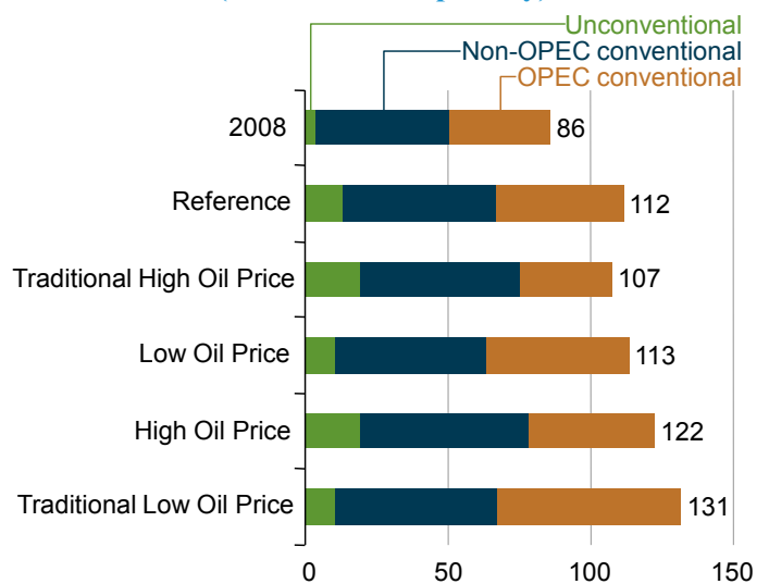
Figure 32. World liquid fuels production in five cases, 2008 and 2035 (million barrels per day)
