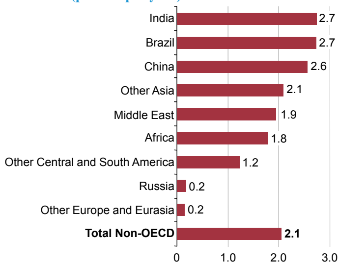
Figure 114. Average annual growth of energy-related carbon dioxide emissions in non-OECD economies, 2008-2035 (percent per year)
