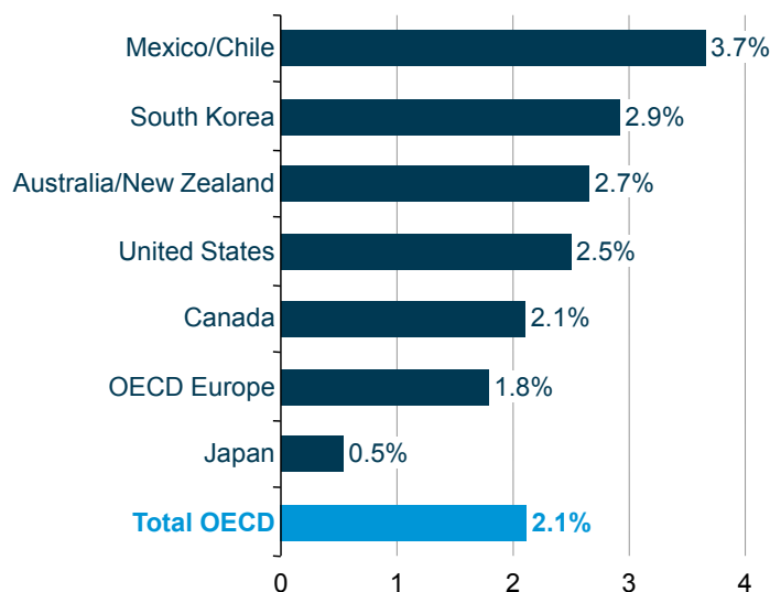
Figure 25. OECD gross domestic product growth rates by country grouping, 2008-2035 (average annual percent change)
