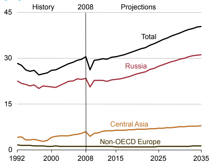
Figure 51. Non-OECD Europe and Eurasia natural gas production, 1992-2035 (trillion cubic feet)
