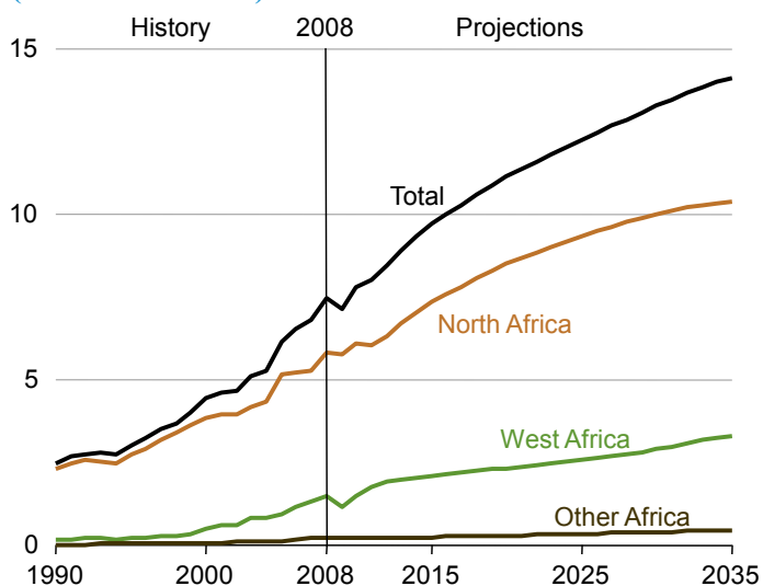
Figure 52. Africa natural gas production, 1990-2035 (trillion cubic feet)
