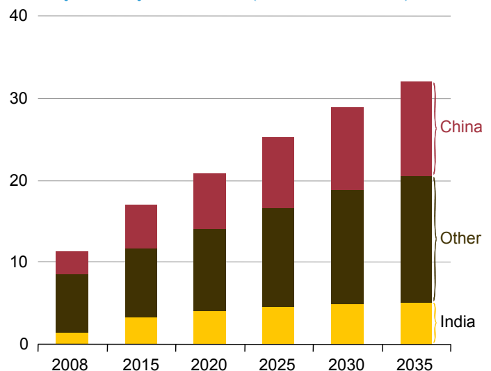
Figure 47. Natural gas consumption in non-OECD Asia by country, 2008-2035 (trillion cubic feet)
