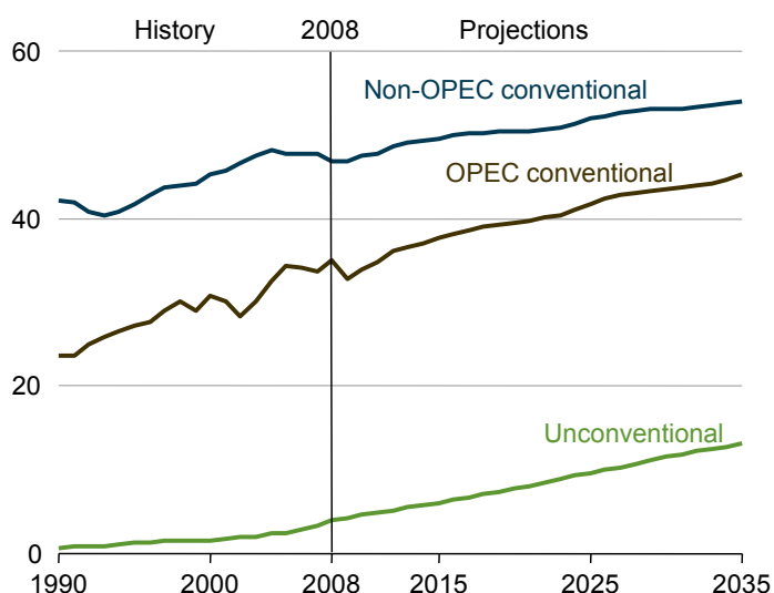
Figure 28. World liquid fuels production, 1990-2035 (quadrillion Btu)
