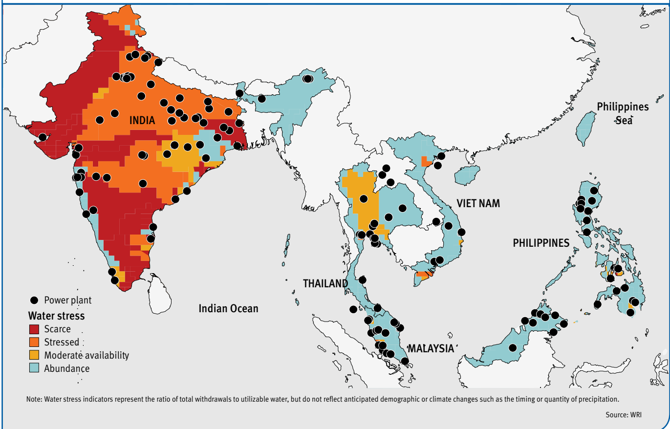
Figure 4.18 Thermal power and hydropower plant locations and water stress levels in five countries of South and South East Asia
