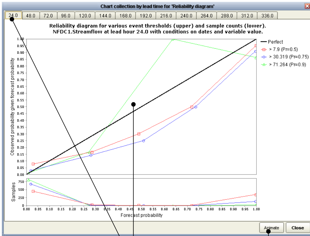
Fig. 13: plot collection for a metric with one plot for each lead time
