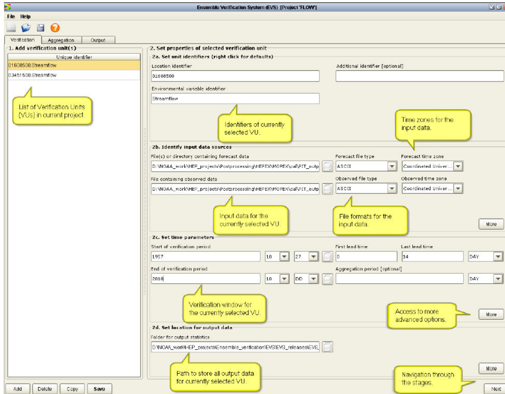
Fig. 1: The opening panel in the “Verification” stage
