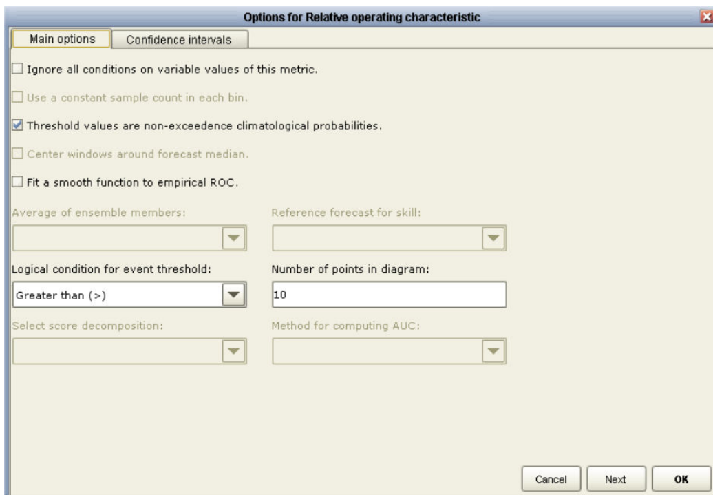
Fig. 10a: Advanced parameter options for a selected metric (ROC in this case)
