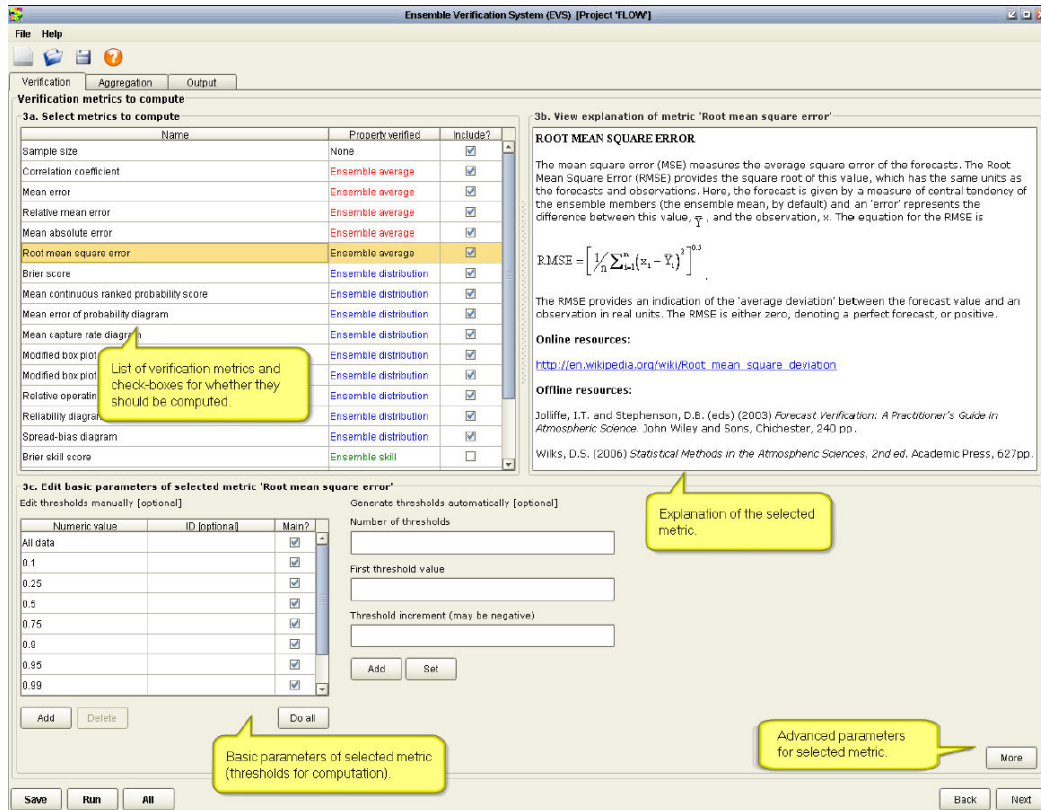
Fig. 2: The second panel in the “Verification” stage
