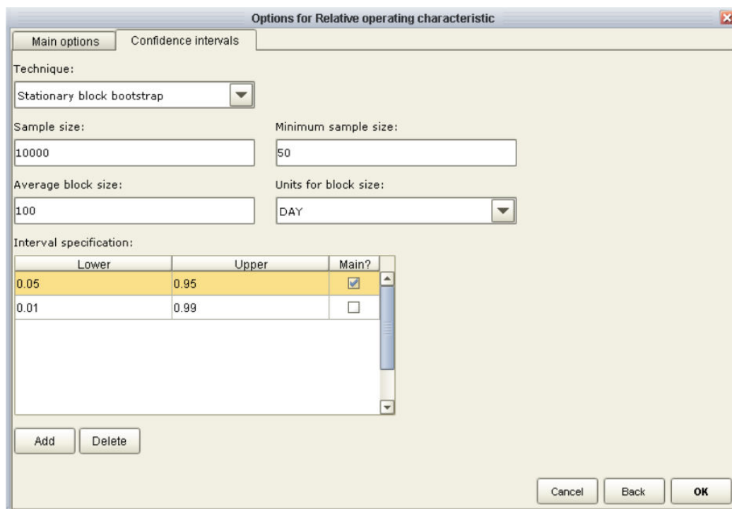
Fig. 10b: Confidence intervals for a selected metric (ROC in this case)
