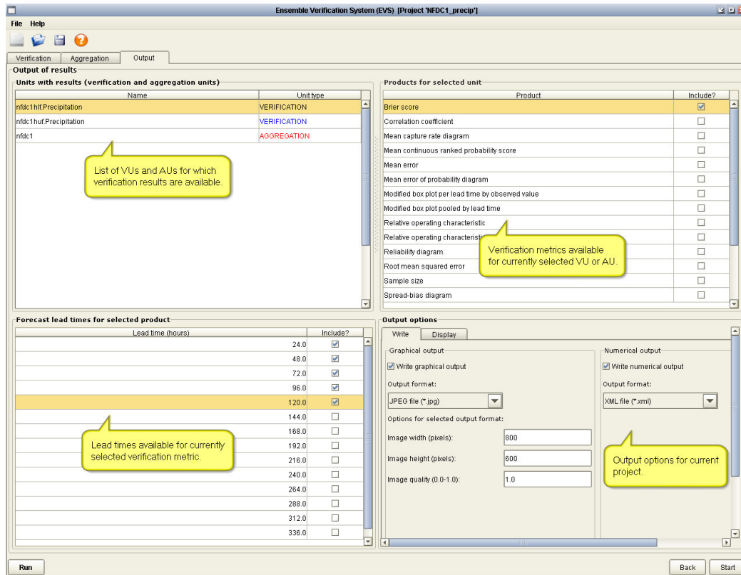
Fig. 4: The only panel in the “Output” stage
