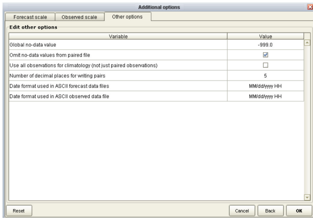
Fig. 8b: Other options (Additional options), accessed from the input data dialog
