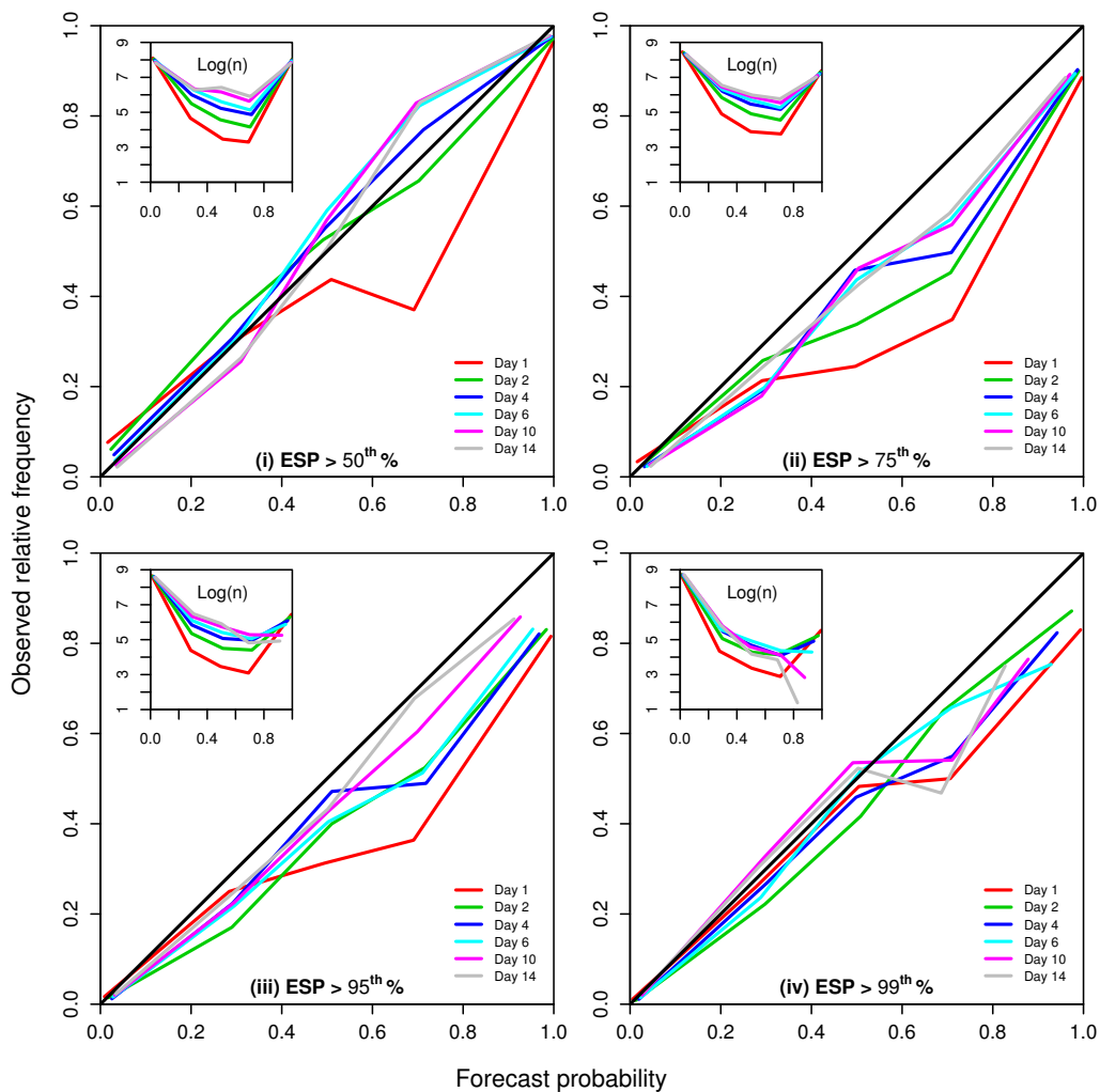
Fig. 19: Reliability diagrams for the ESP forecasts
