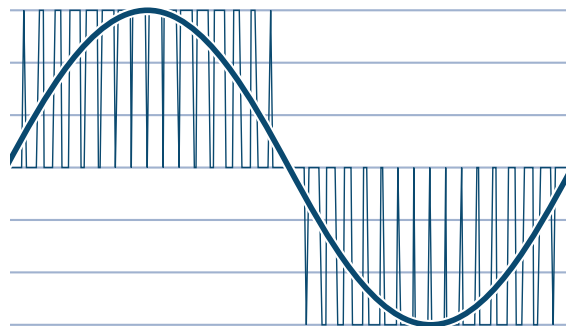
Figure 1. Sine wave overlaid on square carrier waves
