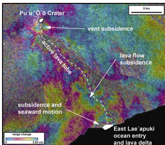
Figure 4. ASAR beam mode 3 track 365 interferogram spanning May 13 to September 30, 2006, and showing subsidence of recent lava flows and the vent region, as well as seaward motion of the coast above the lava delta (white area) caused by surface instability. Area covered by the image is shown in Fig. 1.
