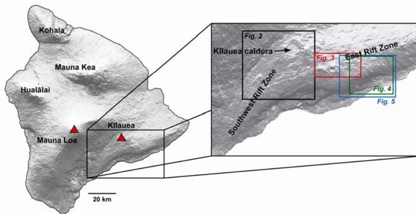
Figure 1. Map showing the locations of the major volcanic centers on the island of Hawai‘i. The summit calderas of Mauna Loa and Kīlauea, the most active volcanoes on the island, are indicated by red triangles. Zoomed map shows the areas on Kīlauea covered by Figs. 2-5
