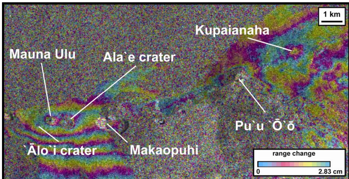
Figure 3. ASAR beam mode 2 track 429 interferogram spanning September 10, 2003 to February 21, 2007, showing deformation along Kīlauea's east rift zone. Labelled features are discussed in the text, and the area covered by the interferogram is given in Fig. 1.
