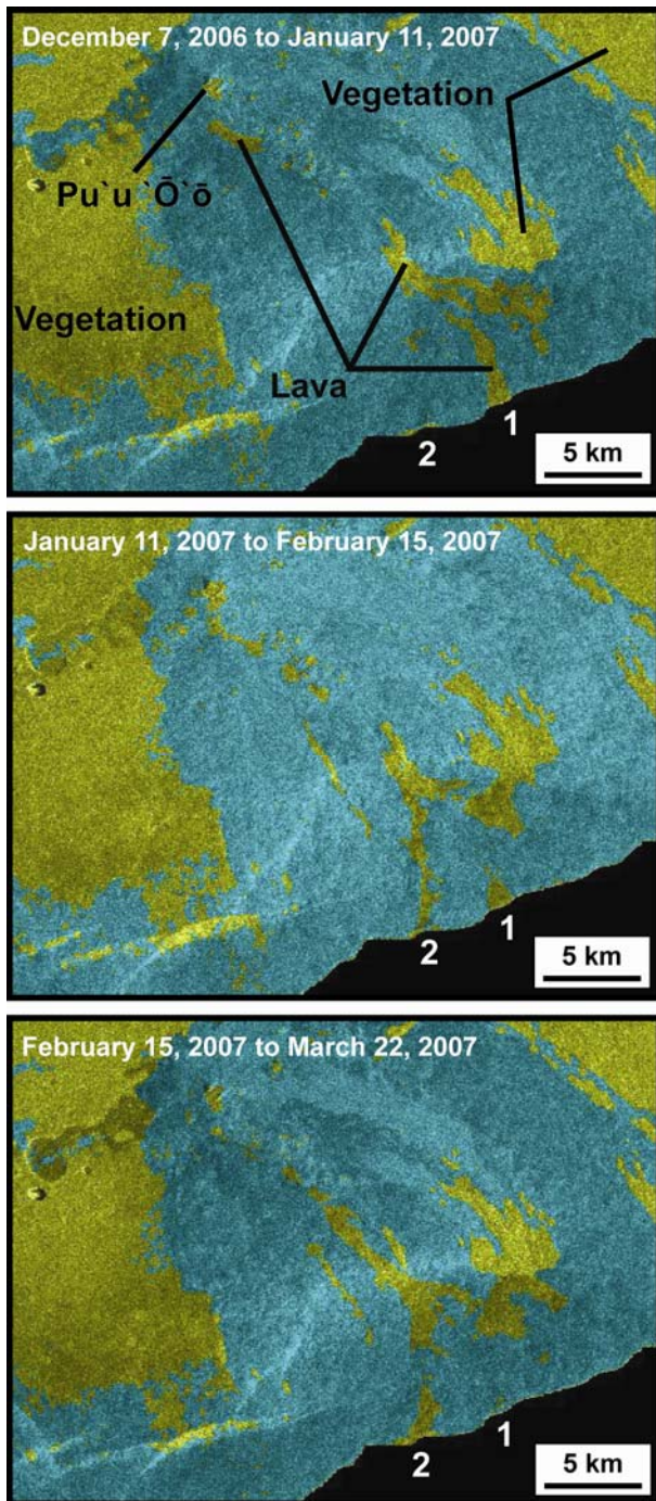
Figure 5. Coherence maps derived from ASAR beam mode 6 track 343 interferograms. Yellow areas have a coherence less than 0.3, and blue areas greater than 0.3. Area covered by the imagery is shown in Fig. 1.
