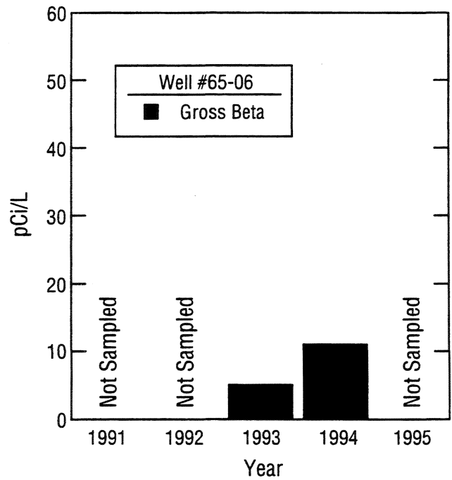
Figure 5-32 Yearly average Gross Beta concentration in wells located in the Waste Concentration Facility area (WCF): Wells 65-02, 65-03, and 65-05 are located at the downgradient margin of the WCF; and, Well 65-06 is located directly upgradient of the WCF.
