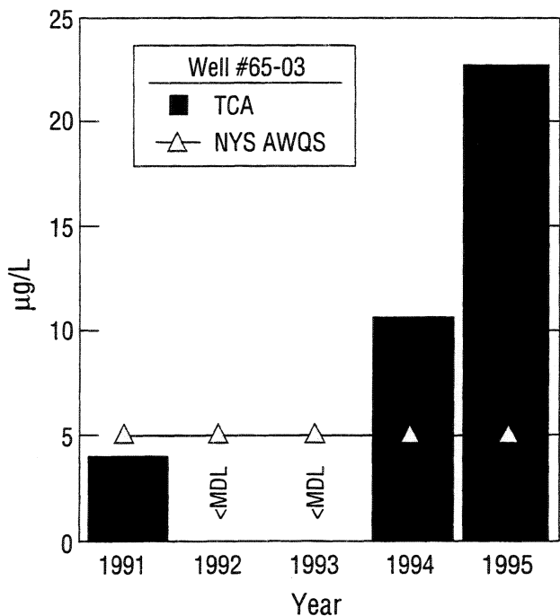
Figure 5-17 Yearly average concentration trends of 1,1,1-Trichloroethane in wells upgradient and downgradient of the Waste Concentration Facility (WCF): Well 65-06 located directly upgradient of the WCF; Wells 65-02, 65-03 and 65-05 are located directly downgradient of the WCF.
