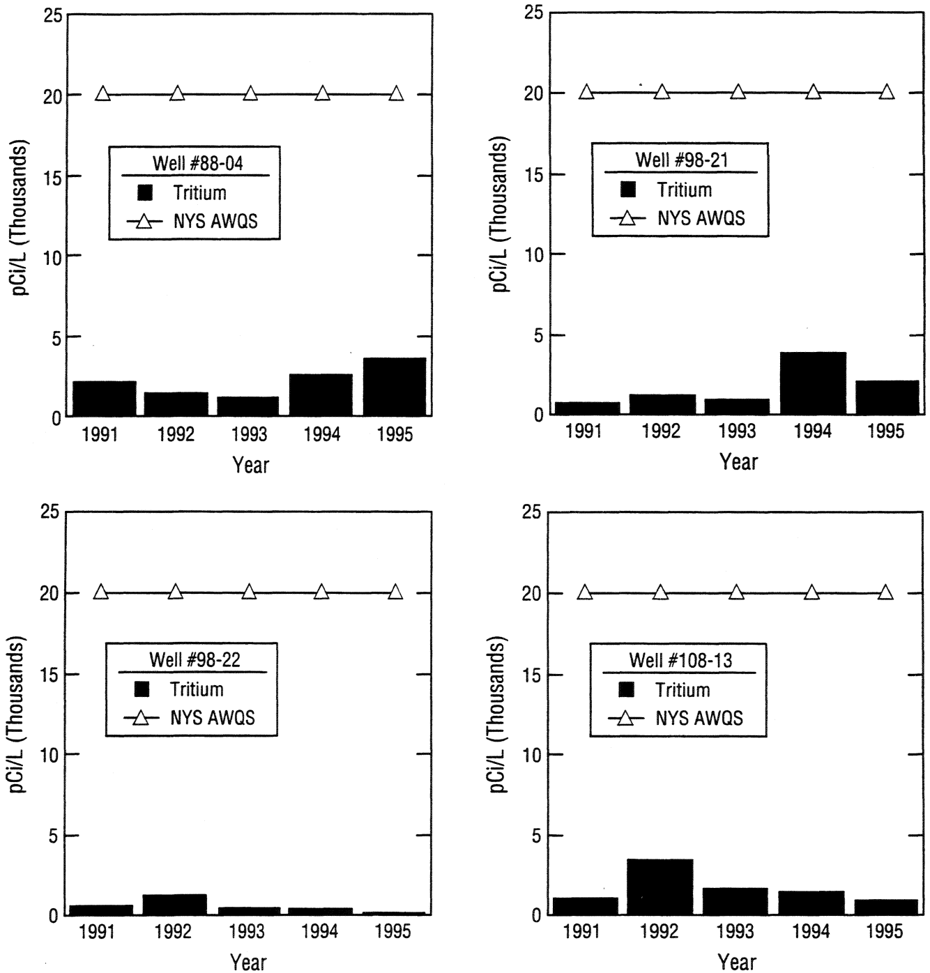
Figure 5-31 Yearly average concentration in wells located in the Hazardous Waste Management Facility area (HWMF): Well 88-04 is located within the HWMF; Well 98-22 is located at the downgradient margin of HWMF; Well 98-21 is located 110 m downgradient of the HWMF; and, Well 108-1 is located at the site boundary, 675 m downgradient of HWMF.
