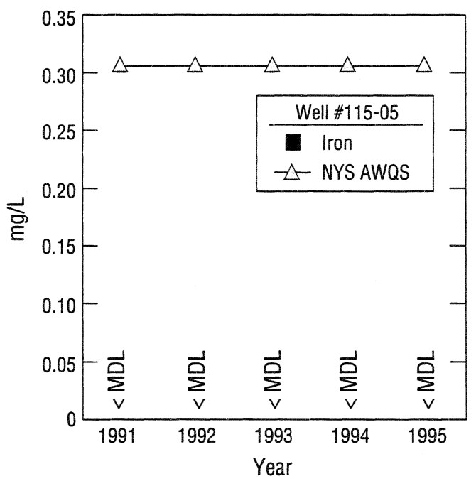
Figure 5-14 Yearly average concentration trends of Iron in wells upgradient and downgradient of the Current Landfill: Well 87-09 located at upgradient margin of landfill; Well 87-05 located at downgradient margin of landfill; Well 87-07 located 75m downgradient of landfill; and Well 115-05 located at the site boundary 1,225m downgradient of the landfill.
