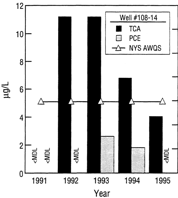
Figure 5-16 Yearly average concentration trends of 1,1,1-Trichloroethane (TCA) and Tetrachloroethylene (PCE) in wells upgradient and downgradient of the Hazardous Waste Management Facility (HWMF): Well 88-04 located within the HWMF; Well 98-21 located 110m downgradient of the HWMF; Well 108-14 located at the site boundary 675m downgradient of the HWMF; and Well 108-17 located at site boundary 680m downgradient of HWMF.
