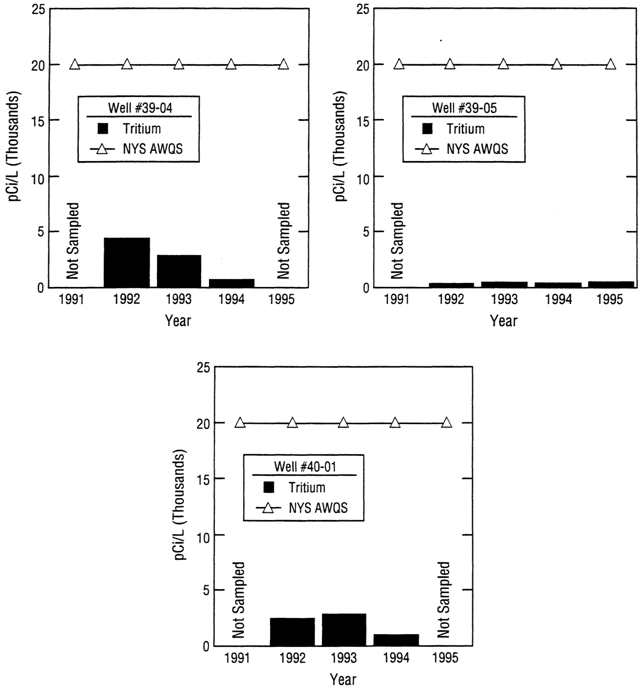
Figure 5-34 Yearly average Tritium concentration in wells located in the Peconic River area: Wells 39-05, 39-04 and 40-01 are located 310 m, 440 m, and 670 m downstream of EA respectively.
