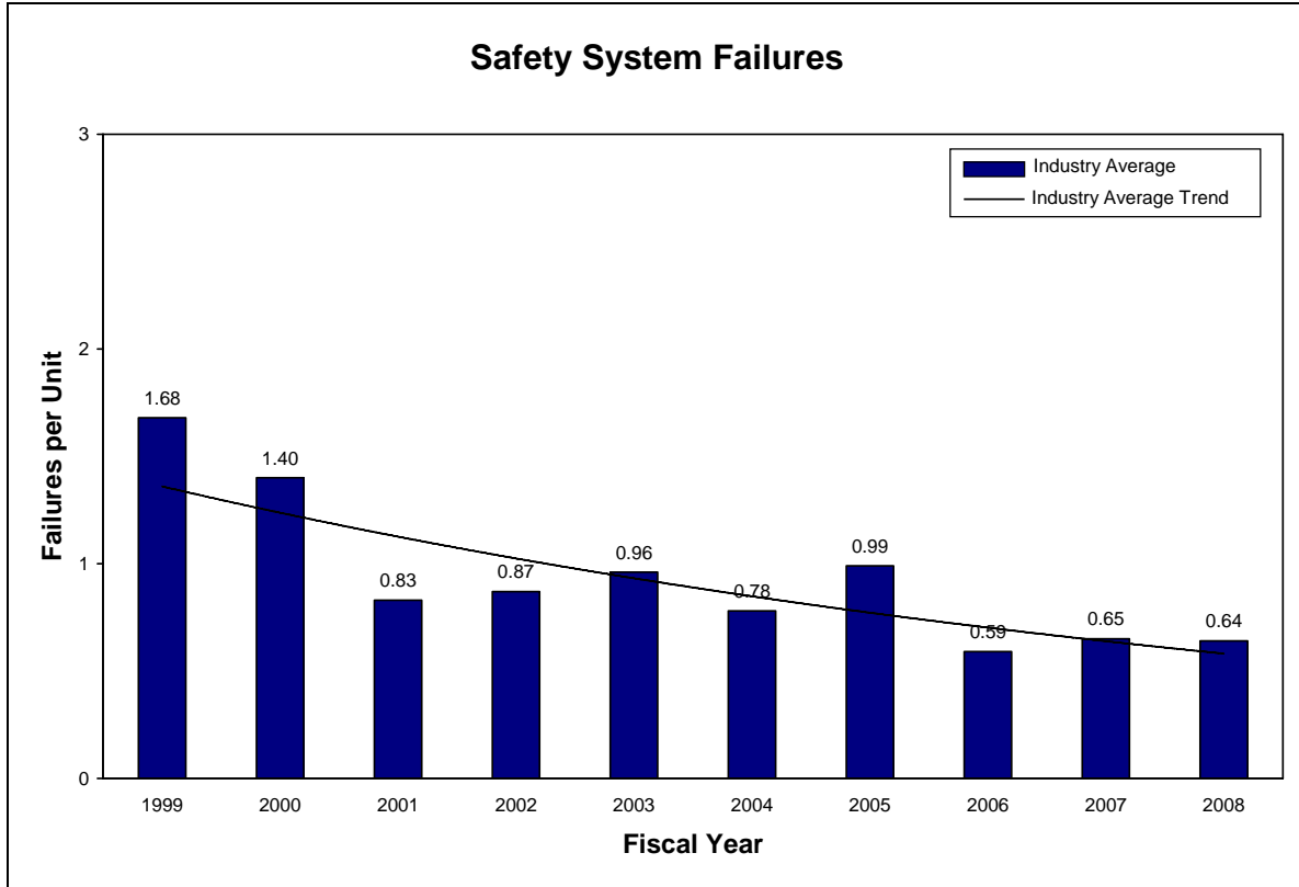
Figure 4. Safety System Failures
