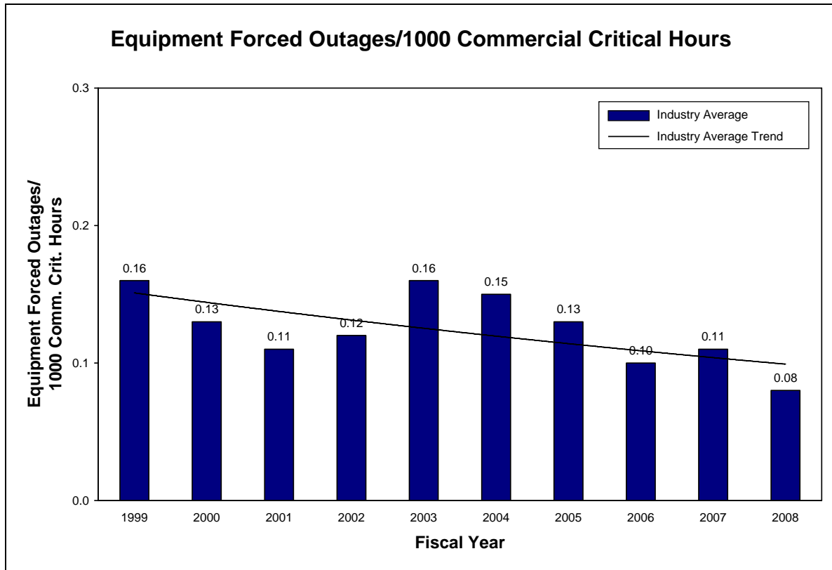
Figure 6. Equipment Forced Outages per 1000 Commercial Critical Hours
