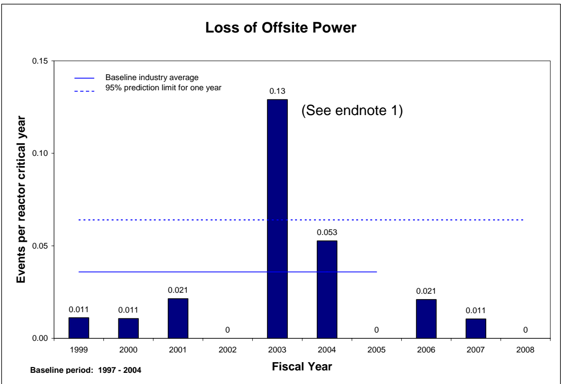
Figure 6. Loss of Offsite Power
