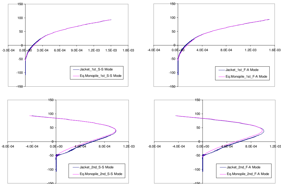
Figure 2.24 Modal Shapes of the Jacket Support Structure
