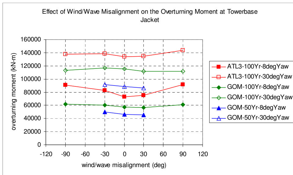
Figure 2.65 Turbine Tower Base Shear and Overturning Moment for the Jacket Case
