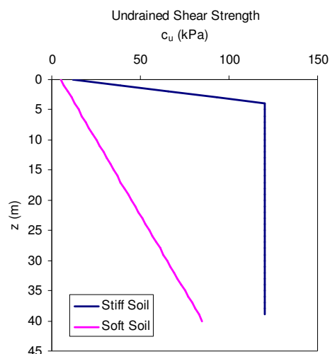
Figure 3.7 Undrained Shear Strength for Stiff and Soft Soil
