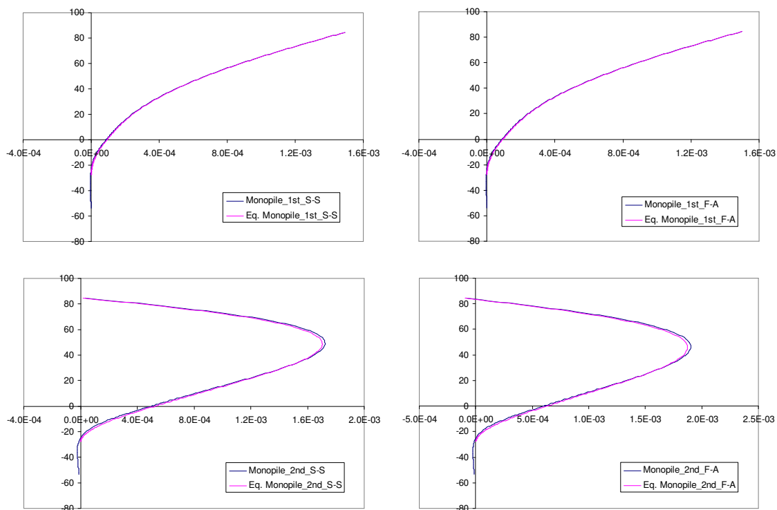
Figure 2.20 Modal Shapes of the Monopile Support Structure
