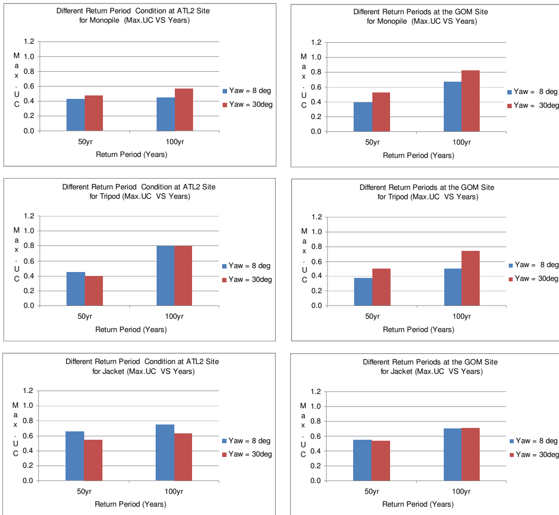
Atlantic Region 2 (ATL2) GOM West Central (GOM) Figure 2.59 Utilization Ratios (50-yr vs. 100-yr) at the ATL2 and GOM Regions
