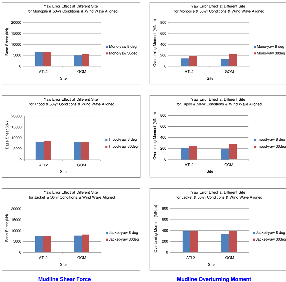
Mudline Shear Force Mudline Overturning Moment Figure 2.60 Mudline Shear Forces and Overturning Moments (Normal vs. Abnormal) under the 50-Year Return Conditions
