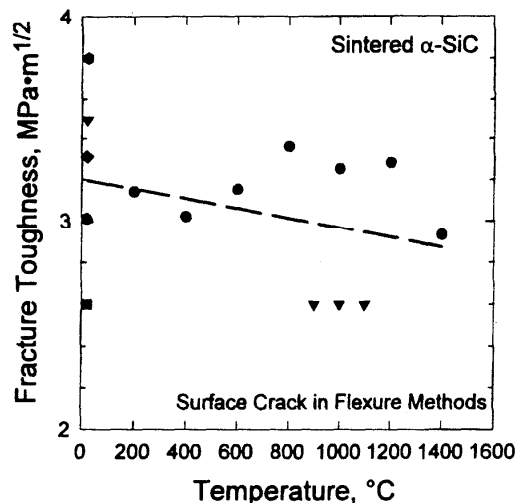
FIG. 8. The fracture toughness of sintered \alpha -SiC by surface crack in flexure methods.
