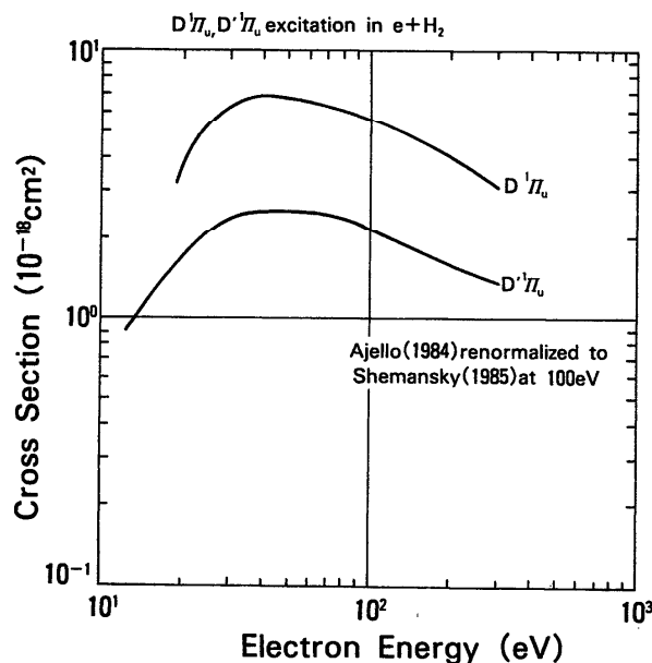
FIG. 9. Cross sections of electronic excitation to D and D'^1\Pi_u .
