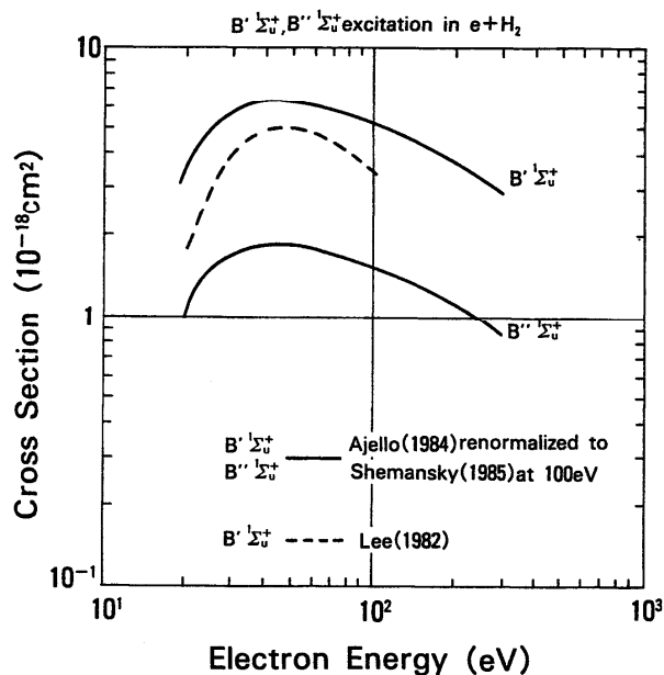
FIG. 7. Cross sections of electronic excitation to B' and B''^1\Sigma_u^+ .
