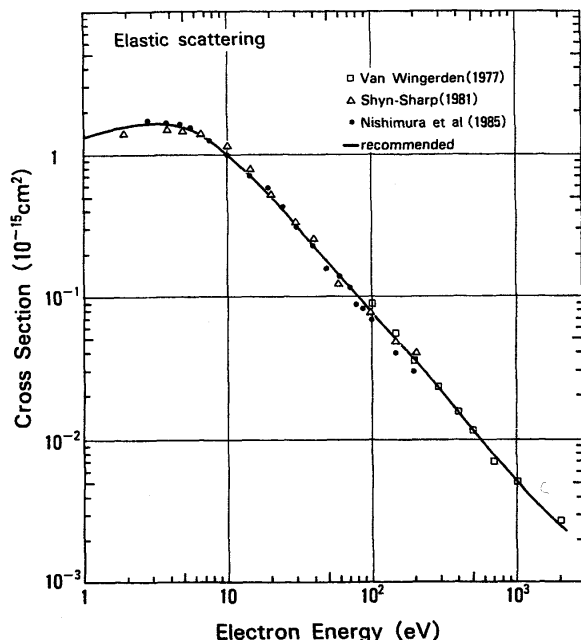
FIG. 3. Cross sections of elastic scattering.
