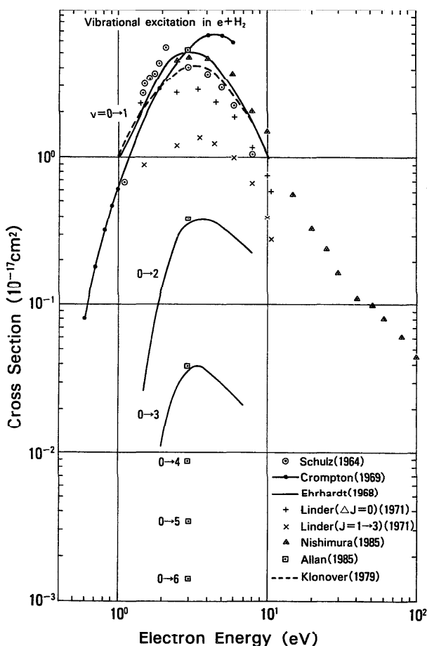
FIG. 5. Cross sections of vibrational excitation.
