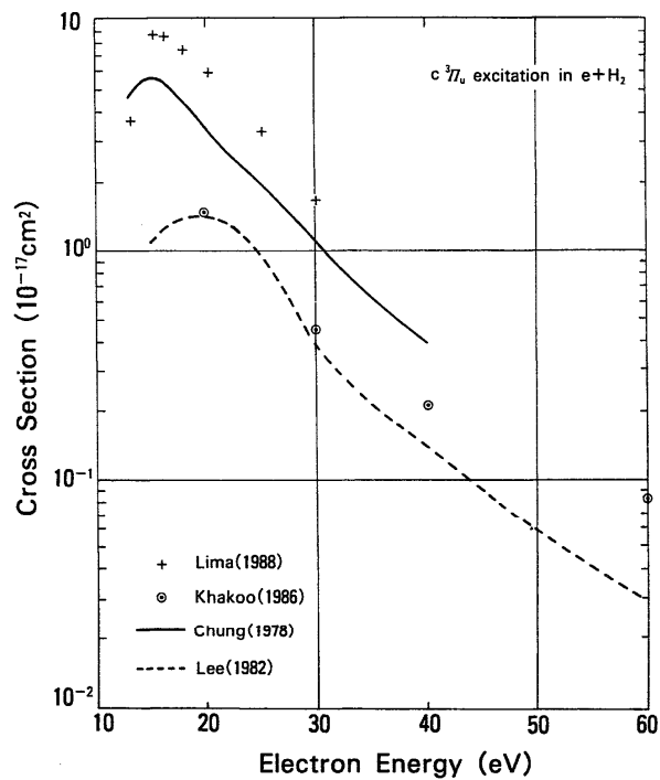
FIG. 13. Cross sections of electronic excitation to c^3\Pi_u .
