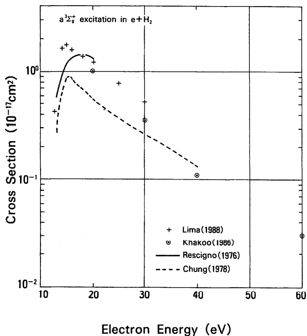
FIG. 11. Cross sections of electronic excitation to a^3\Sigma_g^+ .
