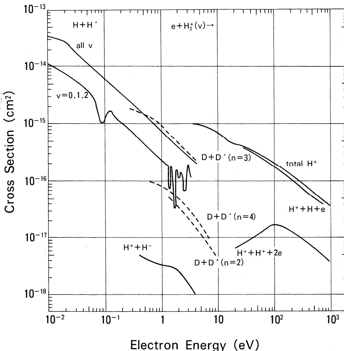
FIG. 18. Cross sections of electron collisions with H(v)_2^+ ions for the production of atomic hydrogens from all v , atomic hydrogens from v = 0, 1 and 2 , D + D^*(n = 2, 3, 4) , total protons, H^+ + H + e , H^+ + H^+ + 2e and H^+ + H^- .
