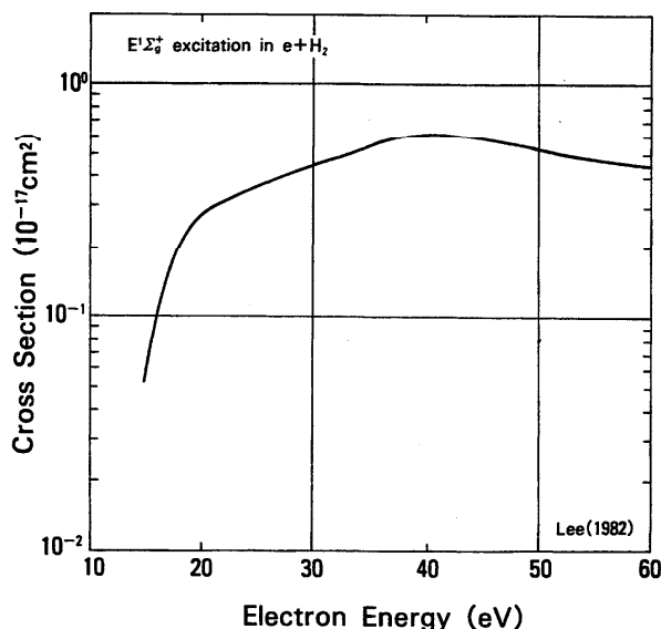
FIG. 10. Cross sections of electronic excitation to E^1\Sigma_g^+ .
