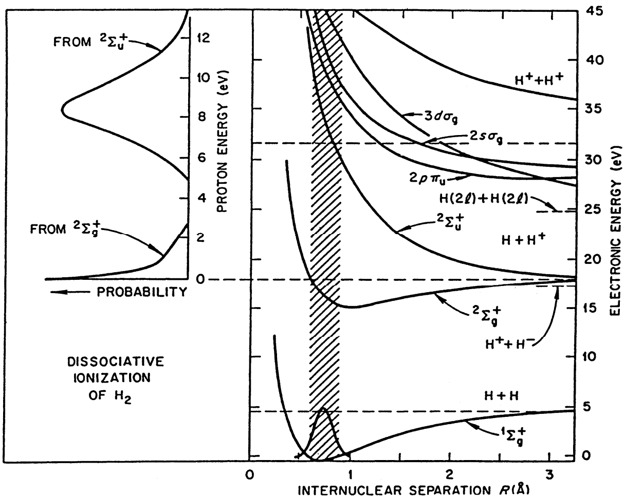
FIG. 21. Potential energy curves of H_2 , H_2^+ and H_2^{2+} and the expected energy distributions of protons produced via ^2\Sigma_g^+ and ^2\Sigma_u^+ states of H_2^+ in dissociative ionization of H_2 (see Ref. 115).
