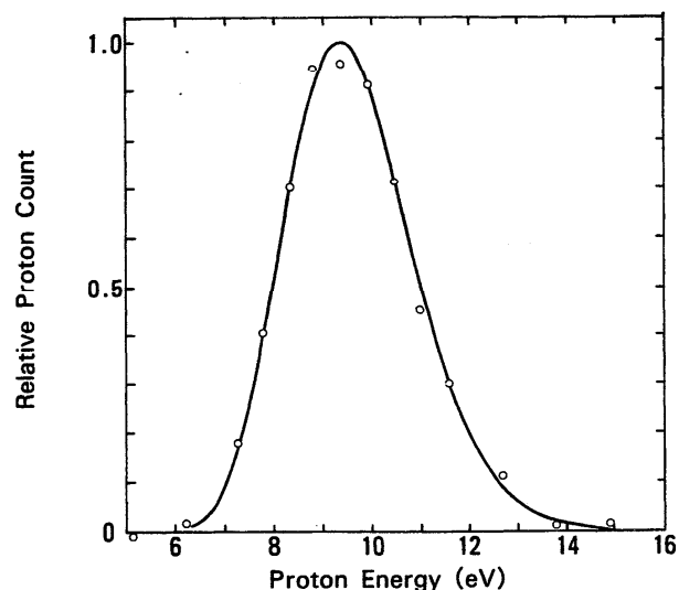
FIG. 27. Energy distribution of protons from doubly ionized hydrogen molecules in electron impact (see Ref. 124). The open circles denote the observed data, meanwhile the solid line represents the calculated distribution.
