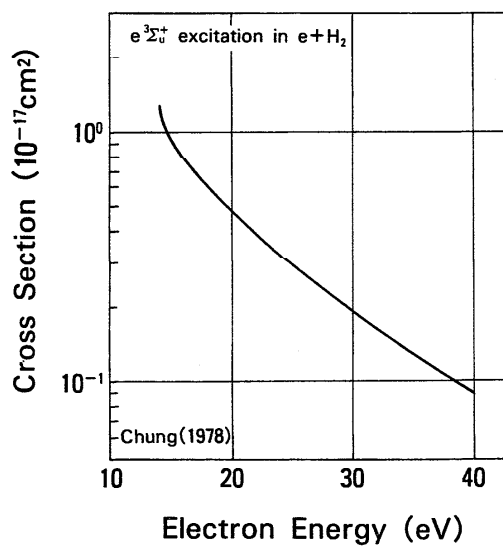
FIG. 14. Cross sections of electronic excitation to e^3\Sigma_u^+ .
