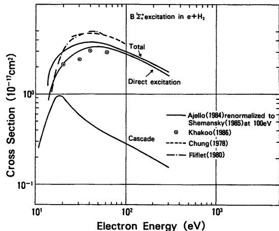
FIG. 6. Cross sections of electronic excitation to B^1\Sigma_u^+ .
