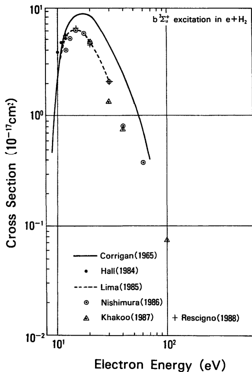
FIG. 12. Cross sections of electronic excitation to b^3\Sigma_u^+ .
