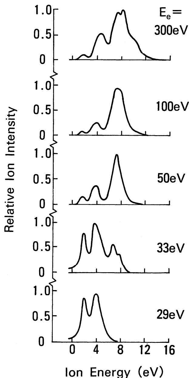
FIG. 24. Proton energy spectra at different electron impact energies. Note that the spectral shapes change with the electron impact energy (see Ref. 119).
