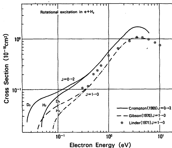
FIG. 4. Cross sections of rotational excitation.
