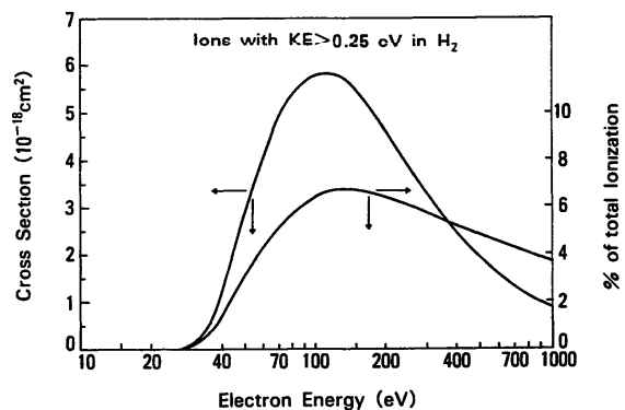
FIG. 23. Cross sections of production of protons with the energy above 0.25 eV and their fractions (see Ref. 117).
