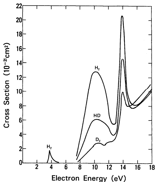
FIG. 17. Cross sections of dissociative attachment for HD and D 2 as well as H 2 (see Ref. 67).
