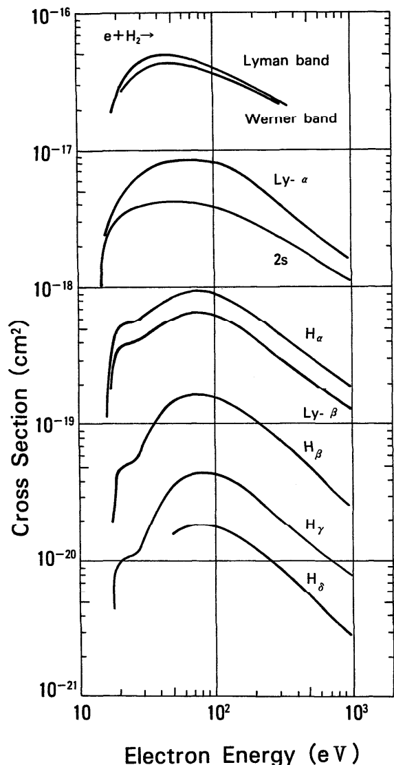
FIG. 15. Cross sections of photon emission for Lyman band, Werner band, Lyman- \alpha , Lyman- \beta , 2s state, Balmer- \alpha , - \beta , - \gamma and - \delta lines (see Ref. 125).
