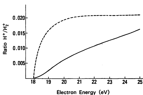
FIG. 22. Ratios of H^+/H_2^+ in electron impact. The solid curve shows these ratios in electron impact whereas the dashed curve represents those in photon impact (see Ref. 116).
