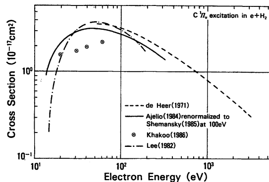
FIG. 8. Cross sections of electronic excitation to C^1\Pi_u .
