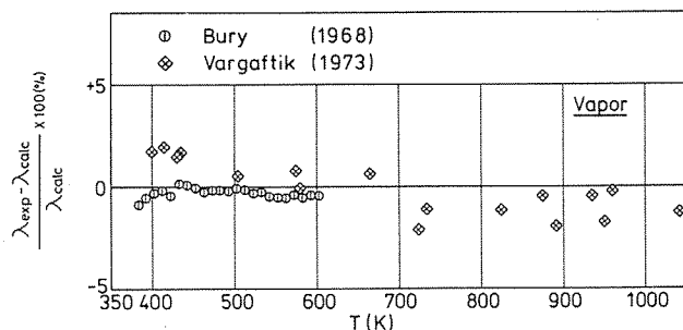
FIGURE 35. Deviation plot: thermal conductivity (selected data, vapor, 1 atm).
