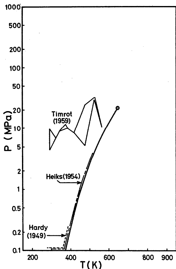
FIGURE 1. Experimental studies of viscosity of D_2O (prior to 1963).
