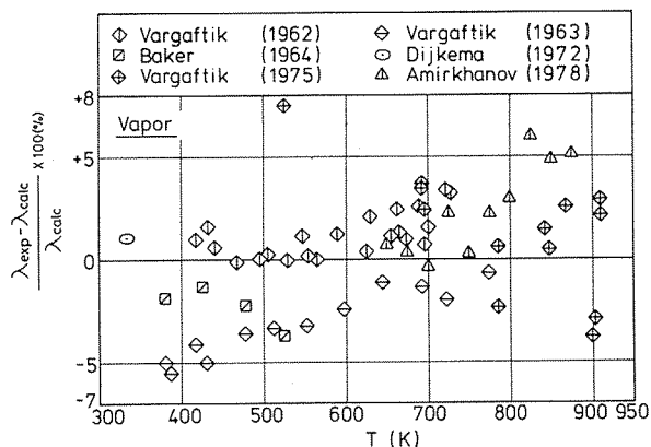
FIGURE 36. Deviation plot: thermal conductivity (remaining data, vapor, 1 atm).
