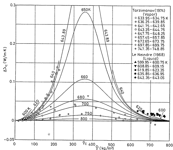
FIGURE 43. Critical enhancement of thermal conductivity.
