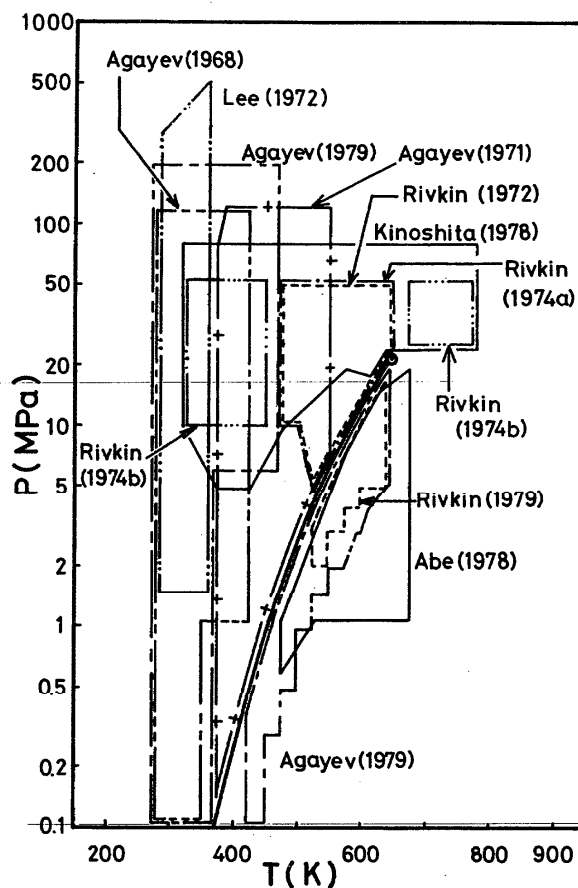
FIGURE 2. Experimental studies of viscosity of D_2O (after 1963).
