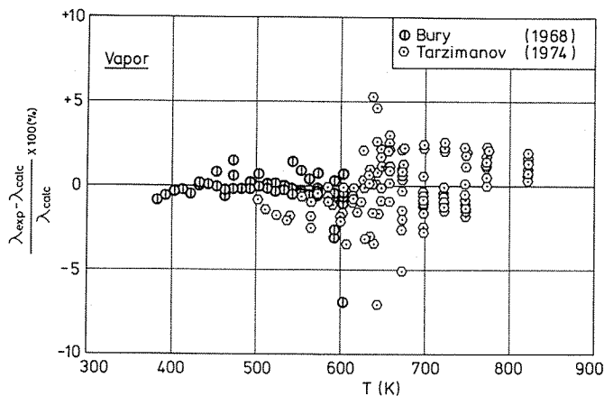
FIGURE 41. Deviation plot: thermal conductivity (selected data, vapor, high pressure).
