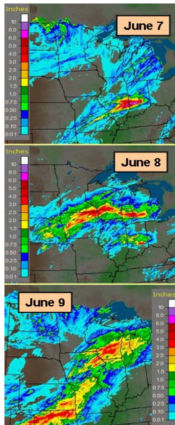
Fig. 6. Precipitation for 24-hour periods ending 12 UTC June 7-9, 2008. (Source: NOAA/NWS, http://water.weather.gov/. )
