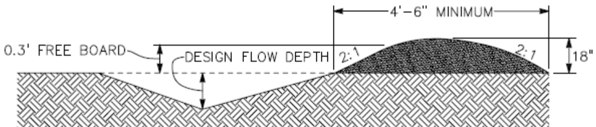
Typical Vee-Shaped Diversion
