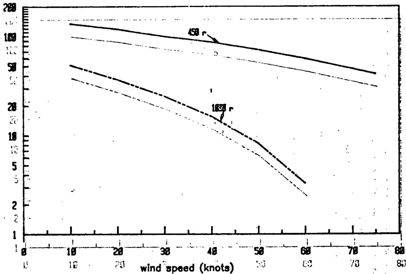
Fig. 10--Impact of wind speed on the lethal area covered by a single fallout pattern
