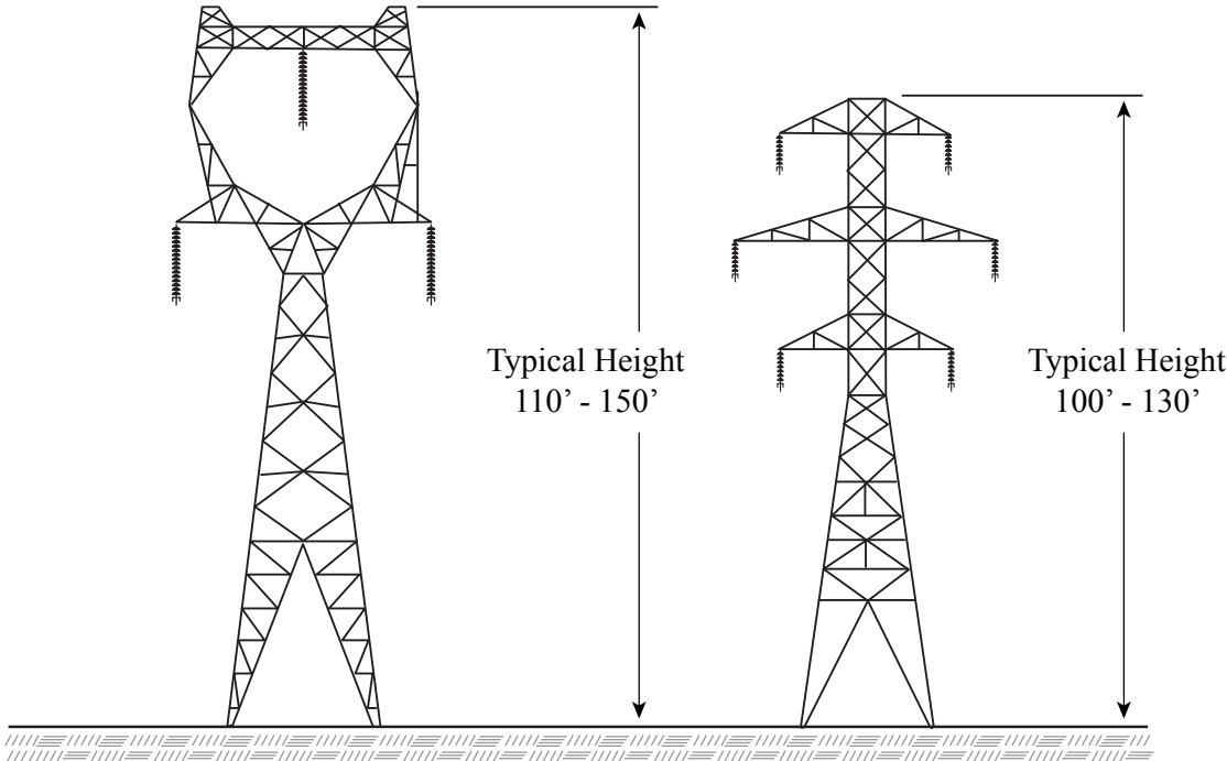
500-kV Single Circuit and 230-kV Double Circuit
