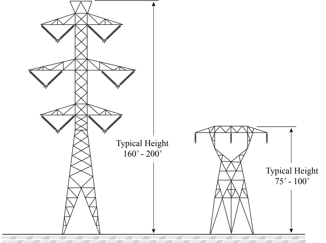
500-kV Double Circuit and 230-kV Single Circuit (one side operated at 230-kV)
