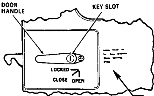
CABIN DOOR EXTERIOR RELEASE HANDLE VIEW LOOKING INBOARD LEFT SIDE (SAME FOR RIGHT SIDE)
