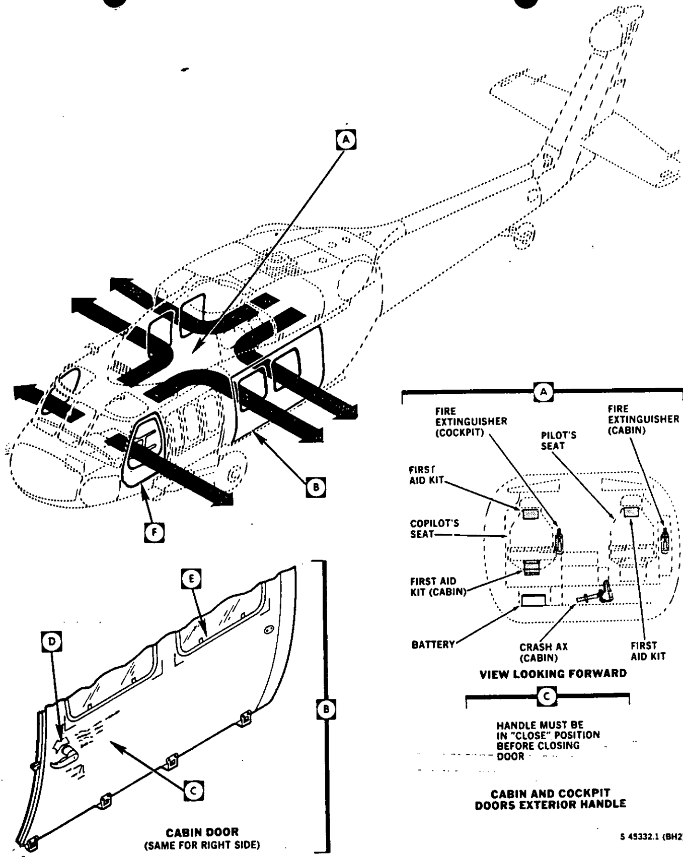
Figure 9-1. Emergency Exits and Emergency Equipment Diagram (Sheet 1 of 2)
