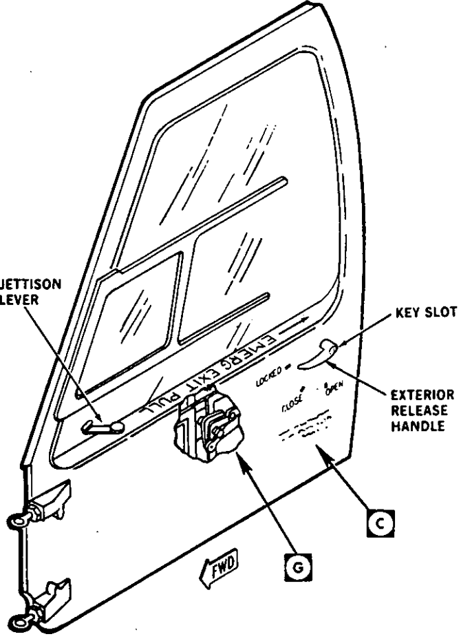
COCKPIT DOOR INTERIOR JETTISON LEVER VIEW LOOKING INBOARD LEFT SIDE (SAME FOR RIGHT SIDE)
