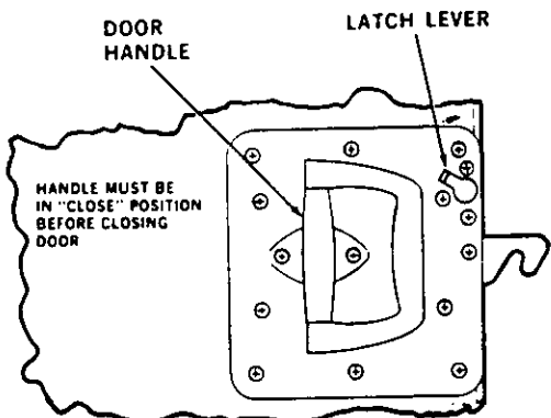
CABIN DOOR INTERIOR RELEASE HANDLE VIEW LOOKING OUTBOARD LEFT SIDE (SAME FOR RIGHT SIDE)
