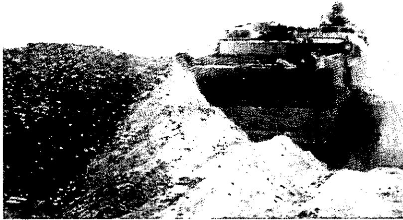
Figure VIII-32 Engineer Equipment Typical of that Used in 1st Infantry Division Breaching Operations
