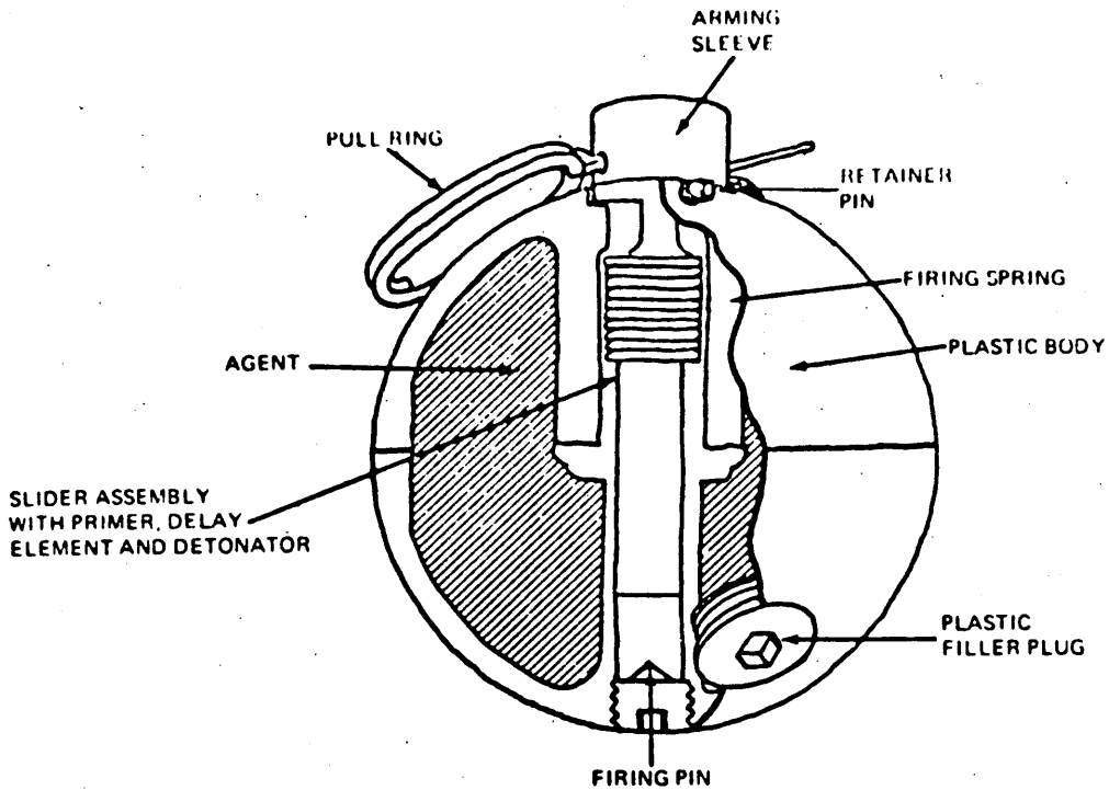
FIGURE 5. MILITARY M25A2 CS1 GRENADE (U)
