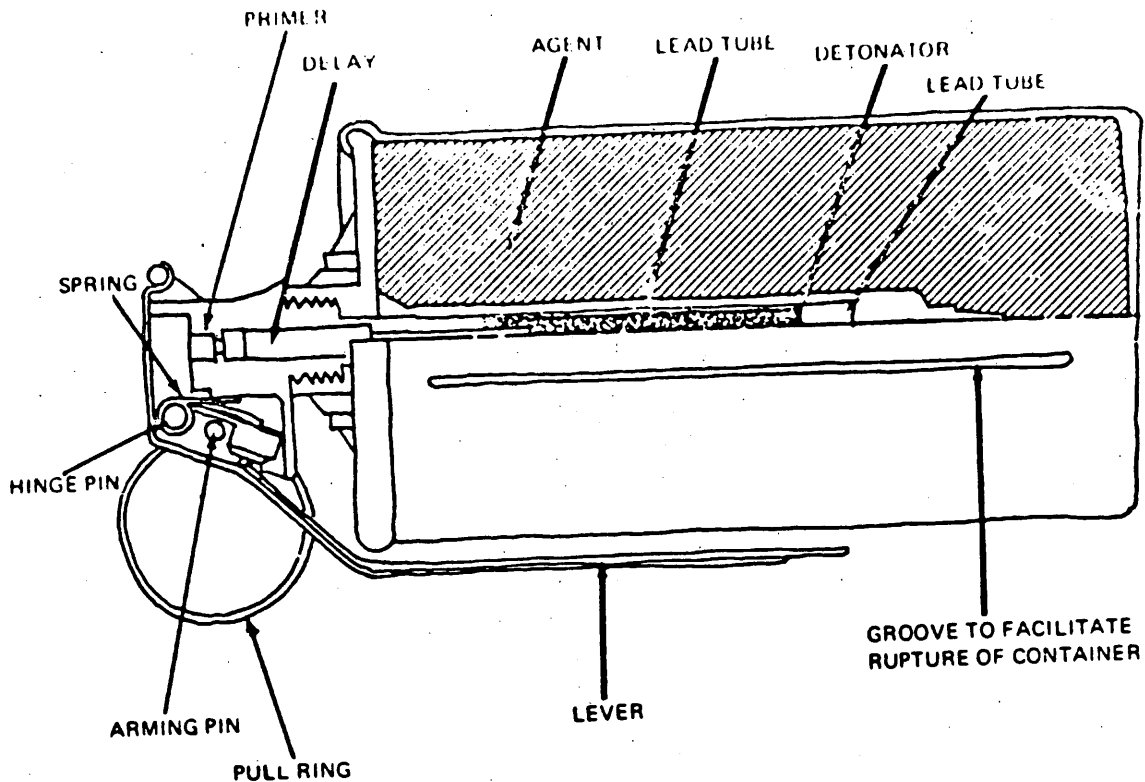
FIGURE 6. FEDERAL BLAST DISPERSION GRENADE (U)
