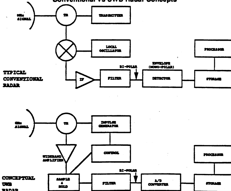
Conventional Vs UWB Radar Concepts
