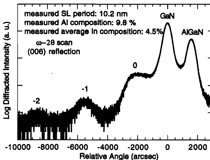
Figure 15. X-ray diffraction scan of a five-period InGaN MQW heterostructure with AlGaN ( x=0.098 ) cladding layers grown on a GaN/sapphire wafer.
