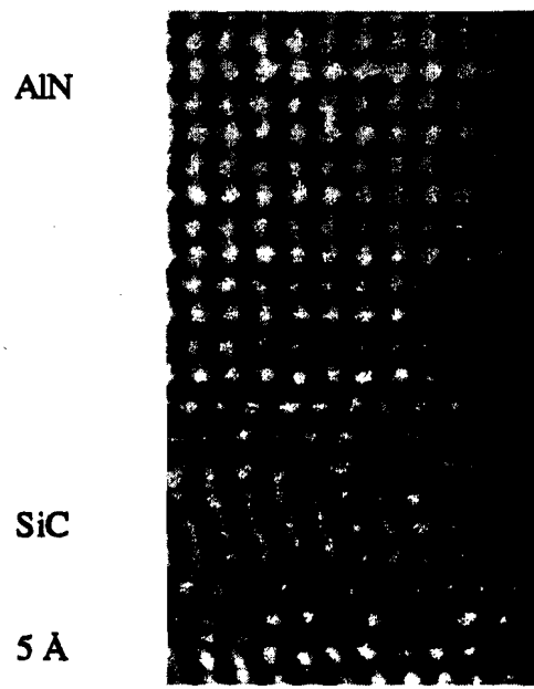
Figure 5. Lattice image of the AlN/SiC interface, for objective lens defocus of -105nm and specimen thickness of 8.5nm.
