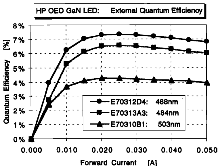
Figure 9. External quantum efficiency versus forward current. Peak quantum efficiencies are obtained at approximately 25 mA for all three devices.
