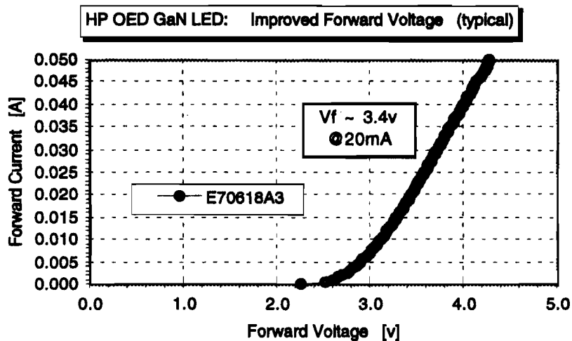
Figure 8. An improved wafer fabrication process reduces the typical forward voltage on a blue HP LED to approximately 3.4 Volts at 20 mA, with a series resistance of 28Ω.
