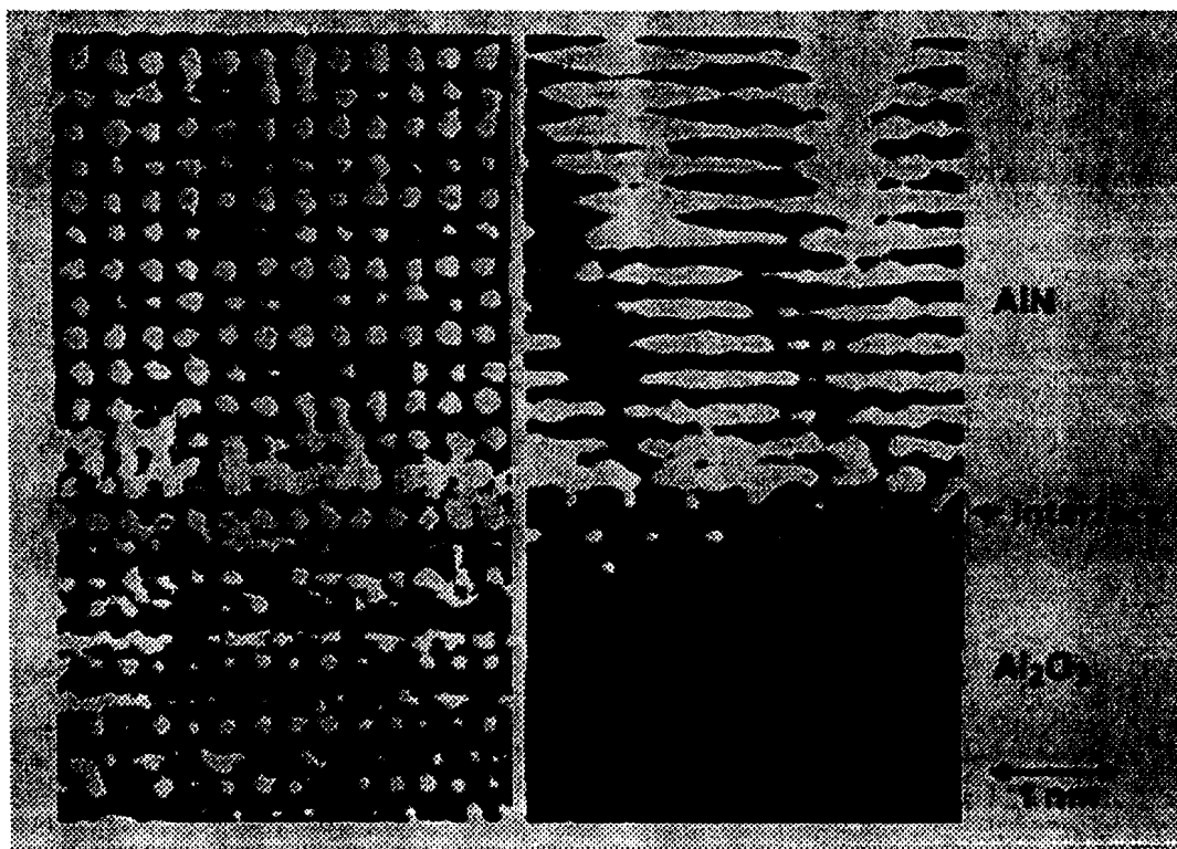
Figure 5. Lattice images of the \text{AlN}/\text{Al}_2\text{O}_3 interface taken in the (a) [01-10] and (b) [11-20] projections of the same interface region.
