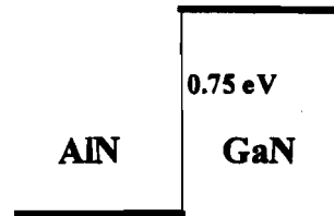
Fig. 6. Unstrained valence-band offset between GaN and AlN.
