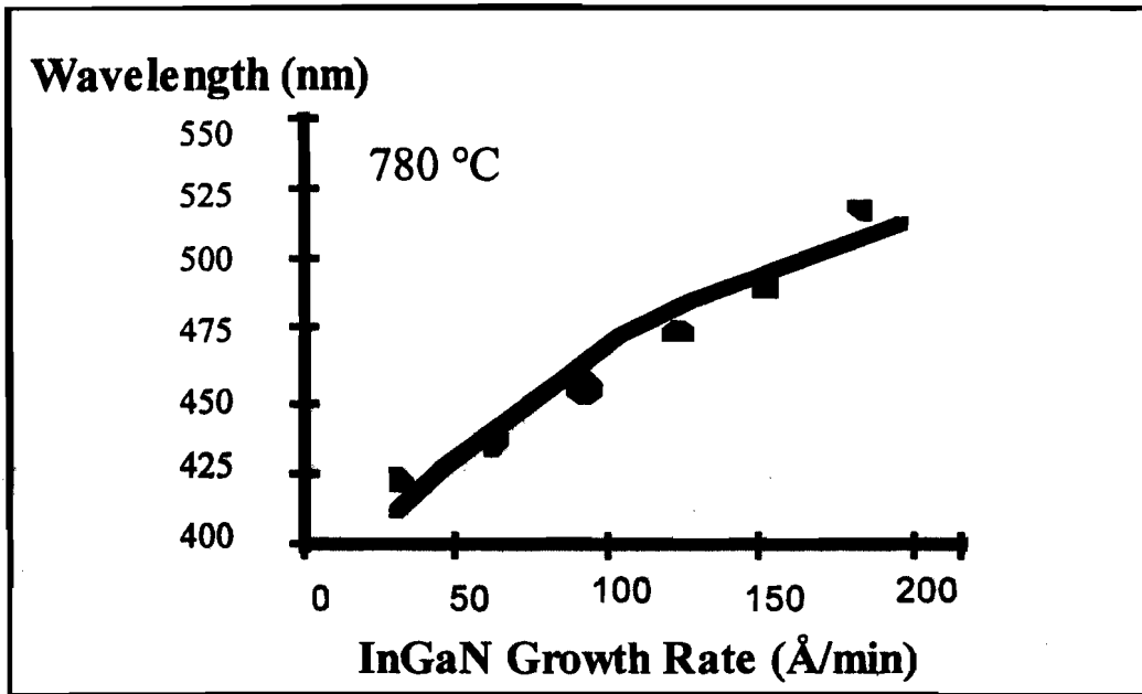
Fig. 3. Effect of growth rate on In incorporation.
