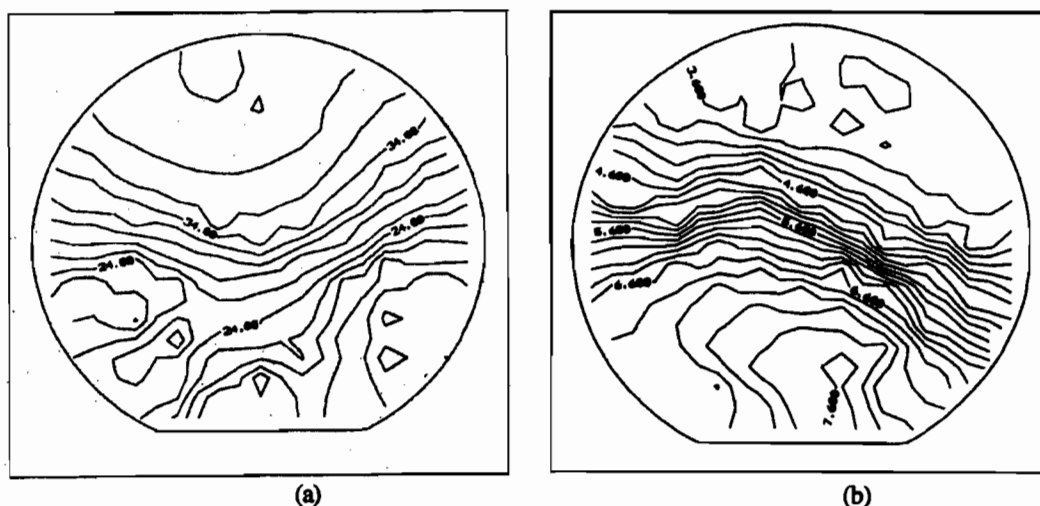
Figure 6. 2D maps of sheet resistance vs. position measured across 2" diameter wafers of (a) undoped (ave: 29 Ω/sq.) and (b) Si-doped (ave: 5.5 Ω/sq.) HVPE GaN-on-sapphire grown by HVPE.
