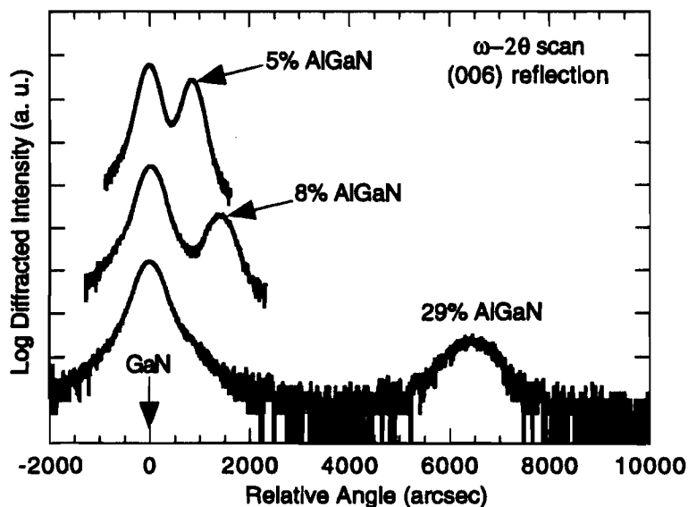
Figure 14. X-ray diffraction data for AlGaN/GaN films grown by MOCVD. The corresponding alloy compositions are indicated.
