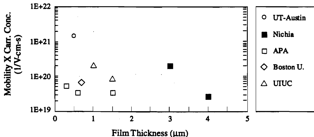
Fig. 7.16 Dependence of the mobility-carrier concentration product (at 300K) upon layer thickness for one of our GaN/sapphire films and recently published data from other groups for thicker GaN/sapphire films.
