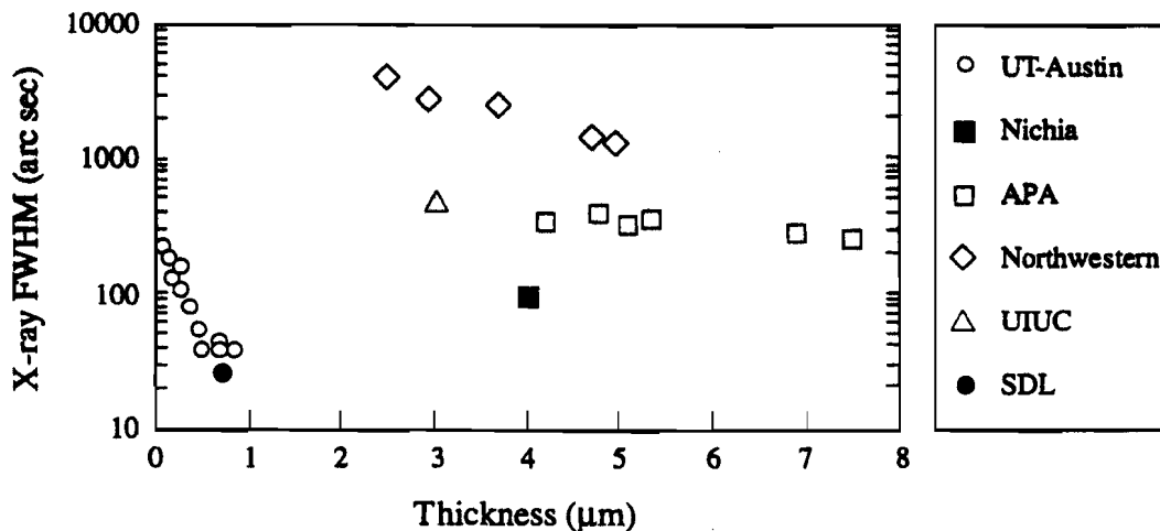
Fig. 7.5 Comparison of reported X-ray FWHM values of GaN/Al 2 O 3 heteroepitaxial films vs. layer thickness. Data are from indicated references.
