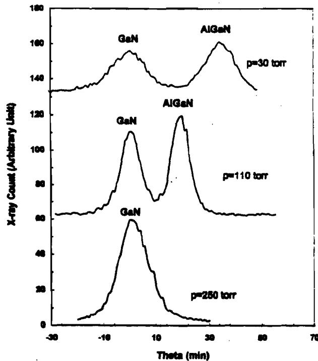
Figure 13: X-ray rocking curves for AlGaIn/GaN heterostructures vs reactor pressure.
