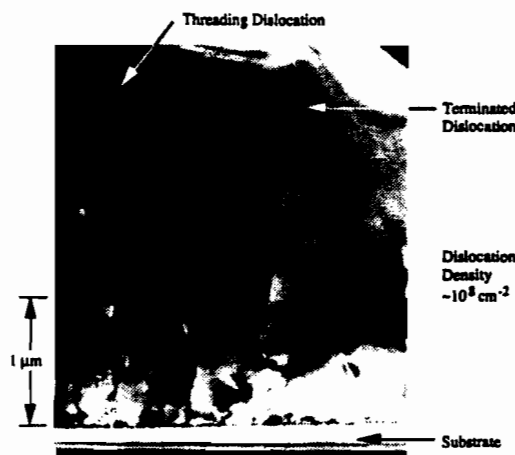
Fig. 7.9 TEM micrograph showing the GaN/AlN/SiC epitaxial structure grown at SDL. The dislocation density is \sim 10^8 \text{ cm}^{-2} .
