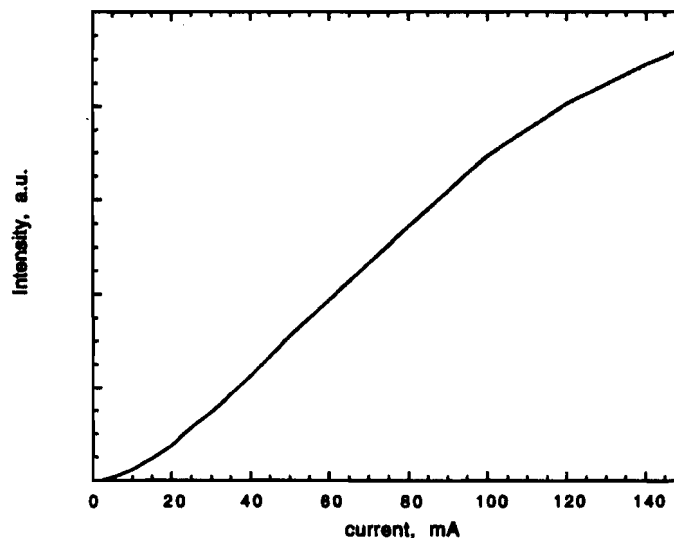
Figure 13. Intensity of electroluminescence versus injection current from a ridge waveguide heterostructure 5\mu\text{m} \times 550\mu\text{m} in area. Heating upon cw injection above 5\text{kA}/\text{cm}^2 and/or poor facets (angled due to failure of temperature control on CAIBE sample stage) precluded observation of stimulated emission.
