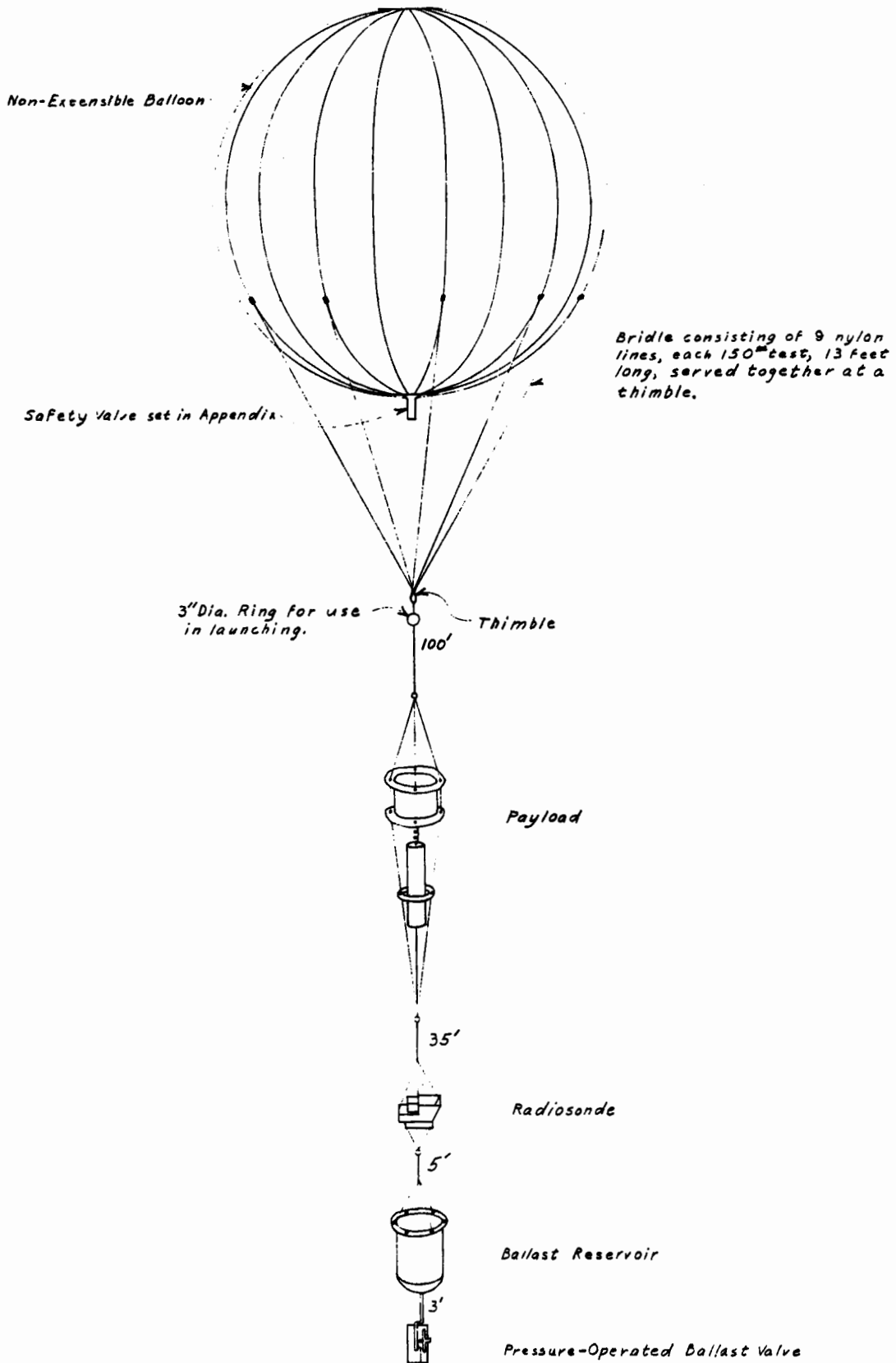
PROPOSED ASSEMBLY OF TRAIN FOR CONSTANT LEVEL BALLOON
