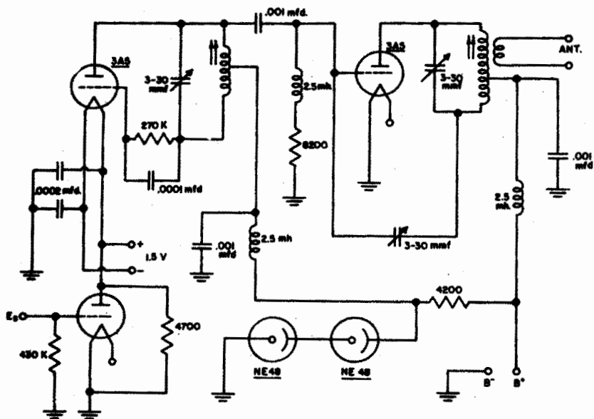
Fig. 5 FM-2 Transmitter
