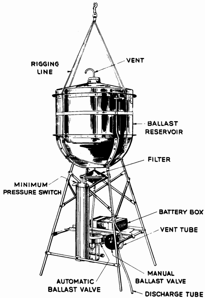
BALLAST RELEASE ASSEMBLY
