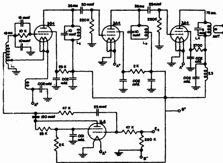
fig. 4 FM-1 Transmitter
