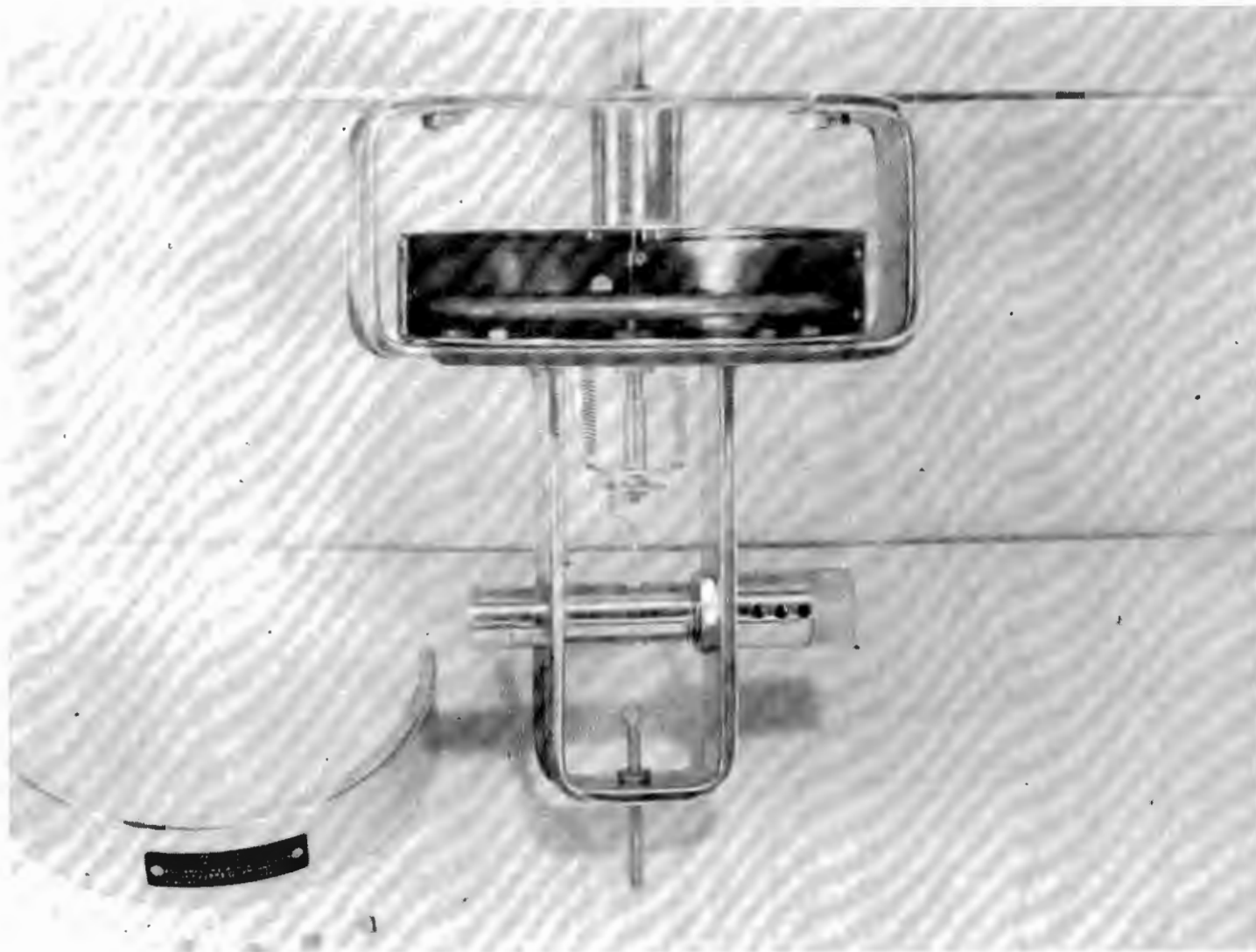
Figure 12 Automatic ballast valve, showing loading diaphragm.
