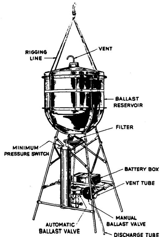
FIG. 3. Ballast-release assembly.
