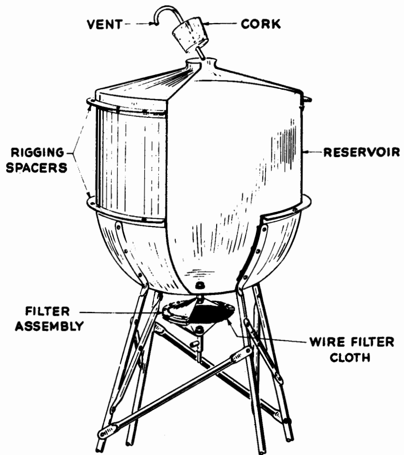
BALLAST RESERVOIR
