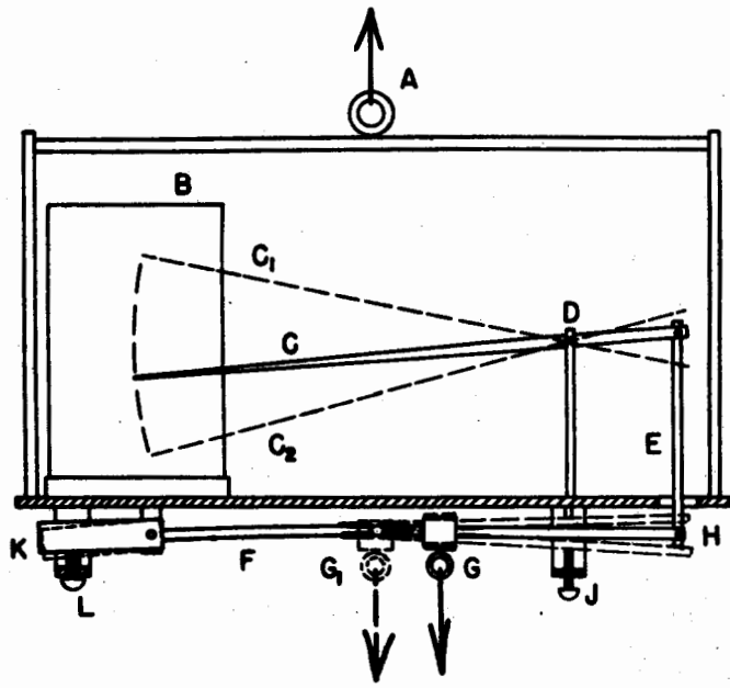
Figure 38. Ballast-recording meter.
