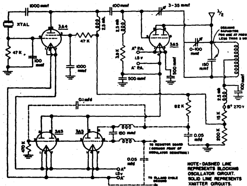
Fig. 6 AM-1 Transmitter
