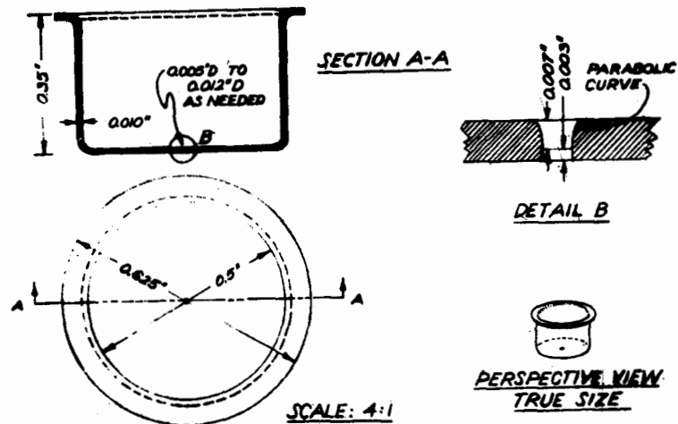
Figure 8. Orifice for fixed-rate ballast flow.
