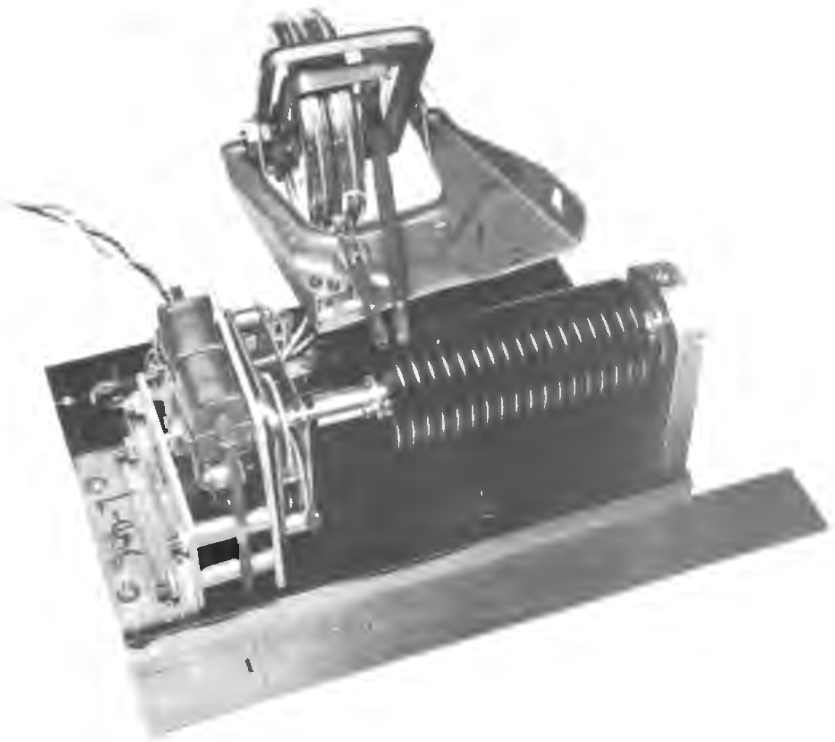
Figure 31 Olland Cycle Pressure Modulator
