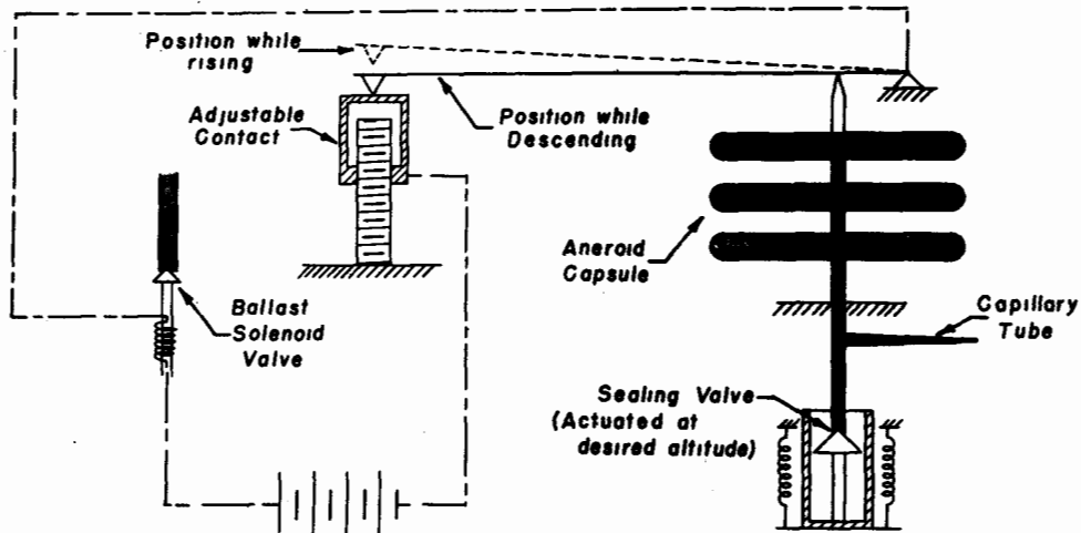
Figure 16. Rate-of-descent switch.
