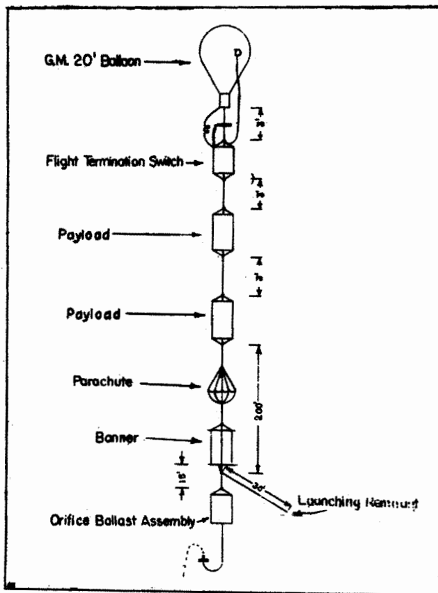
Fig. 10 Flight Train, Service Flight
