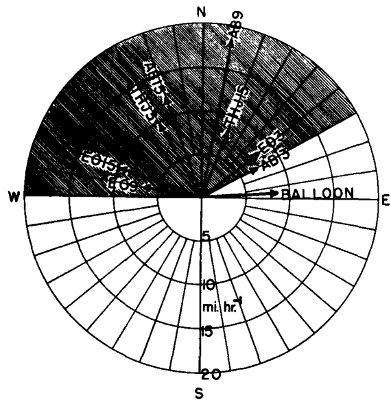
FIG. 8. Wind vectors at 16,000 feet for El Paso (EO), Albuquerque (AB), and Roswell (THJ), at 03 h , 09 h and 15 h (MST) on 7 July 1947, in connection with balloon Flight 11, mean motion of which is shown by the balloon vector. Cross-hatched sector contains all wind vectors at these three stations for the three observation hours and for the three levels, 14,000, 16,000, and 18,000 feet.
