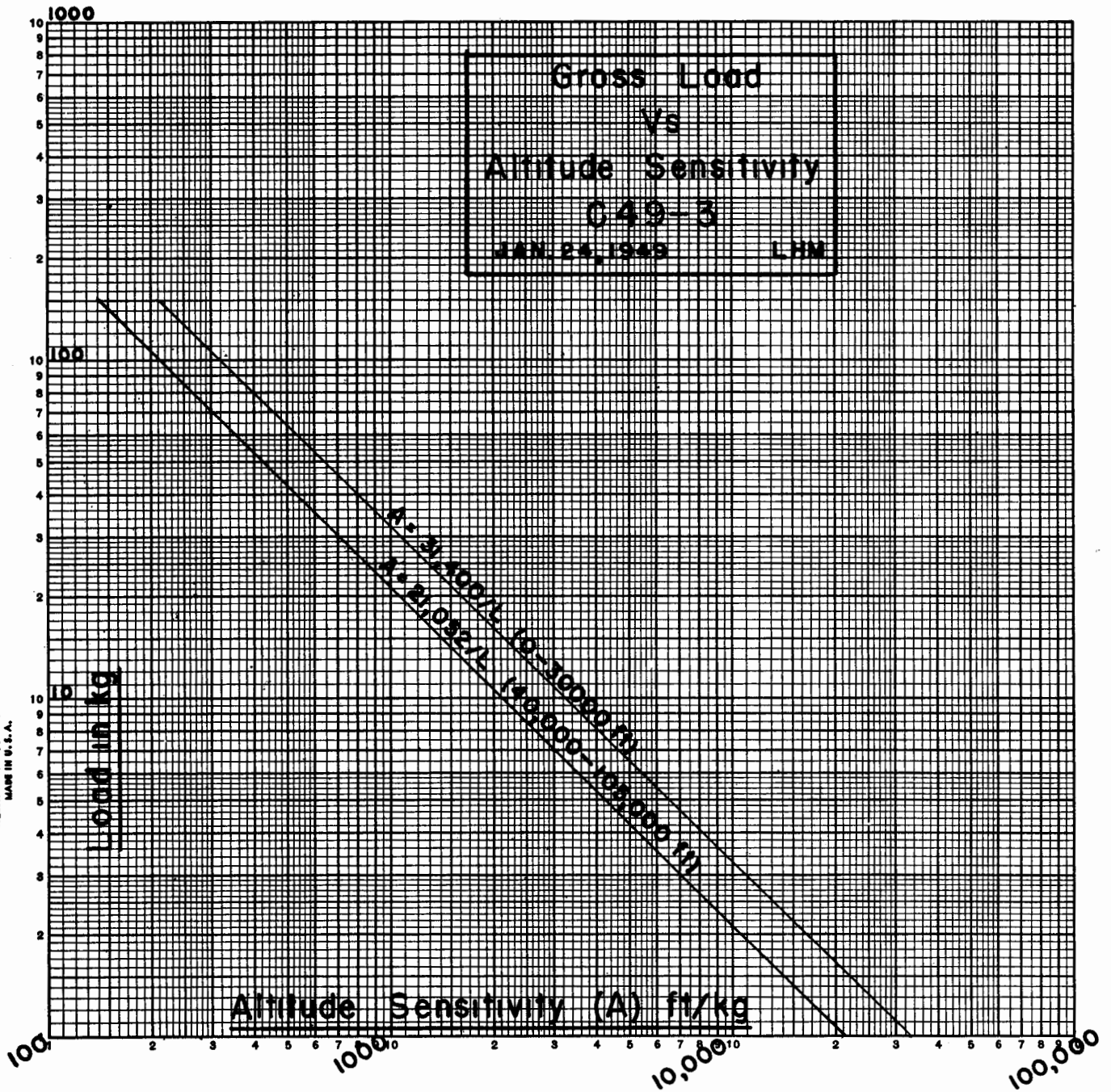
Graph 4
