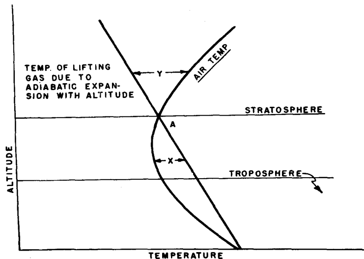
Figure 22. Lapse rate of air and helium.
