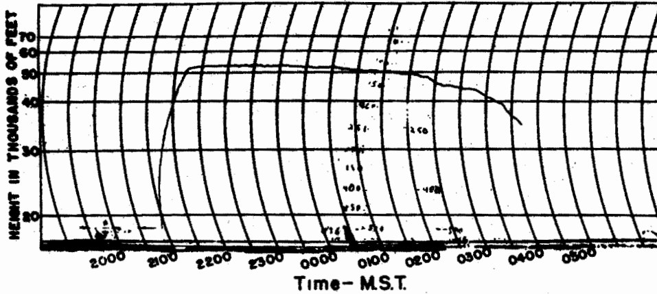
NYU BALLOON PROJECT FLIGHT 71 Barograph Record Of GM. 20 Ft. Plastic Balloon Showing Balloon Performance When No Ballast Was Dropped RELEASED AT ALAMOGORDO N.M., 2042 MST - 9 JULY, 1948 RECOVERED AT VALENTINE TEXAS, 10 JULY, 1948 ESTIMATED DURATION 10 HOURS
