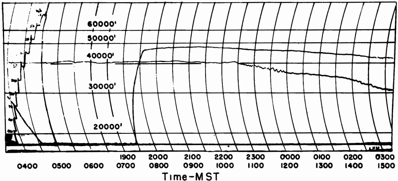
NYU BALLOON PROJECT FLIGHT 55 Barograph Record Of G.M. 20 Ft. Balloon With Automatic Ballast Valve RELEASED AT ALAMOGORDO, N.M., 1907 MST- 3 MAY, 1948 RECOVERED AT NORTHEAST, PA., 4 MAY, 1948 DURATION 23 HOURS
