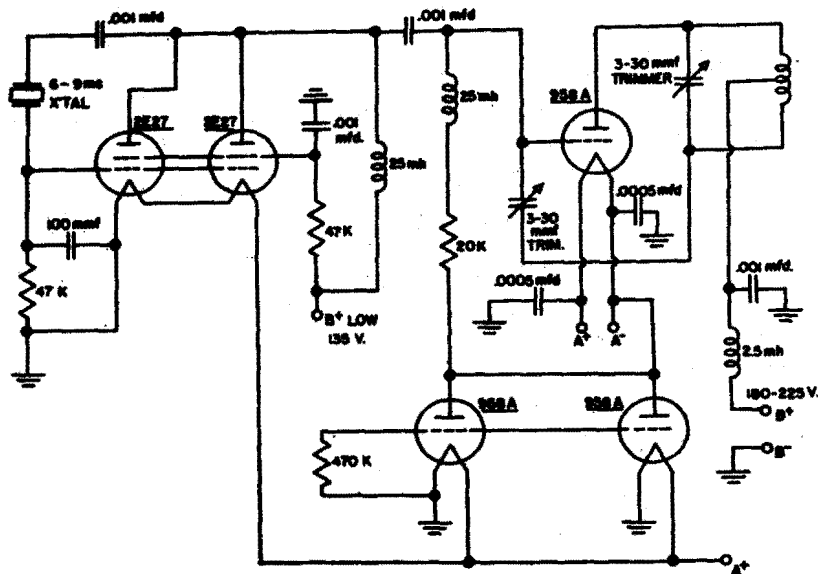
Fig. 7 AM-2 Transmitter
