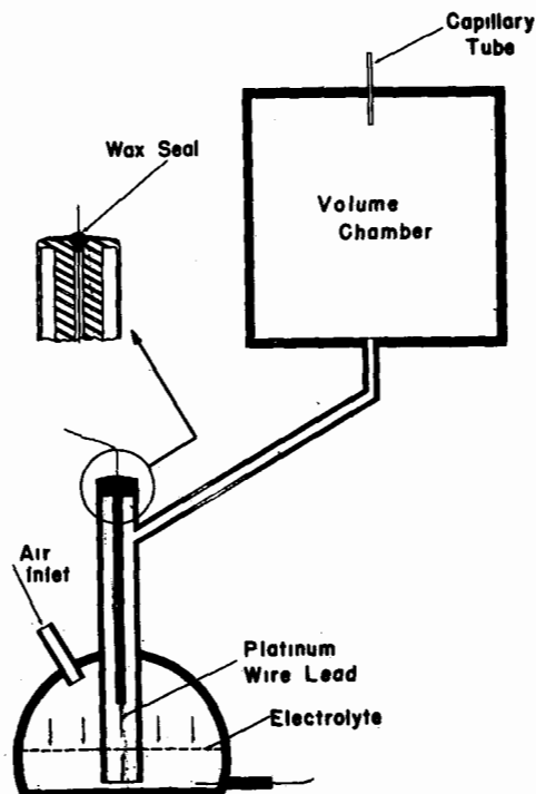
Figure 12. Rate-of-ascent switch.
