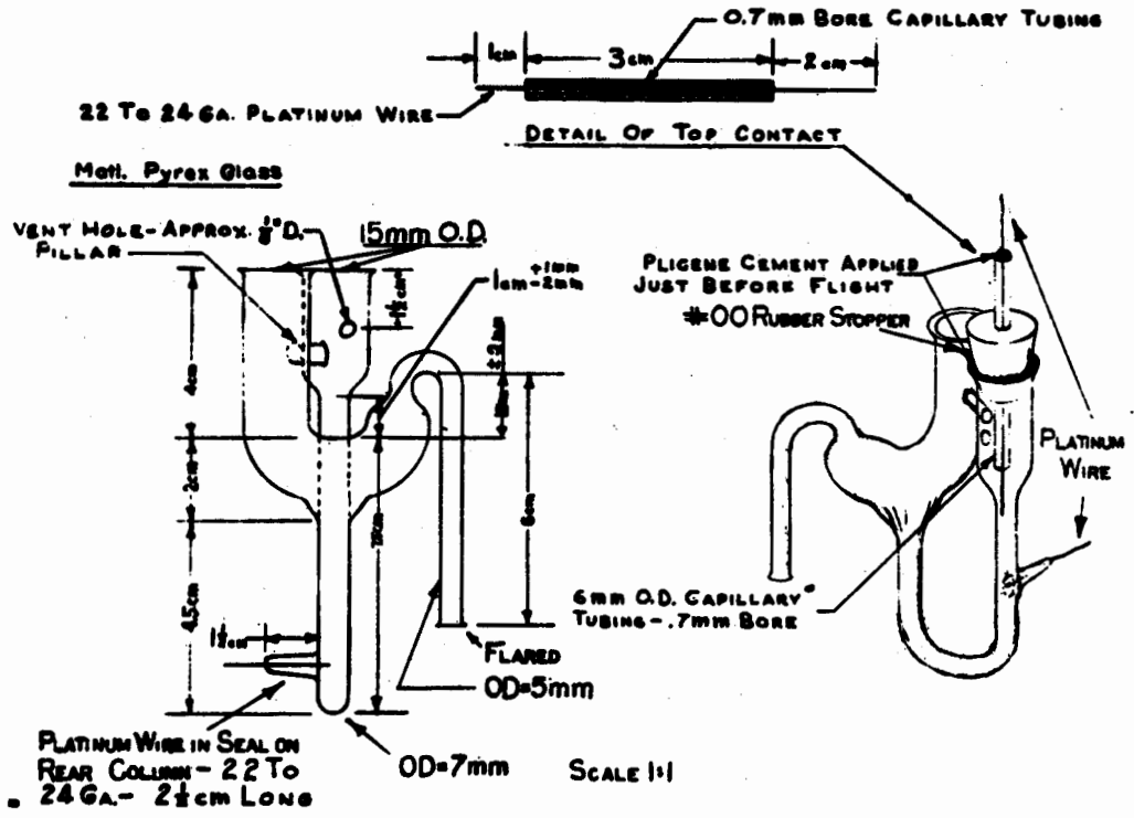
Figure 37. Automatic siphon.
