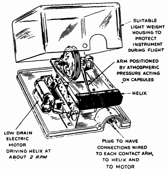
FIG. 5. Olland-cycle pressure modulator.
