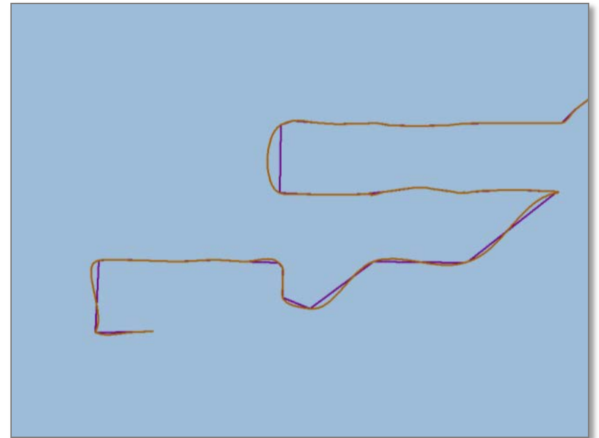
BEZIER Interpolation
