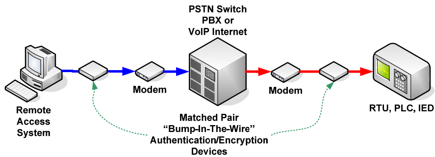
Figure 4. Bump-in-the-wire installation.
