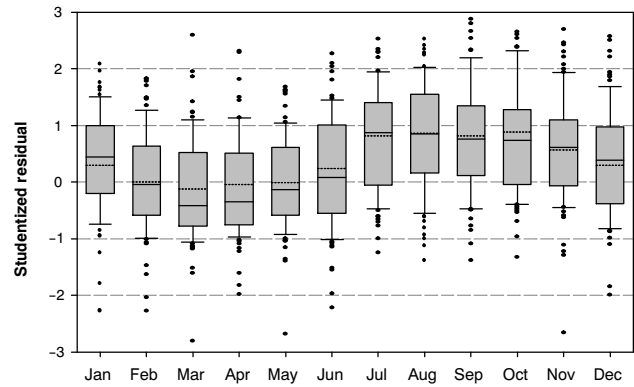
Figure 7. Seasonal distribution of Studentized residuals. Replicates are years and HUC8 watersheds. The box encloses the inter-quartile range, including horizontal lines for the mean (dotted) and median (solid). Whiskers indicate the 10th and 90th percentiles, and values outside this range are shown individually as points.
