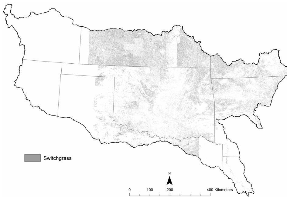
Figure 9. Preliminary estimates of agricultural areas where cultivation of switchgrass may become economically feasible by 2030 in the Arkansas-White-Red River basin.
