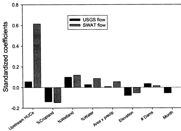
Figure 8. Comparison of influences on estimated monthly flows at HUC8 outlets (USGS flow) and those predicted by the SWAT model.
