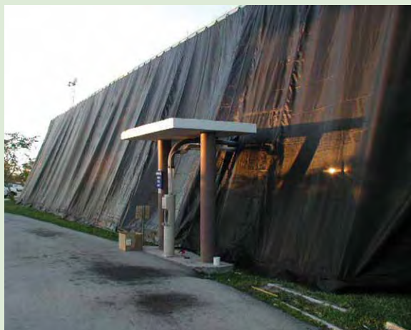
Figure 4-23. Hurricane screen, mesh, or fabric consists of woven polypropylene, which is a plastic polymer. The screen can cover large areas and provide protection to windows with unusual configurations. Light can pass through the fabric so that the area inside is not totally dark. Photo courtesy of the Department of Emergency Management, City and County of Honolulu.
