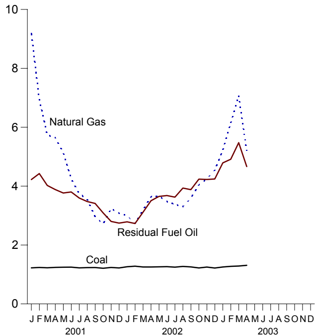
Figure 9.3 Cost of Fossil-Fuel Receipts at Electric Generating Plants (Dollars per Million Btu )
