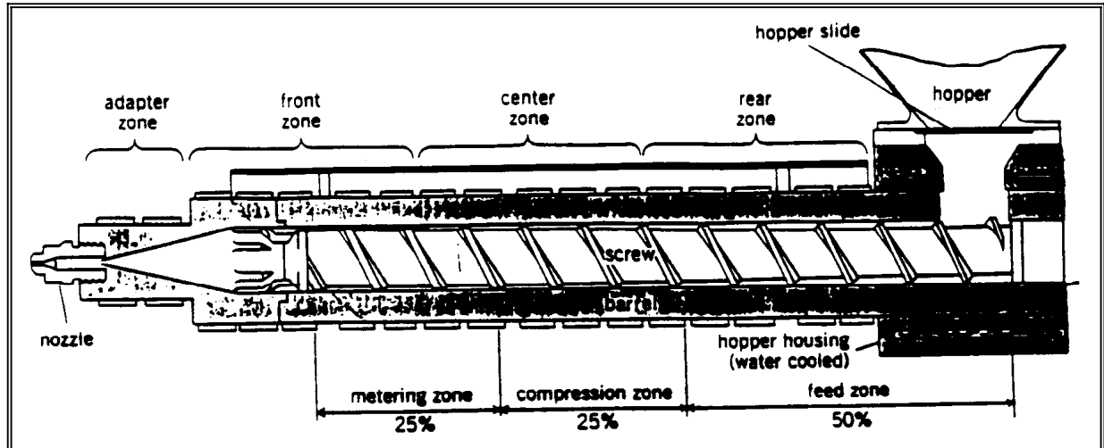
Figure 8: Injection Molding
