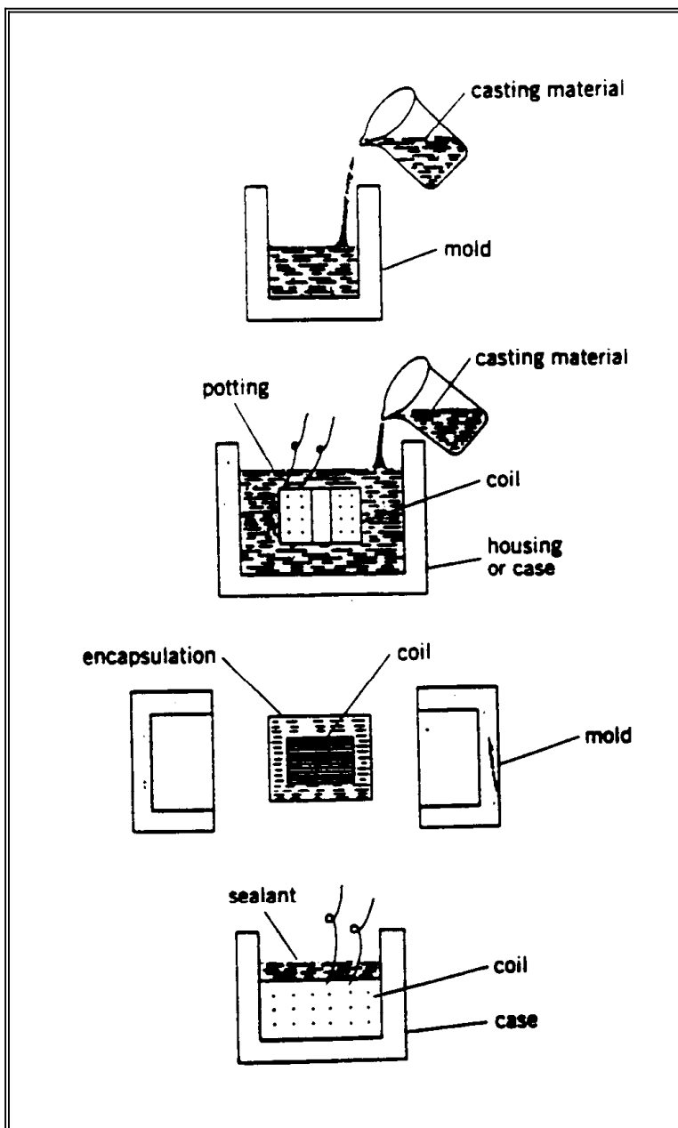
Figure 12: Encapsulation
