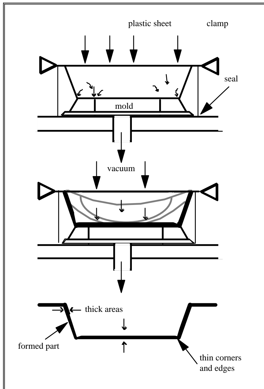
Figure 10: Thermoforming
