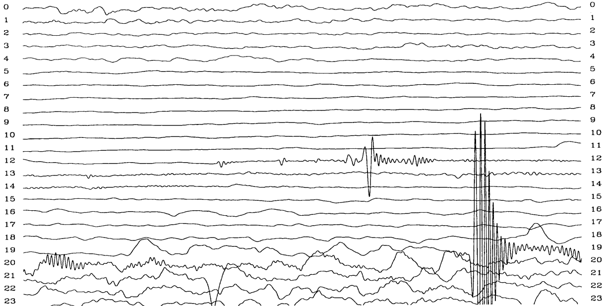
Figure 3.2 Time record for day 178 from the STS-1 horizontal sensor installed on a glass plate cemented to the floor under a sealed glass bell jar. The last four hours of the record contain data during a windy time period
