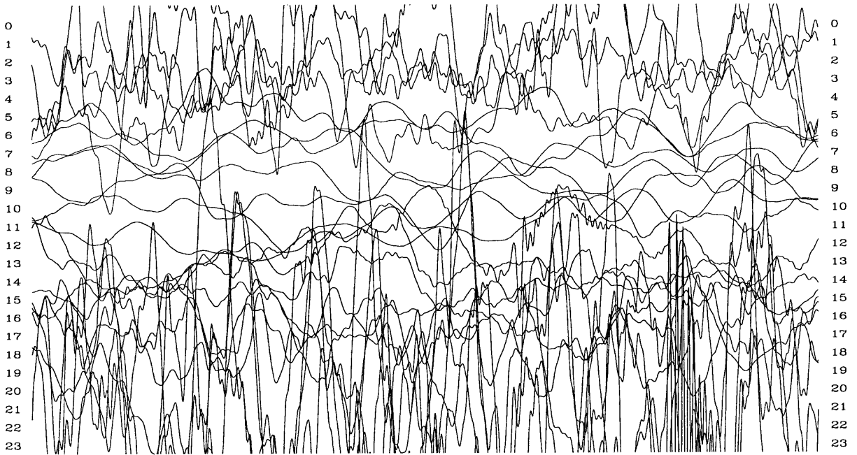
Figure 3.1 Time record for day 178 from the STS-1 horizontal sensor installed on a glass plate resting on sand under a sealed plastic bell jar. The last four hours of the record contain data during a windy time period.
