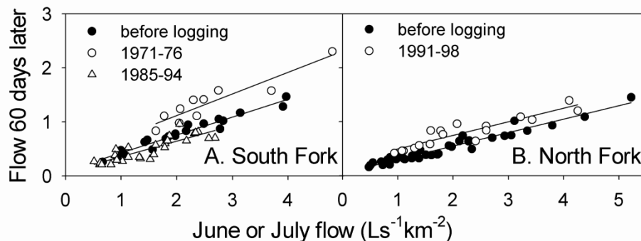
Figure 4 —Comparison of early and late dry-season flows before and after logging at the A. South Fork and B. North Fork Caspar Creek weirs.
