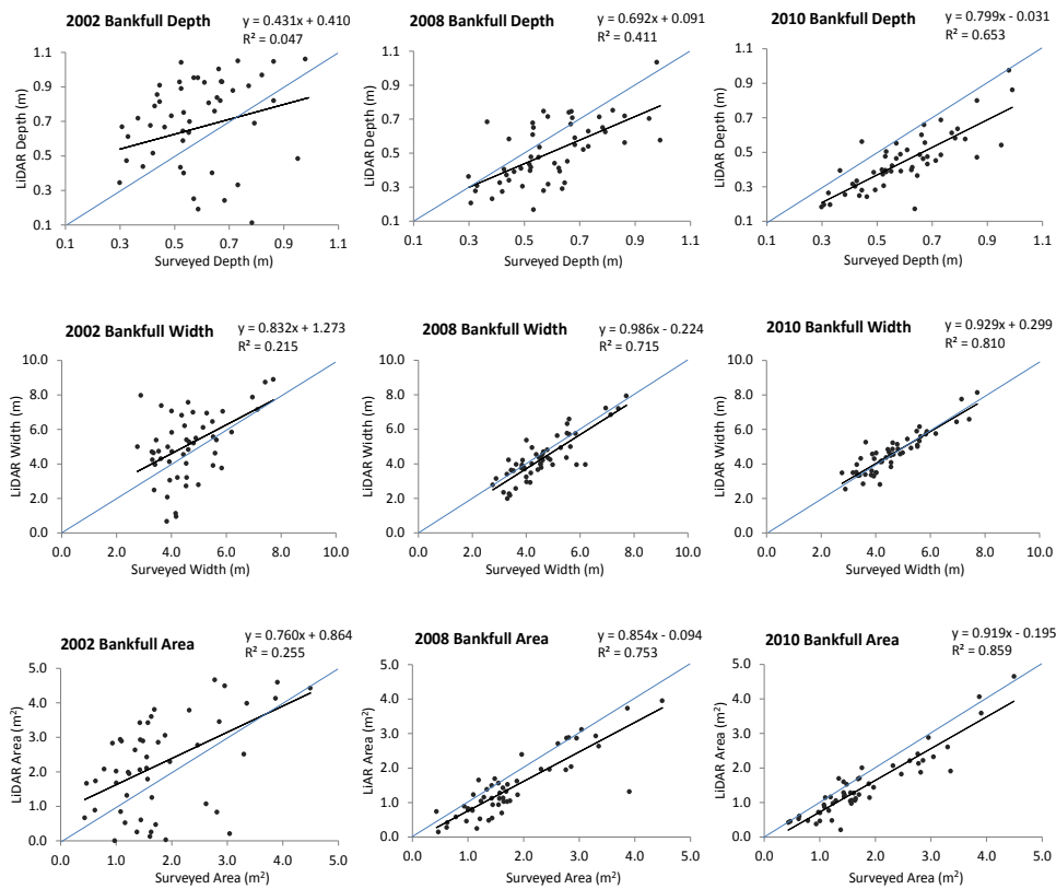
Figure 3 —Scatterplots showing LiDAR- and field-surveyed channel features (bankfull depth, width, and area) from 2002, 2008, and 2010 data. A 1:1 line is drawn for reference.
