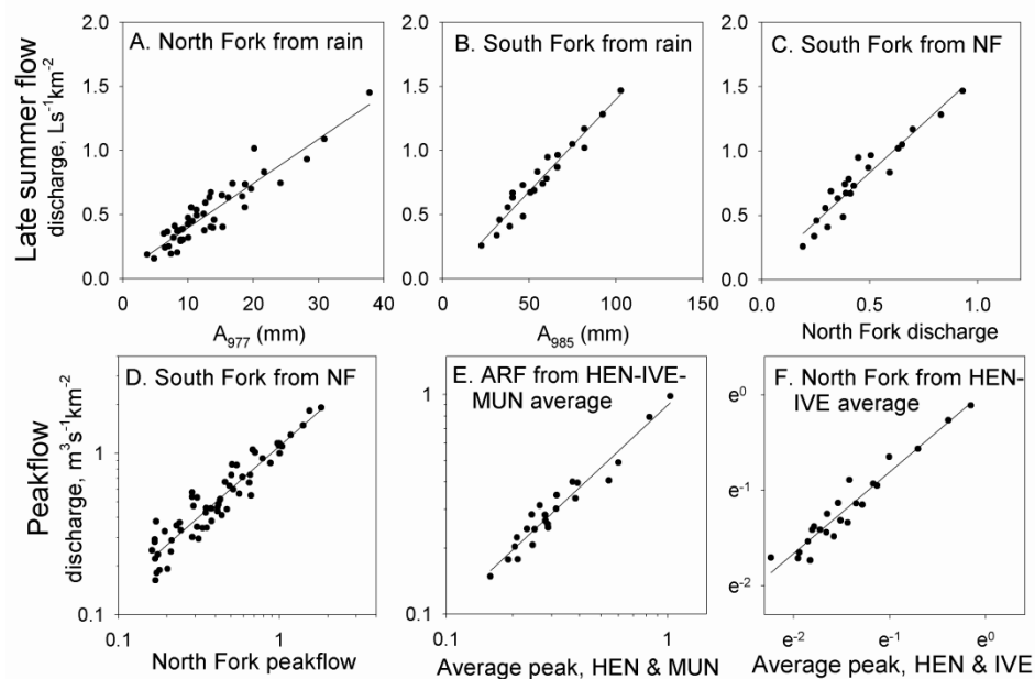
Figure 2 —Calibrations between A. North Fork late-summer flows and API_{977} ; B. South Fork late-summer flows and API_{985} ; C. South Fork late-summer flows and those observed at the North Fork; D. South Fork and North Fork peakflows; E. ARF peakflows and the average of those at HEN, IVE, and MUN; and F. North Fork peakflows and the average of those at HEN and IVE.
