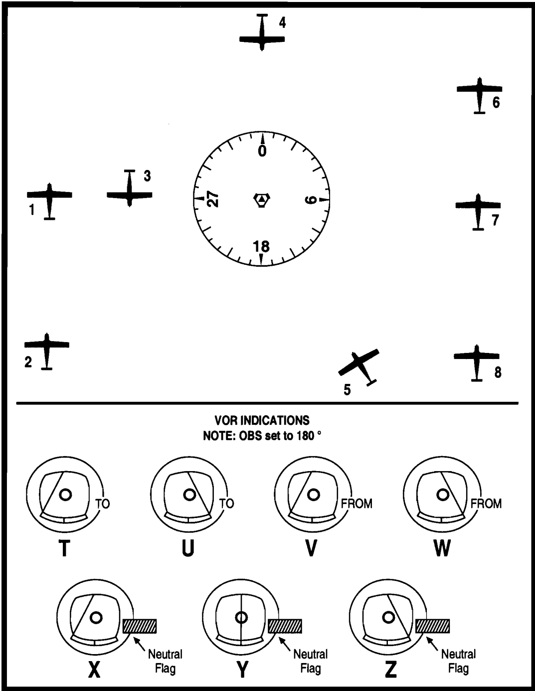
FIGURE 42.—VOR Indications.
