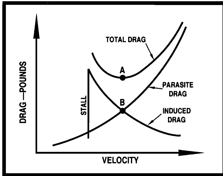
FIGURE 20.—Drag Chart.
