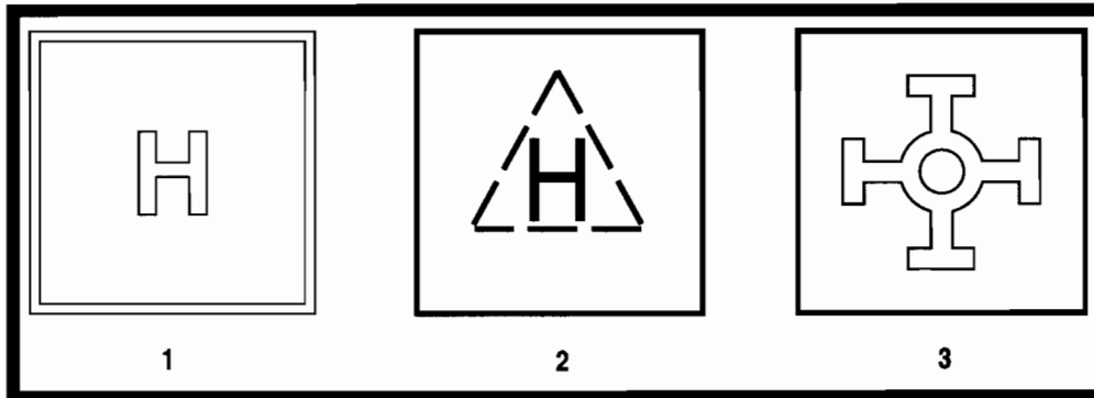
FIGURE 53.—Heliport Markings.
