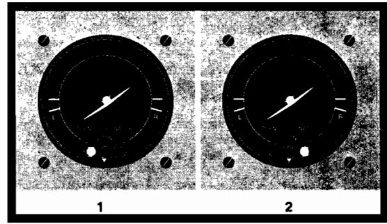
FIGURE 52.—Turn-and-Slip Indicators.
