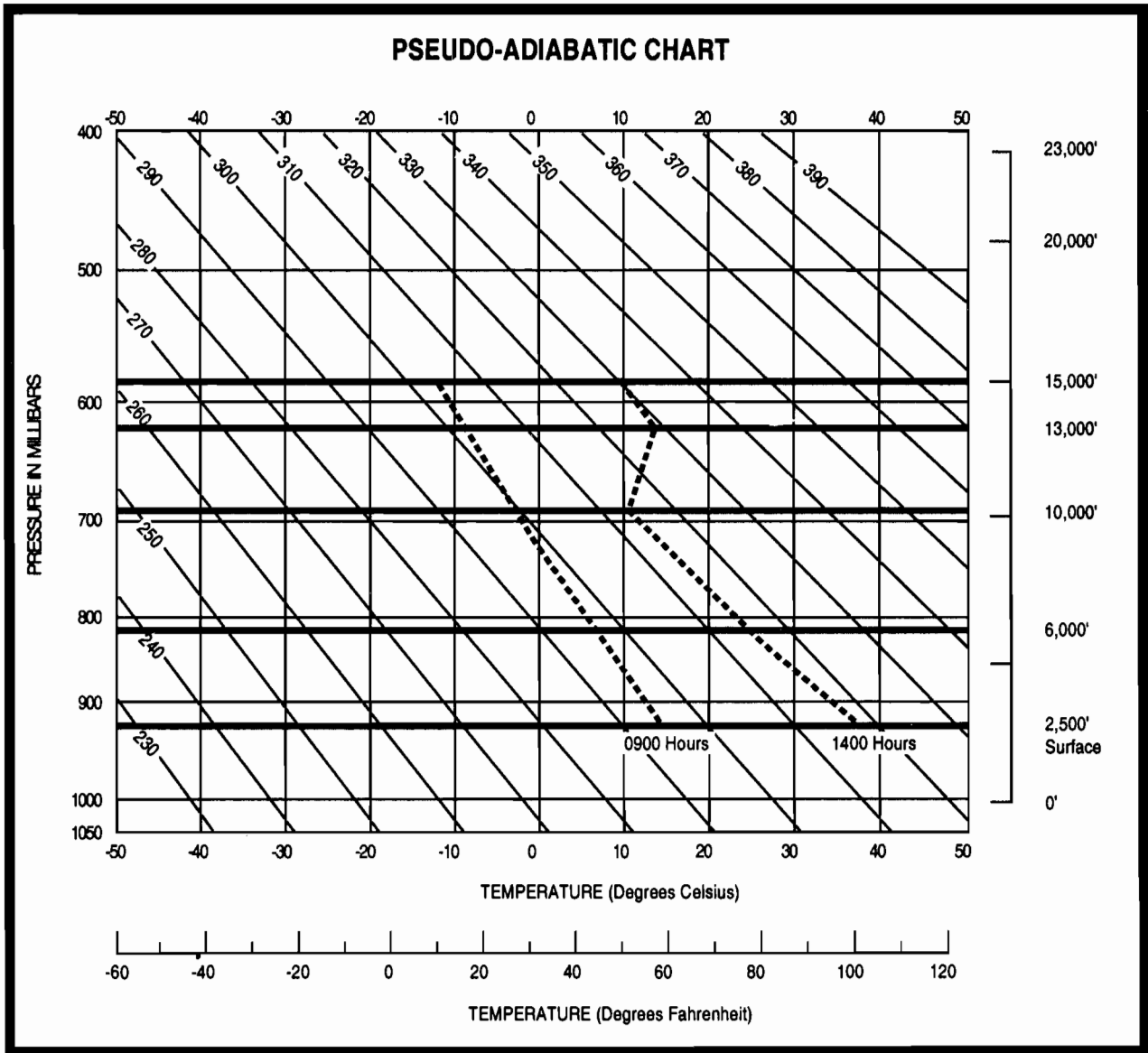
FIGURE 2.—Pseudo-Adiabatic Chart.
