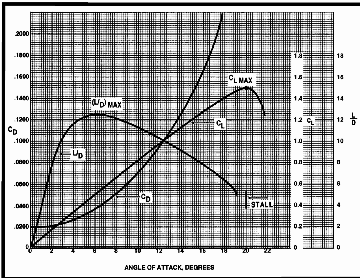
FIGURE 19.—Angle-of-Attack Chart.
