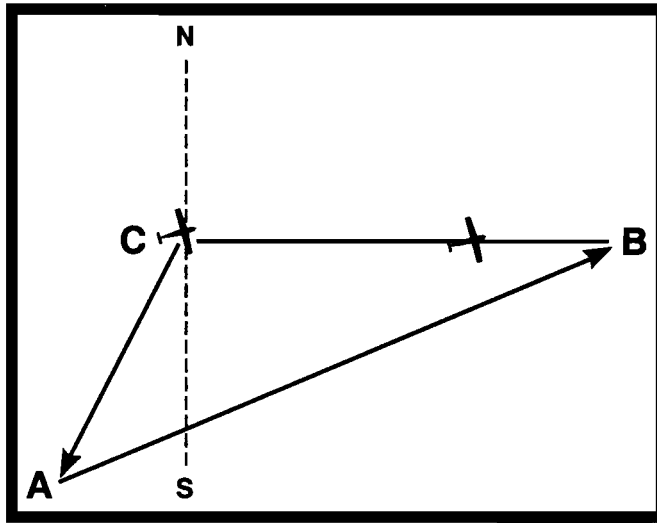
FIGURE 40.—Wind Triangle.
