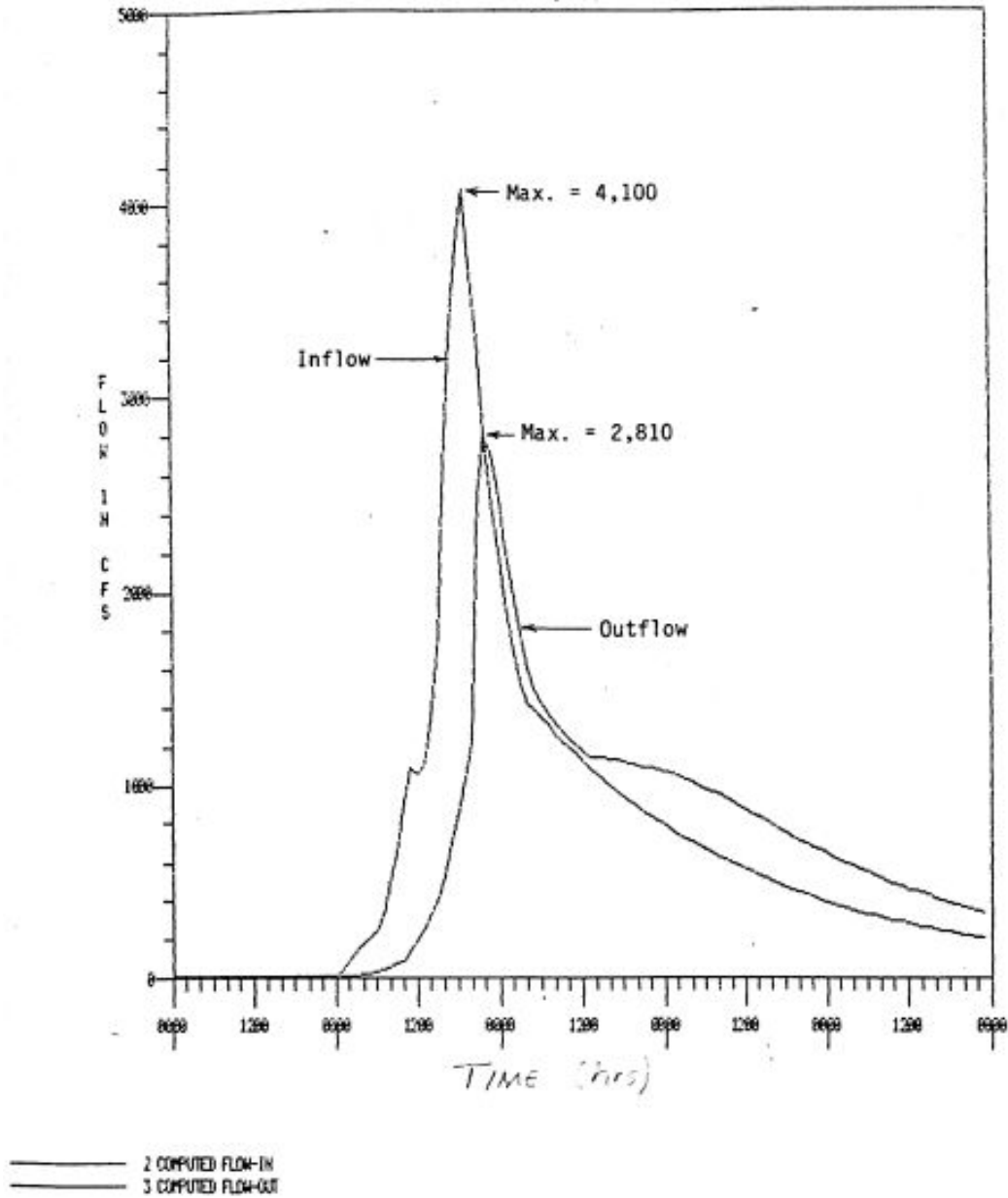
Inflow/Outflow Hydrograph for General Storm PMF SAMPLE PROJECT
