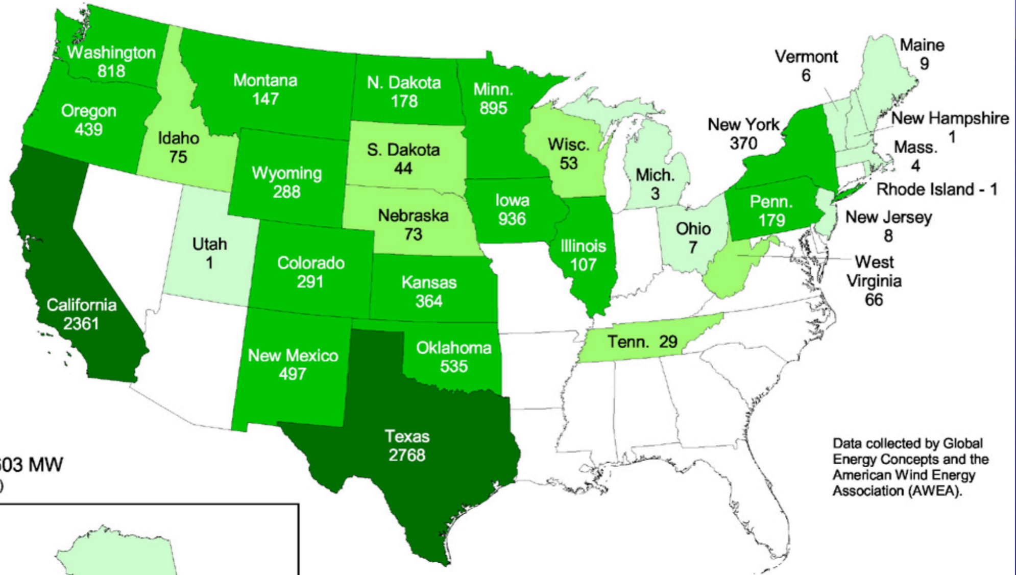
2006 Year End Wind Power Capacity (MW)
