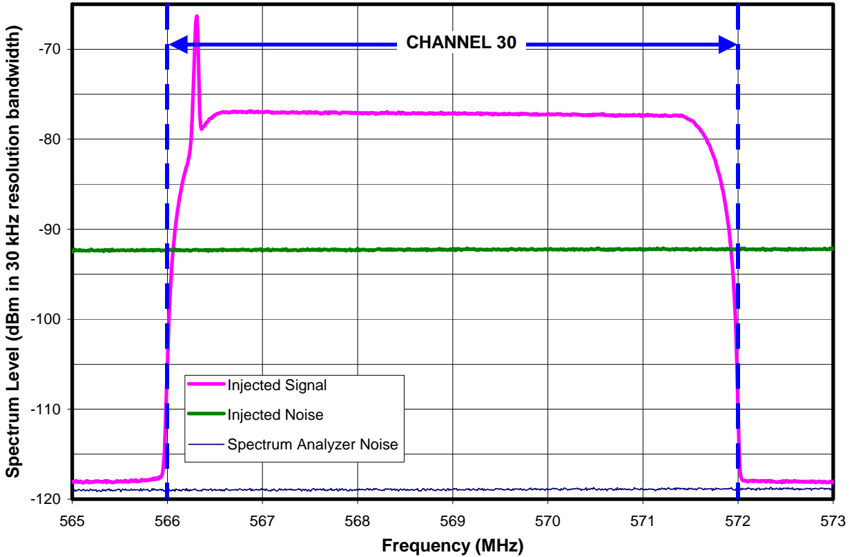
Figure A-6. Spectra of Injected Signal and Noise at 15-dB CNR
