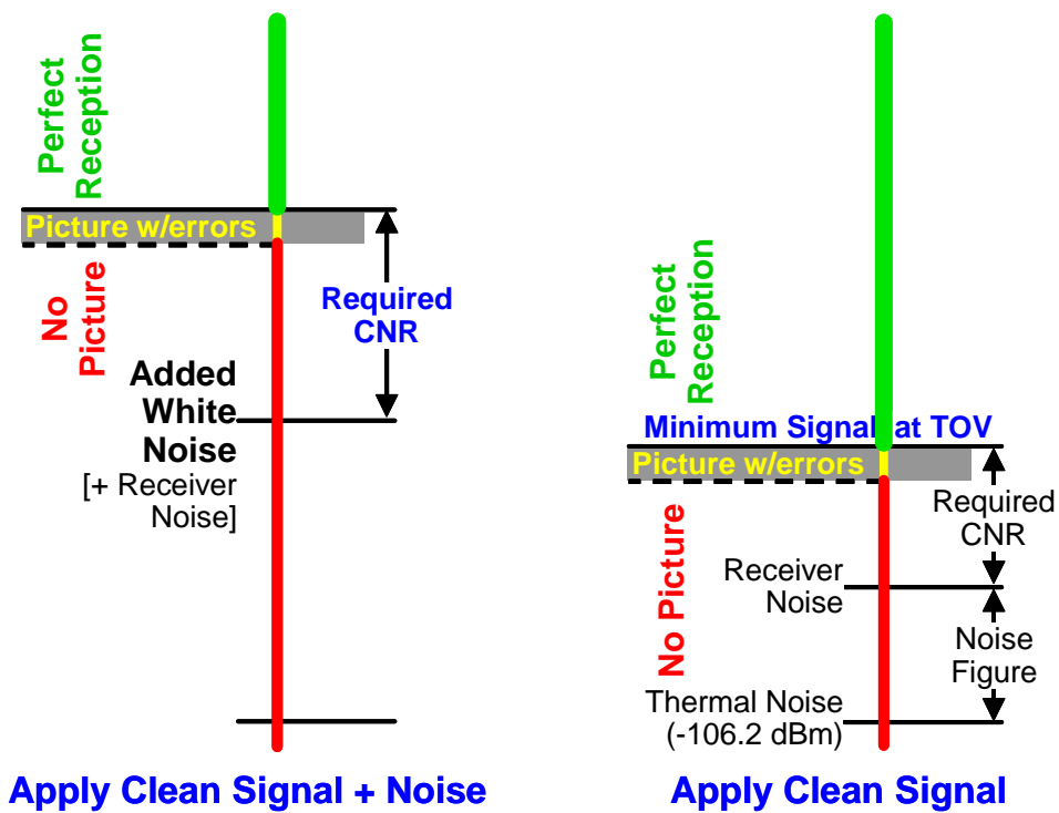
Figure 5-1. Relationship between Minimum Signal at TOV and Required CNR
