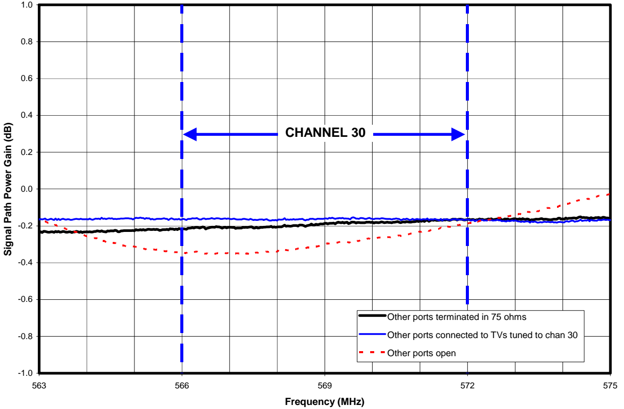
Figure A-4. Effect of Load Impedance Mismatch
