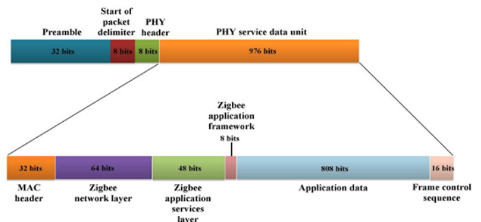
Figure 2. Anatomy of the simulated 1024-bit Zigbee data packets, based on [12]
