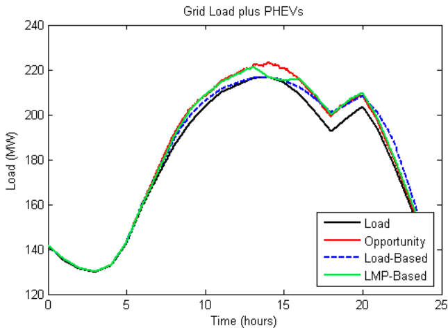
Figure 6. Utility load curve for April 11, 2005, assuming a 5% PHEV adoption rate. Opportunity, load-, and LMP-based charging load profiles are plotted on top of the existing load.
