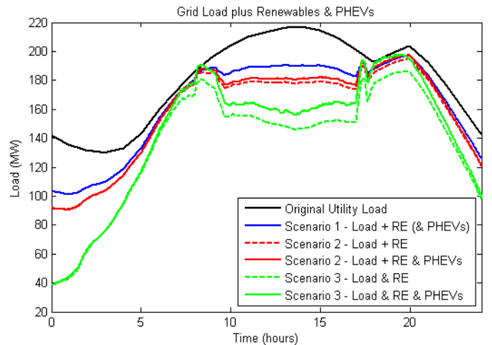
Figure 8. Scenario 3: Utility load curve, including renewable power generation and PHEV loads.
