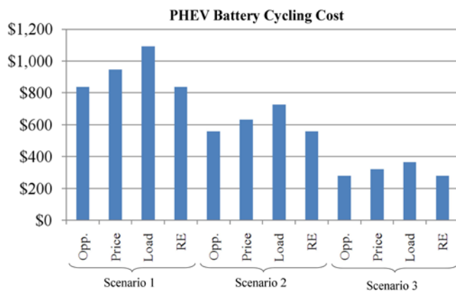
Figure 4. Battery wear cost for 12 scenarios
