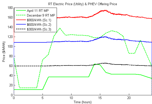
Figure 5. Real-time utility prices and PHEV fleet V2G offering prices, using the price-based algorithm
