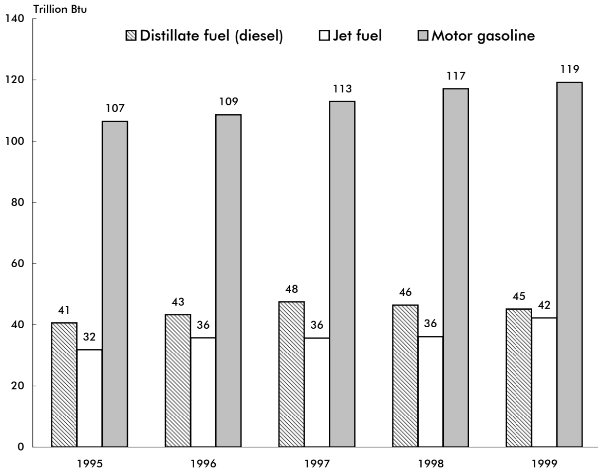
Figure 7-2: Utah Transportation Energy Consumption
