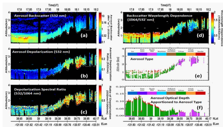
Fig. 22. (a) Aerosol backscatter (532 nm), (b) aerosol depolarization (532 nm), (c) ratio of aerosol depolarization (532/1064 nm), (d) backscatter wavelength dependence ((1064/532 nm) measured by the airborne HSRL between 17:45–18:12 UT on 19 June. This portion of the B200 flight covered about 160 km between the Sacramento area (left) and the mountains east of Sacramento (right). The dark area in the bottom part of the images represents the ground surface. (e) aerosol type inferred from the HSRL measurements of aerosol intensive parameters. (f) AOD apportioned to aerosol type.
