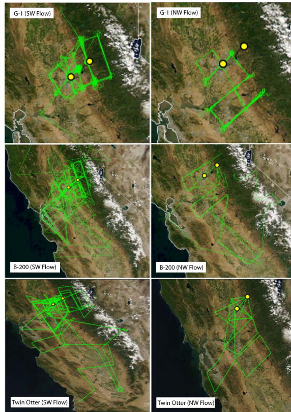
Fig. 4. DOE G-1, NASA B-200, and NOAA Twin Otter Flight Tracks during the SW and NW flow periods.
