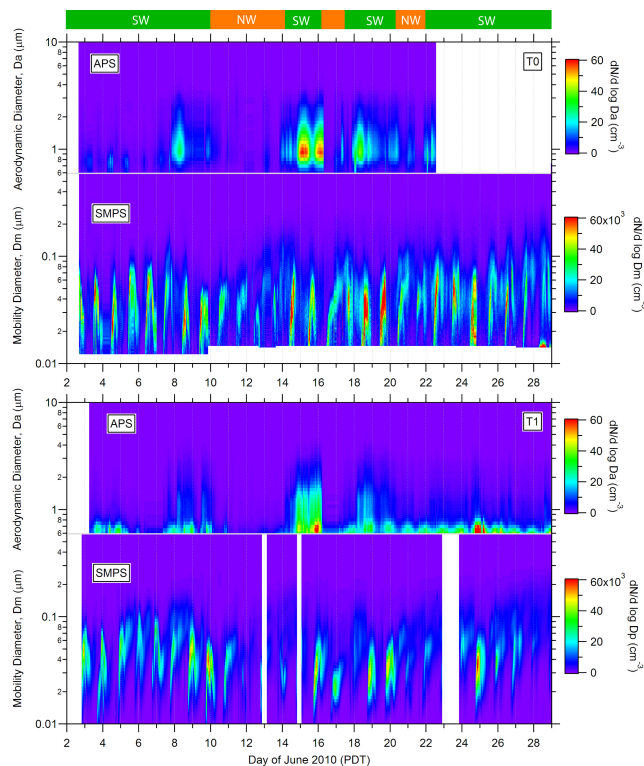
Fig. 11. Comparison of aerosol number size distributions at T0 and T1 sites. Note that the color scales for APS and SMPS distributions differ by three orders of magnitude.
