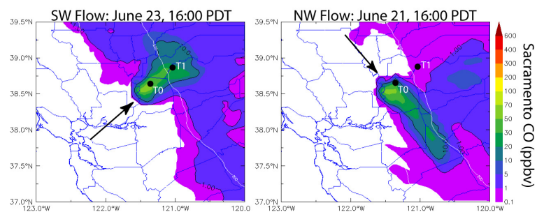
Fig. 3. Examples of tracer forecasts, based on CO emitted from Sacramento, shown at 16:00 PDT under southwesterly (left panel) and northwesterly wind (right panel) flow conditions.
