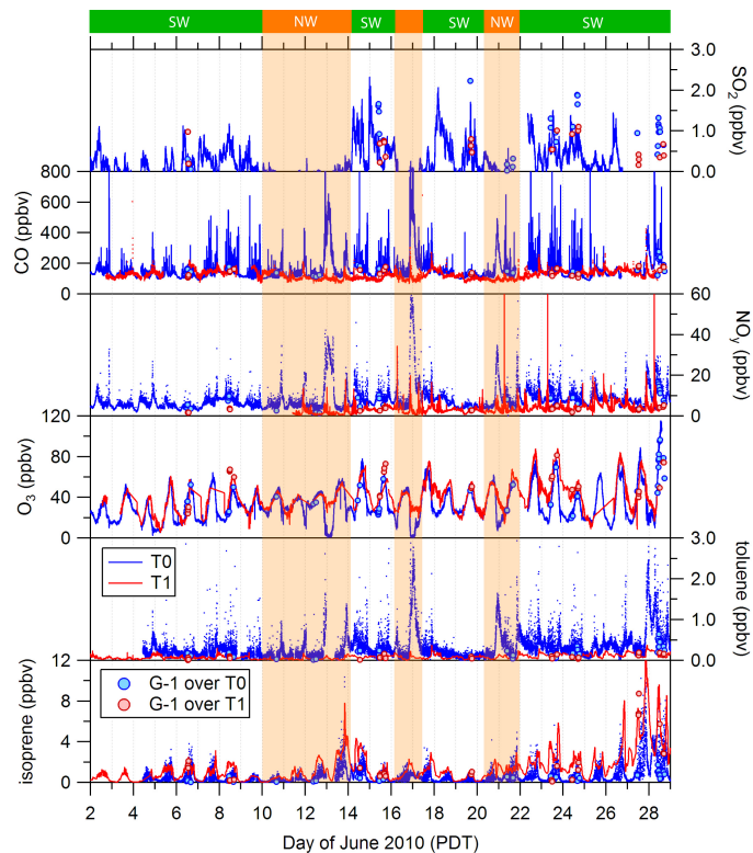
Fig. 6. Comparison of trace gases time series at T0 and T1 ground sites along with observations onboard the G-1 during overpasses at the respective sites. The NO y instrument at the T1 site did not operate until 11 June and the SO 2 instrument at the T0 site did not operate on 27–28 June.
