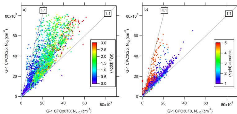
Fig. 10. Scatter plots of CPC-3025 vs. CPC-3010 number concentrations observed on the G-1: (a) the points are colored by the corresponding \text{SO}_2 mixing ratios; (b) the points are colored by the corresponding isoprene mixing ratios (points with isoprene mixing ratios < 1 ppbv were removed from the plot for clarity). Grey lines show slopes of 4:1 and 1:1.
