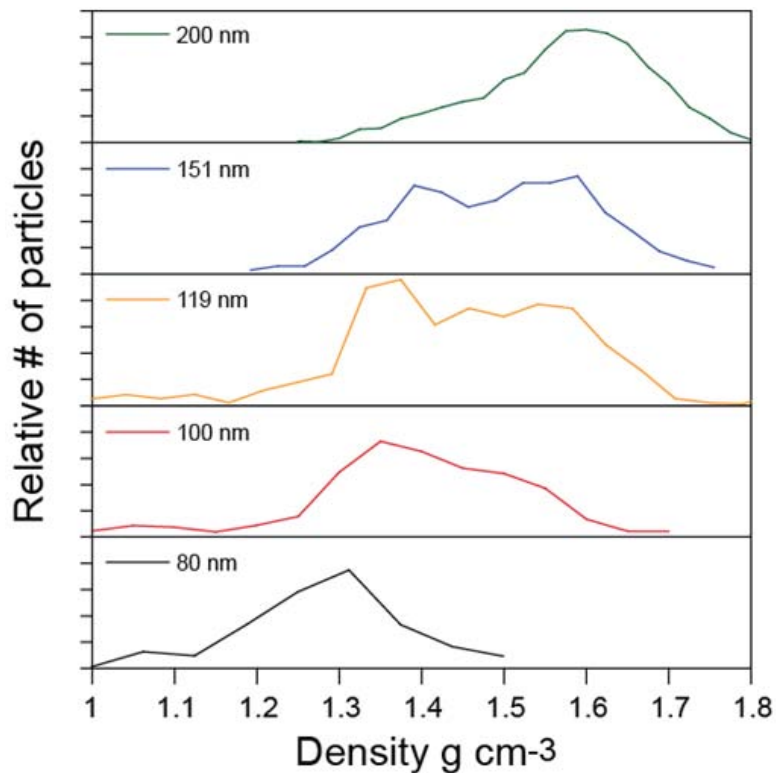
Fig. 14. Size-dependent particle densities as measured by SPLAT II on 6 June at 10:00 a.m.
