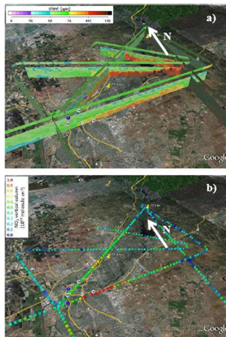
Fig. 25. (a) Ozone mixing ratio profiles measured with the TOPAZ lidar and (b) \text{NO}_2 vertical column densities measured with the CU AMAX DOAS system over the Sacramento area on 28 June. Data are from two flight segments from 11:28–12:03 and 13:04–13:52 PDT. The ozone profiles extend from near the ground to 1500 m MSL. The colored line above the ozone “curtain” plot represents the ozone in situ measurements at flight level (approx. 2100 m MSL). The locations of the T0 and T1 ground sites are indicated by yellow pushpin markers.
