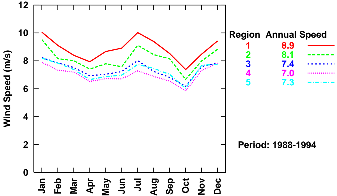
Dominican Republic Satellite-based Ocean Wind Speeds
