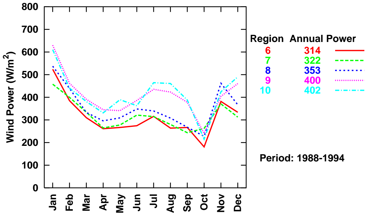
Dominican Republic Satellite-based Ocean Wind Power Densities
