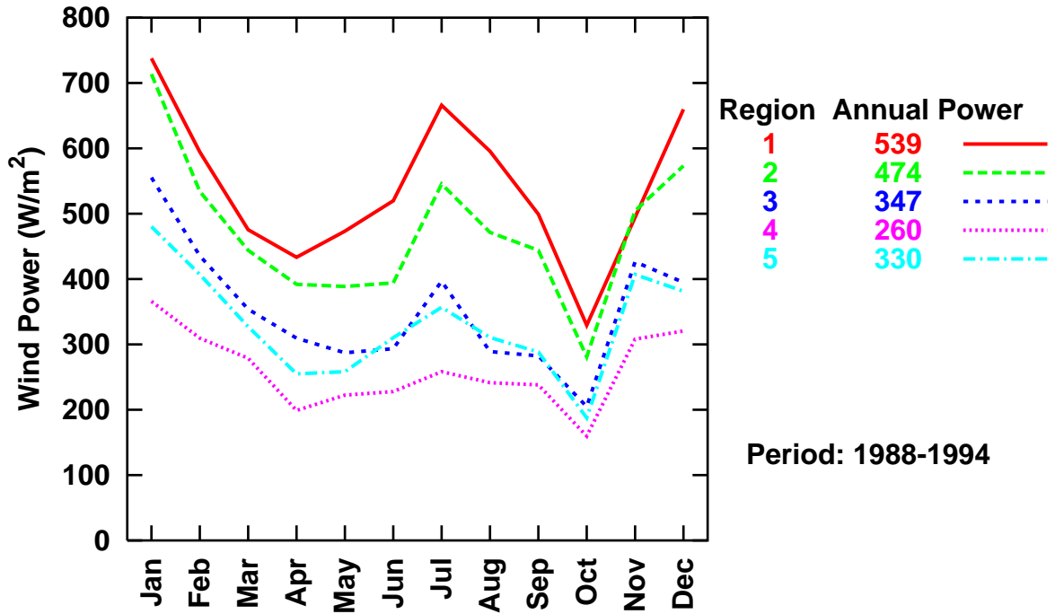
Dominican Republic Satellite-based Ocean Wind Power Densities
