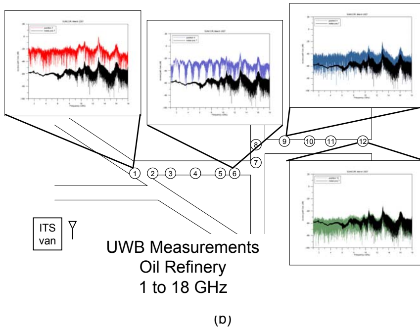
Figure 7.2-9: Summary of the excess-path-loss measurements in the oil refinery. Carrier frequencies from (a) 25 MHz to 1.2 GHz and (b) 1 GHz to 18 GHz.
