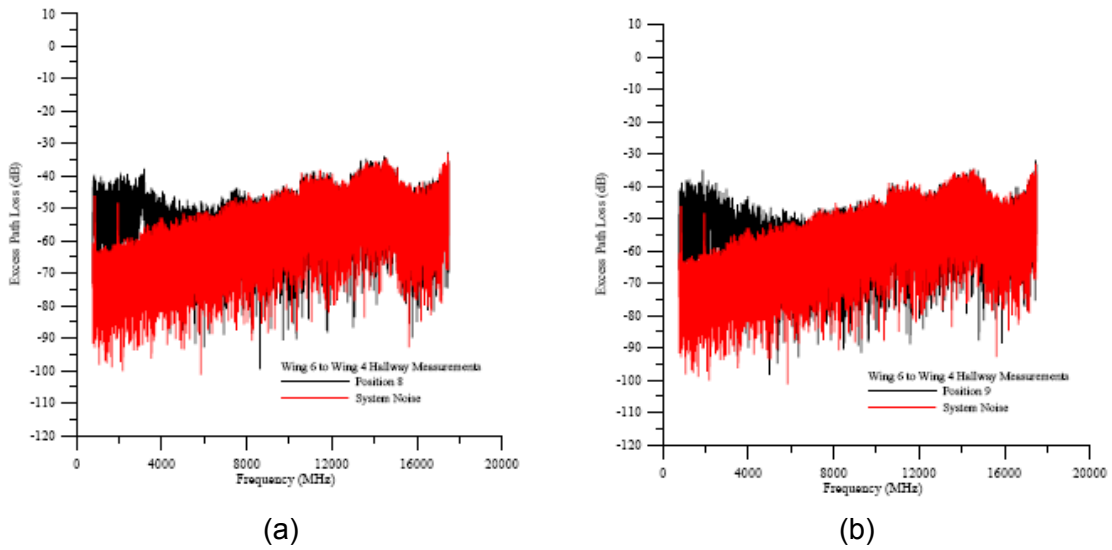
Figure 4.3-4: When the transmitting antenna was located outside the building, there was little change in the excess path loss as the receiving antenna moved from position 8 in the junction (a) to position 9 around the corner (b). The overall signal level was lower than for the case where the transmitting antenna was inside the building. Most of the high-frequency signals were below the noise floor of the measurement system.
