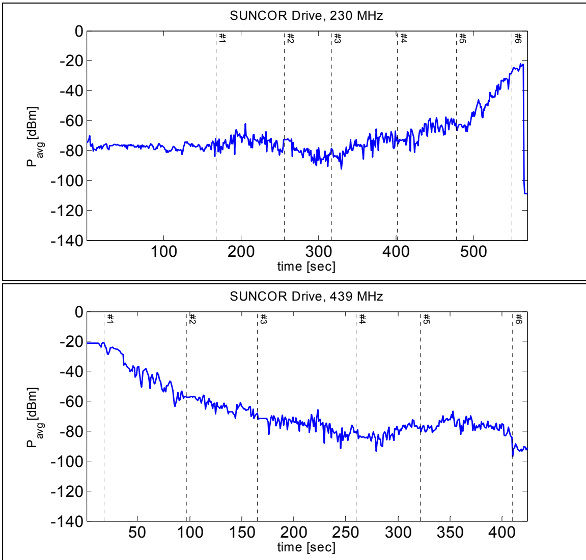
Figure C.5: Received-power data for carrier frequencies of 230 MHz (top) and 439 MHz (bottom). The path covered a drive around the perimeter of the refinery. The top figure was in one direction and the bottom figure was in the opposite direction.
