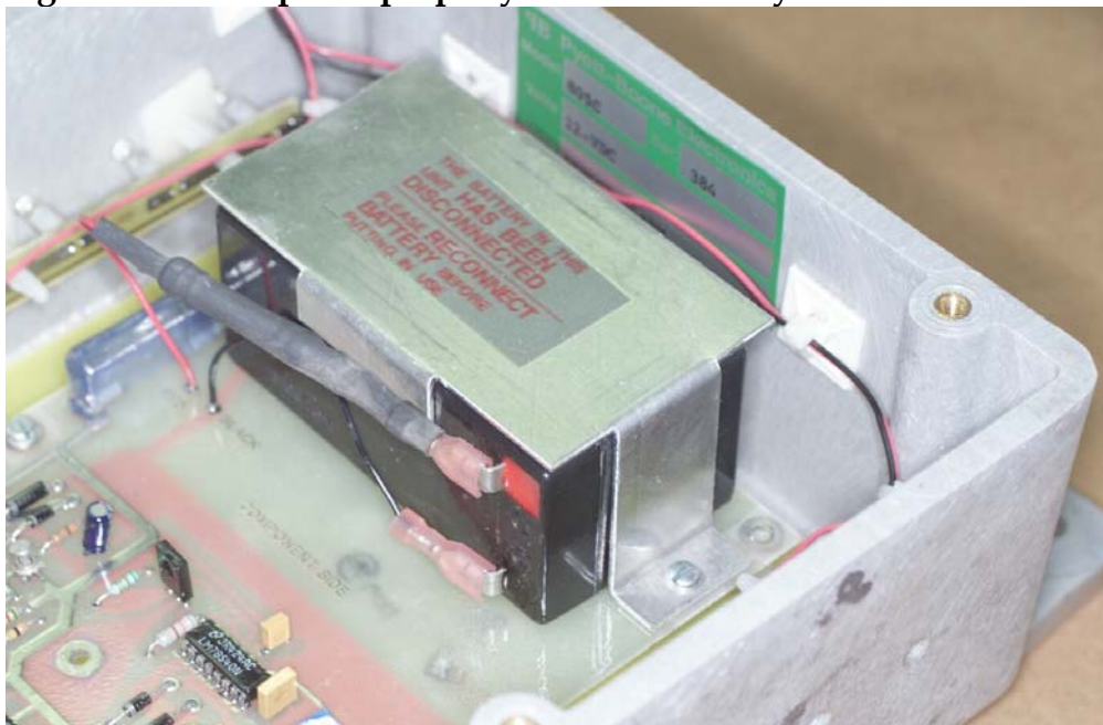
Figure 13 - Example of properly installed battery.
