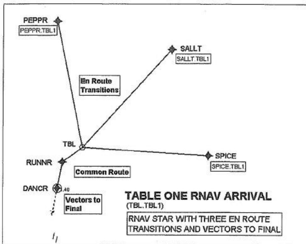
FIG 1 RNAV STAR Example
