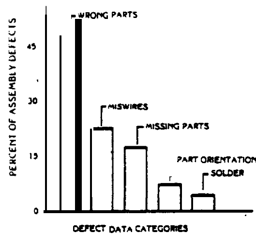
Figure 5-1. Assembly Defects
