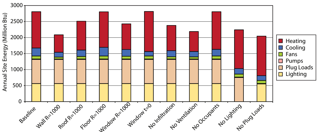
Figure F-8. Load Elimination Parametric Analysis for Annual Site Energy Use
