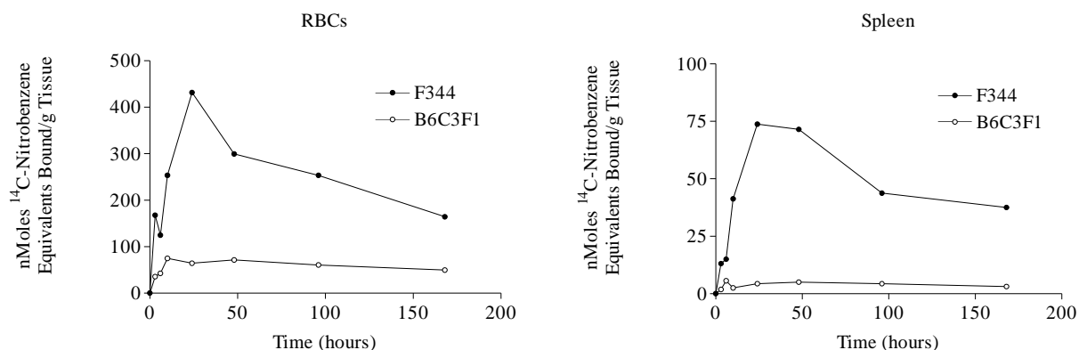
Figure 3-1. Time course of covalently bound [ ^{14}\text{C} ]-nitrobenzene in RBCs and spleen of rats and mice.
