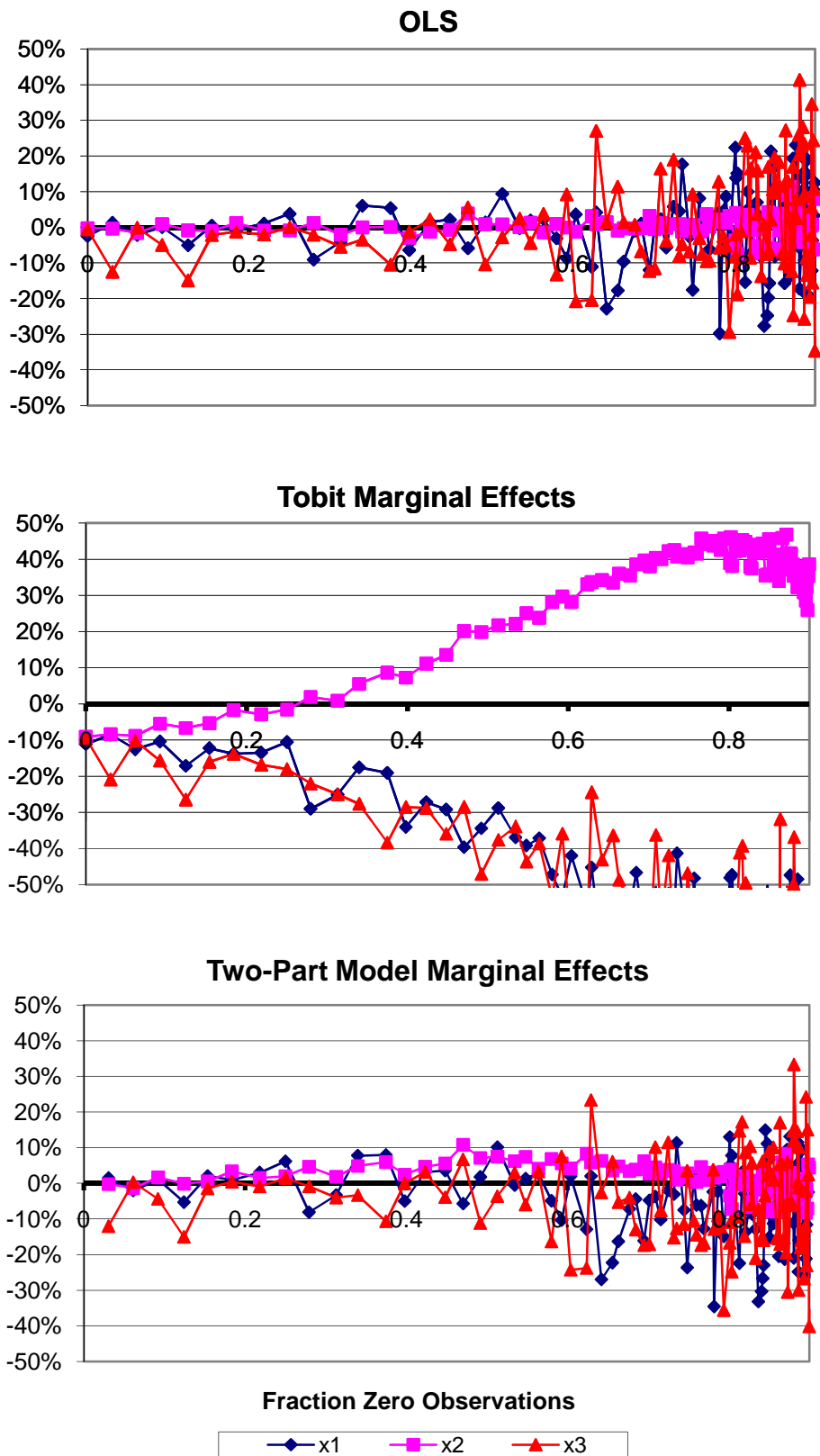
Figure 4: The Fraction of Zero Observations is Positively Related to x_2
