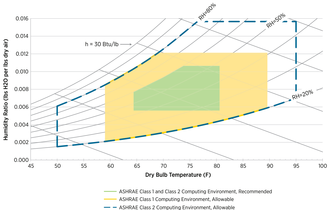
Figure 1. 2008 ASHRAE Allowable and Recommended Environment operating conditions for data centers.
