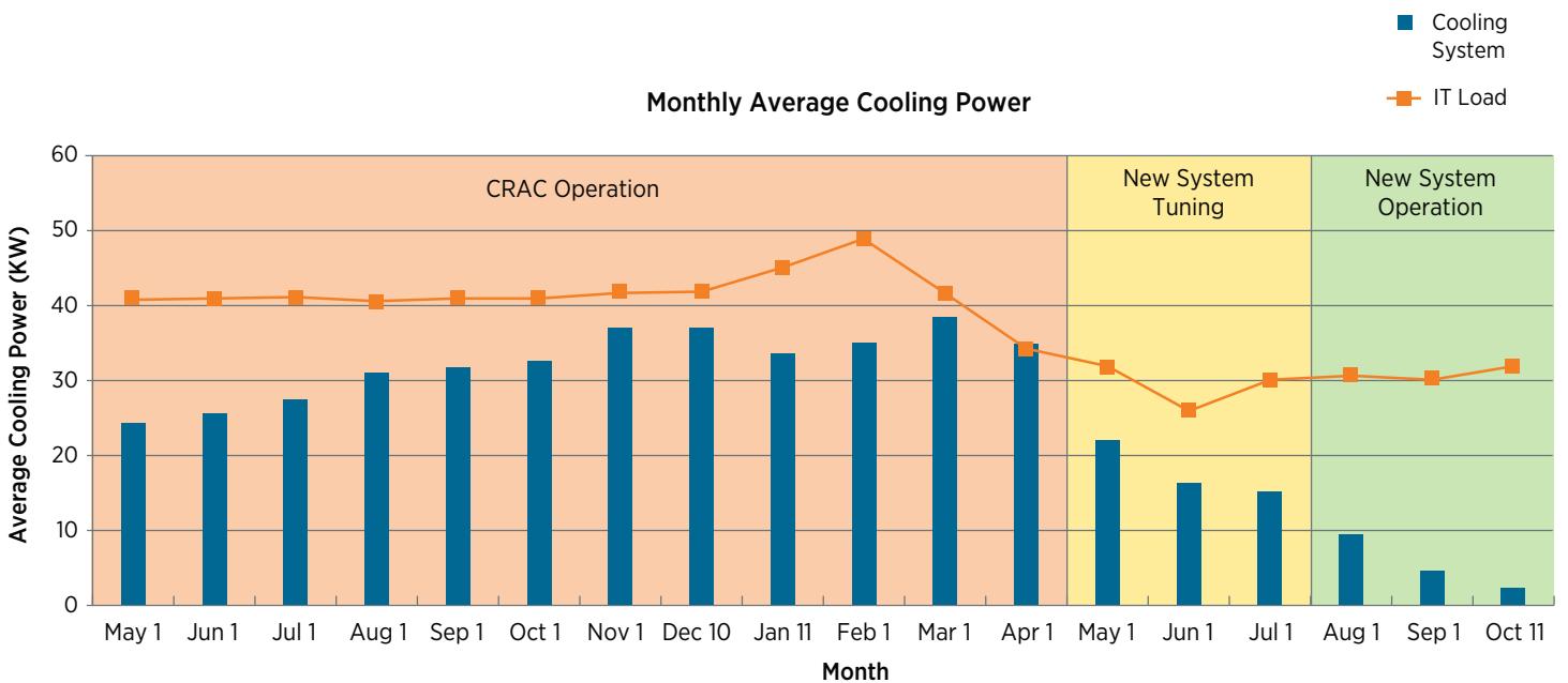
Figure 5. Monthly average cooling power comparison between CRAC system and new system.
