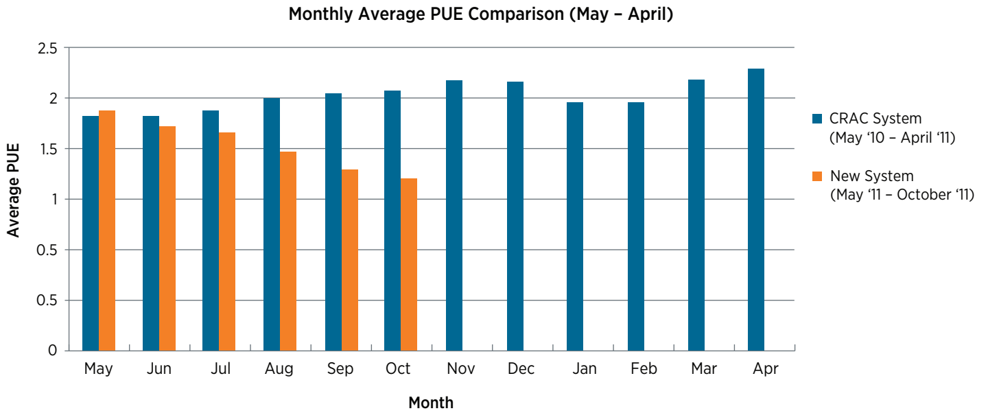
Figure 4. Monthly average PUE comparison.
