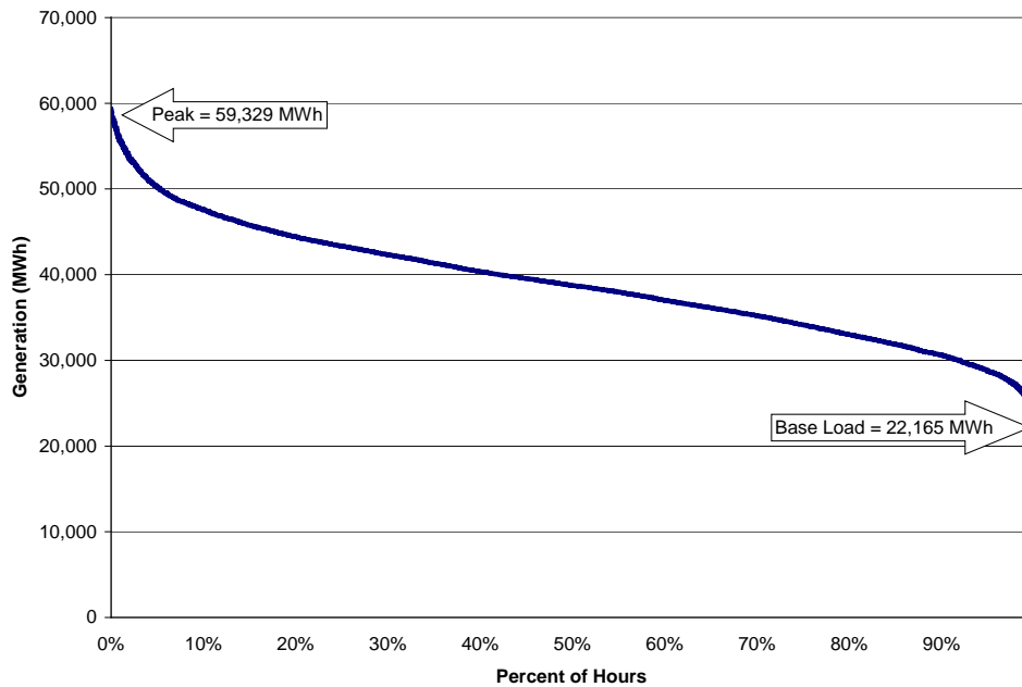
Figure 4-1. MAIN-MAPP 2000 Load Duration Curve
