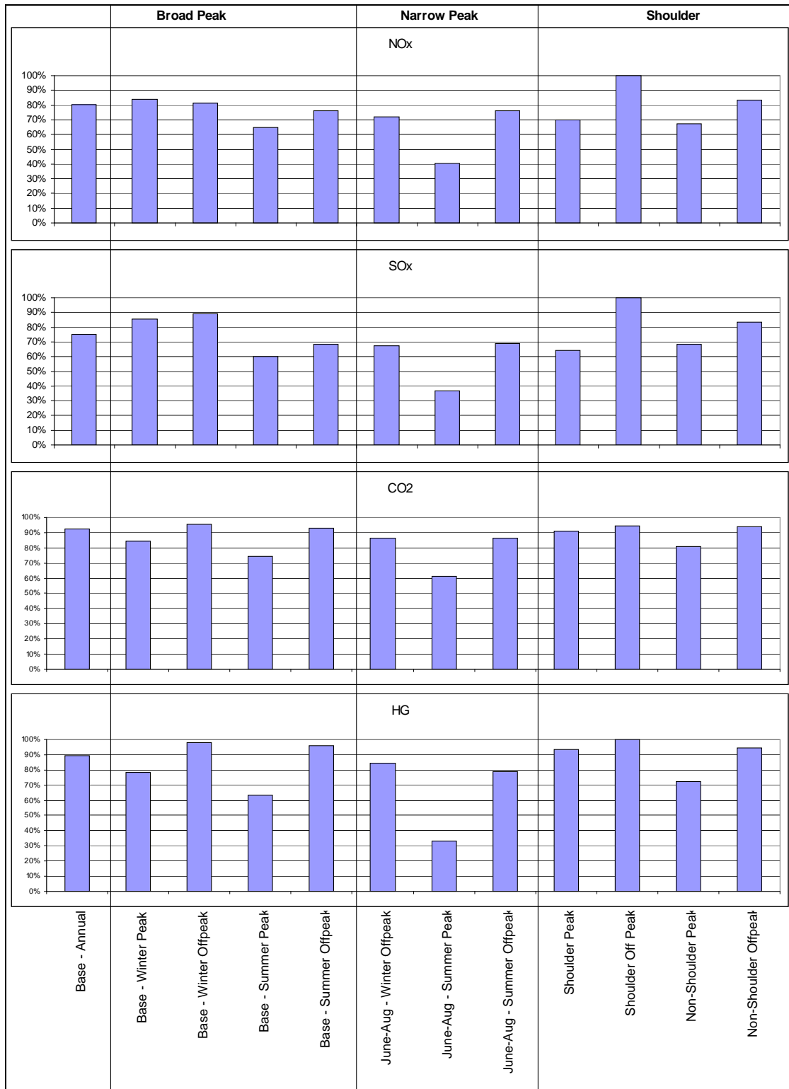
Figure 4-7. EMISSION RATES ACROSS THREE SCENARIOS (Percent of Maximum Emission Rate by Substance)
