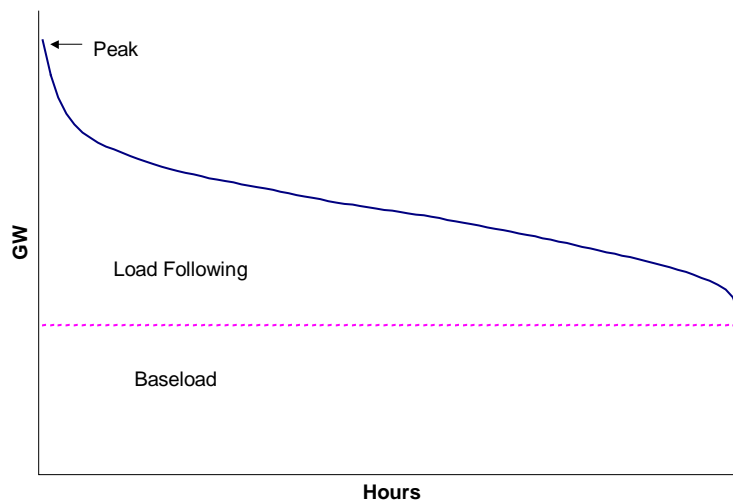
Figure 3-1. LOAD DURATION CURVE
