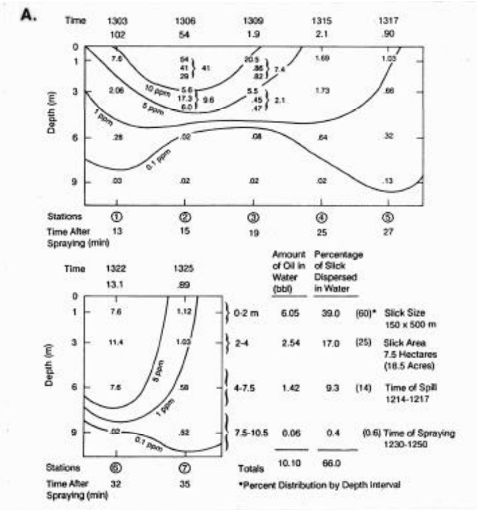
Figure 5-9. Results of water sampling at the California 1979 dispersed oil experiments, where 20 barrels of crude oil were treated (McAuliffe et al., 1981). A) Immediately after the application of dispersants, maximum concentrations in the top meter averaged 41 ppm.
