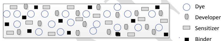
Figure 3-2: Elements of the Thermal Reactive Layer
