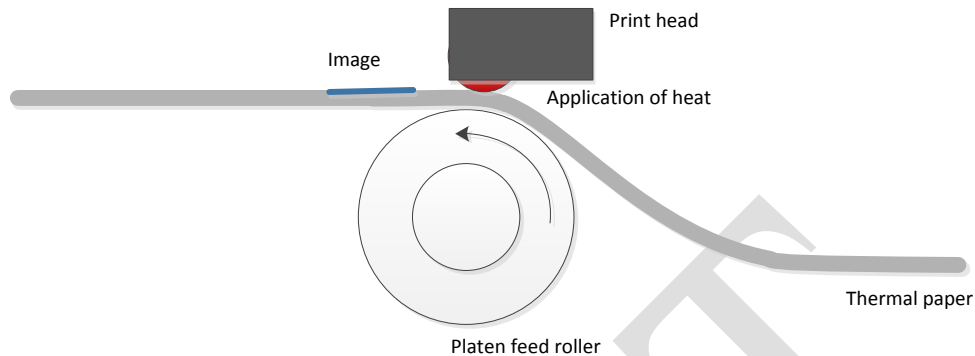
Figure 3-3: Overview of Thermal Printing Process (based on Koehler Thermal Paper n.d. and Charters Paper Pty Ltd 2006)
