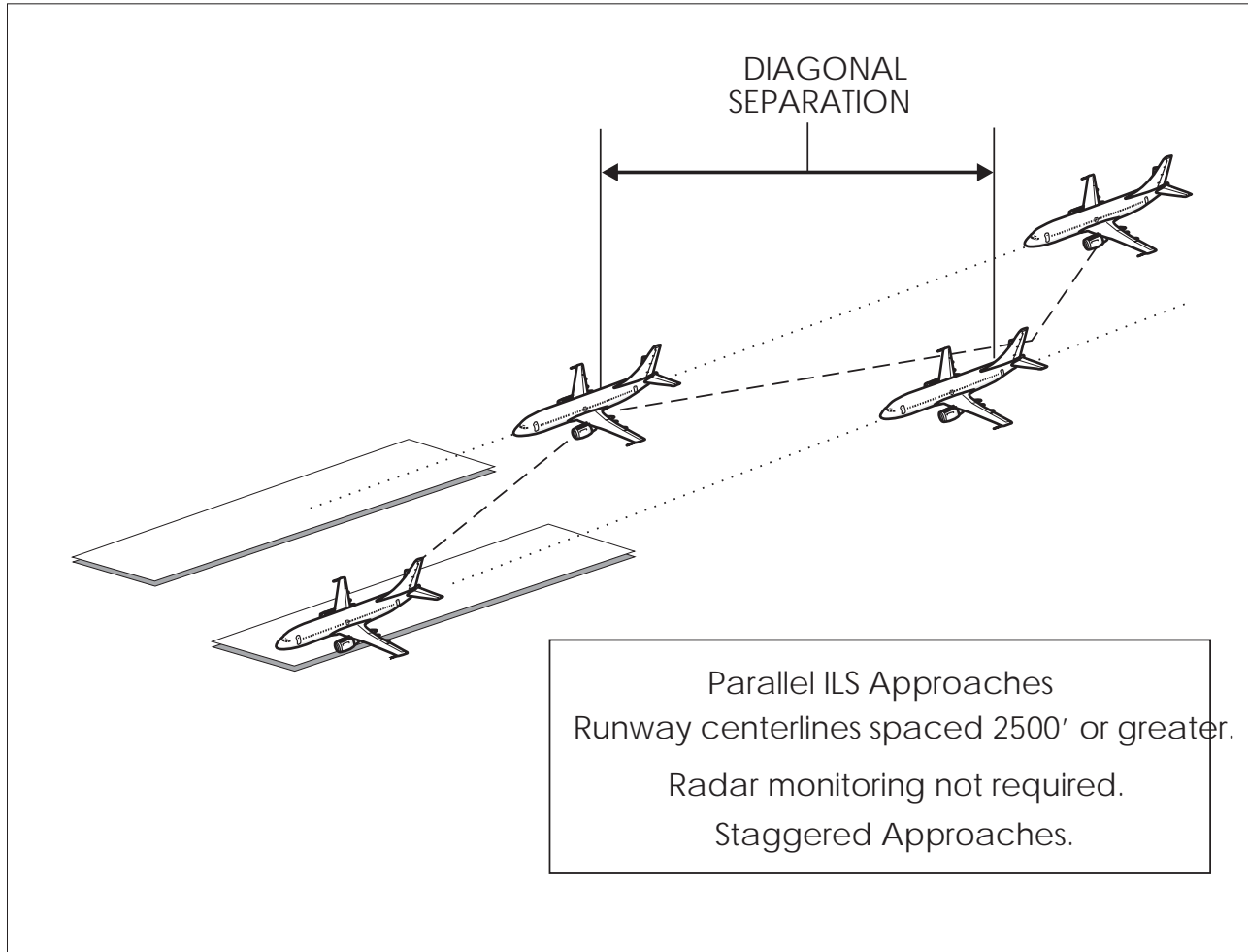
FIG ENR 1.5-29 Staggered ILS Approaches
