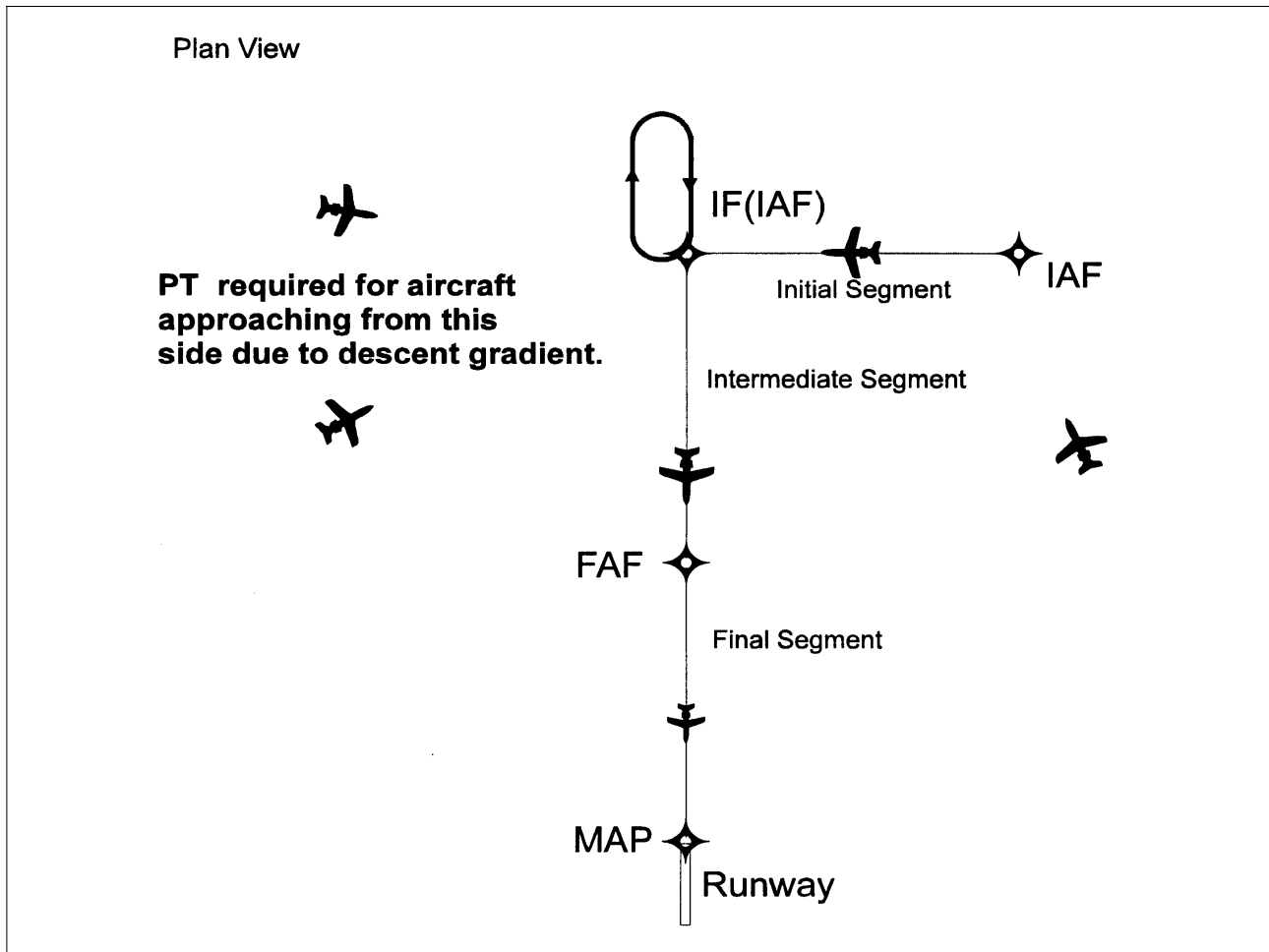
FIG ENR 1.5-17 Modified Basic "T"
