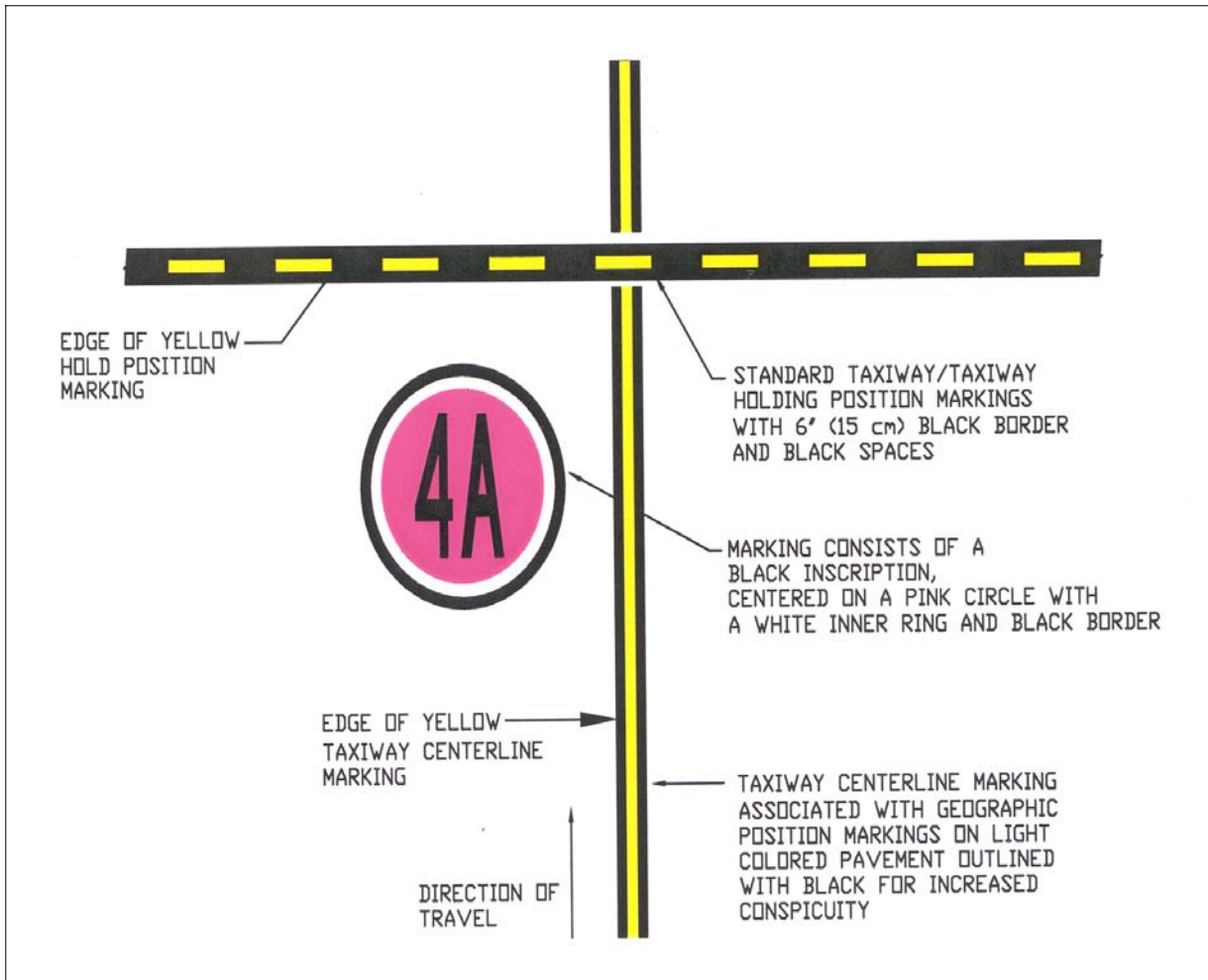
FIG AD 1.1-24 Geographic Position Markings
