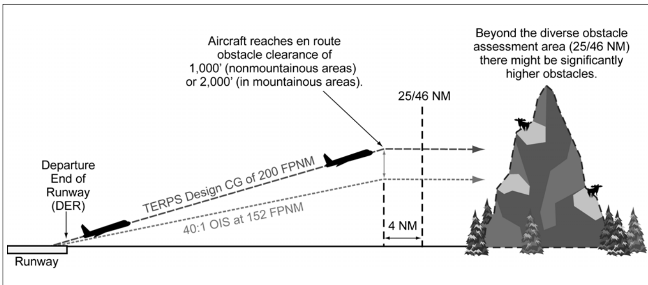
FIG ENR 1.5-37 Diverse Departure Obstacle Assessment to 25/46 NM
