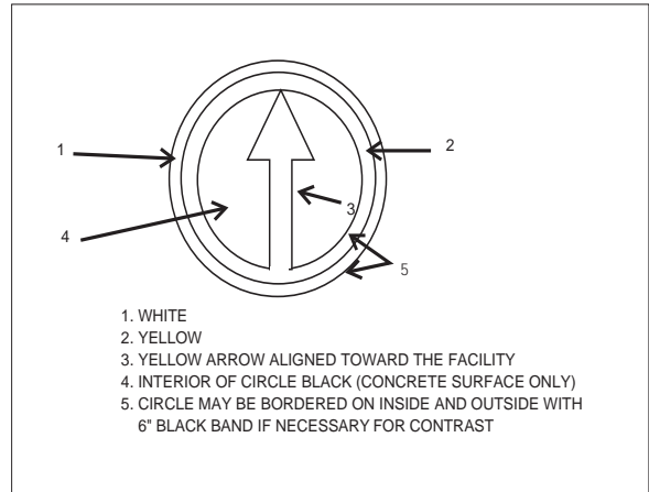
FIG AD 1.1-33 Nonmovement Area Boundary Markings
