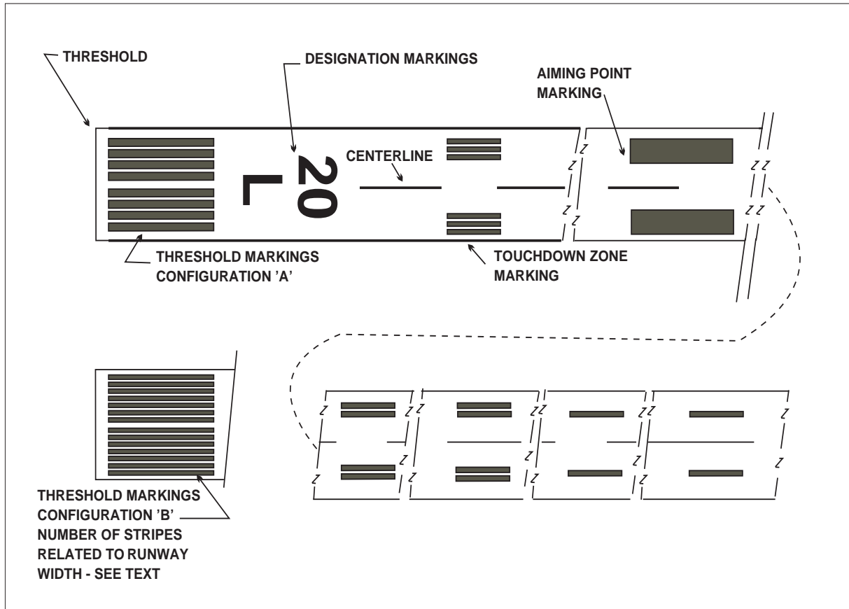
FIG AD 1.1-13 Precision Instrument Runway Markings
