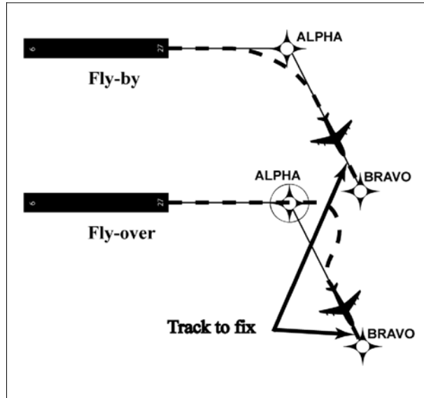
FIG ENR 1.19-2 Track to Fix Leg Type
