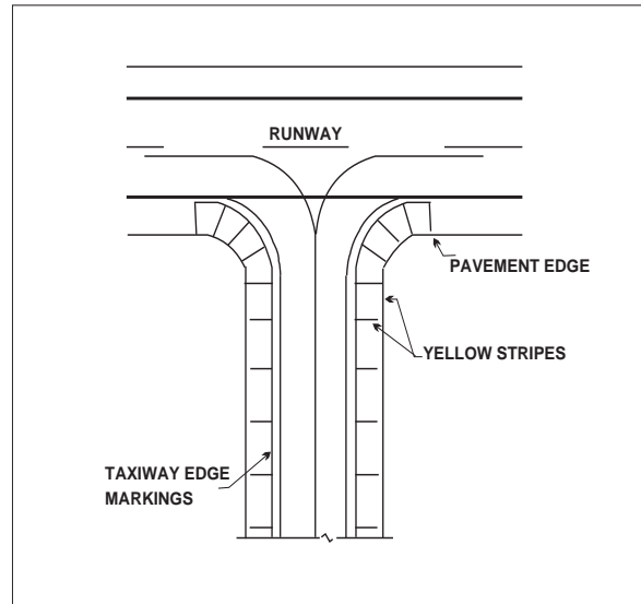
FIG AD 1.1-22 Taxi Shoulder Markings
