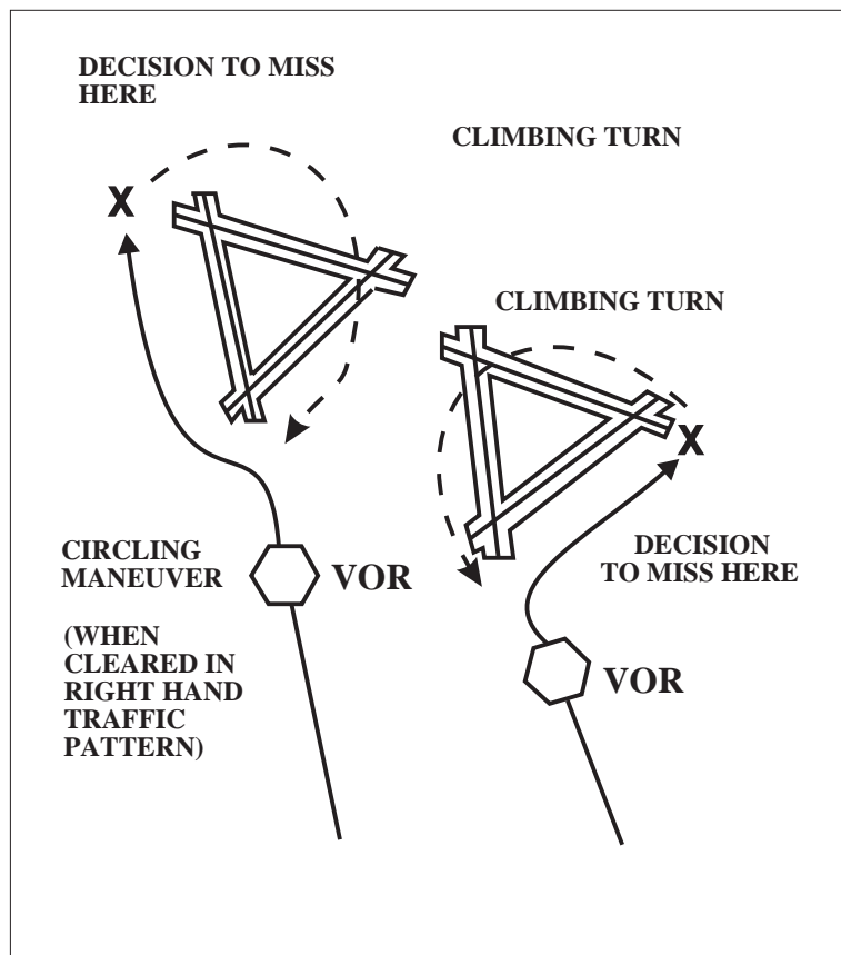
FIG ENR 1.5-34 Circling and Missed Approach Obstruction Clearance Areas
